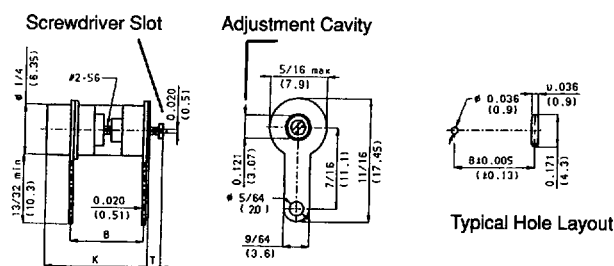
Fig. 3 Printed Circuit Lug and Lead Series.
