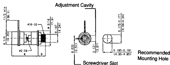
Fig. 1 Panel Mount Series
