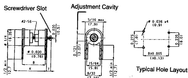
Fig. 2 Printed Circuit 4 Wire Series.
