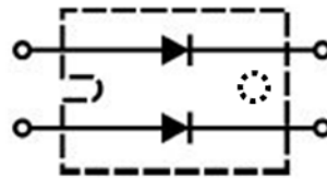
Equivalent Circuit
