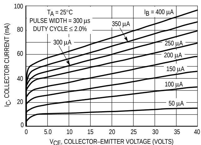
Figure 8. Collector Characteristics
