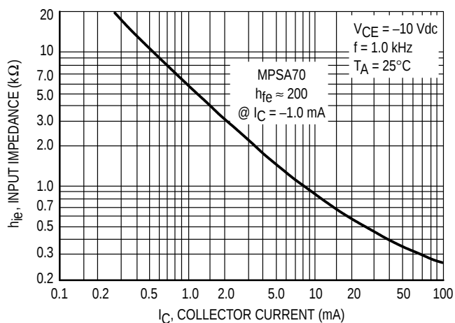
Figure 15. Input Impedance
