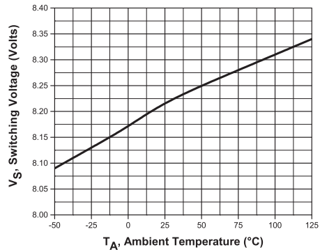
Switching Voltage
