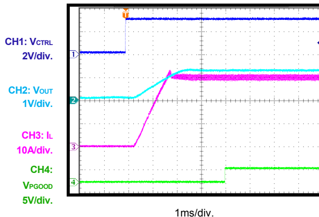
Power-On through CTRL, DCM, I_{OUT} = 30A , Single-Phase
