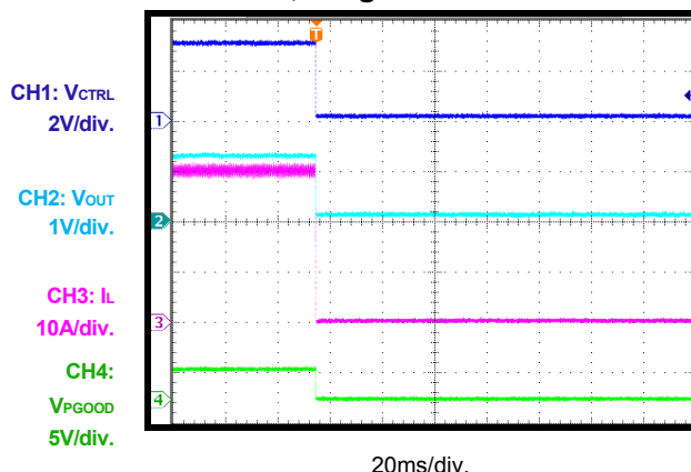
Power-Off through CTRL, CCM, I_{OUT} = 30A , Single-Phase
