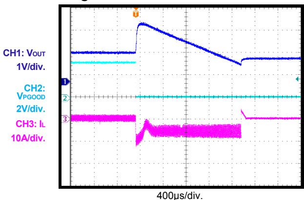
OVP, Latch-Off Option, CCM, Single-Phase
