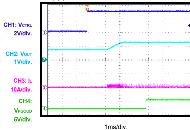
Pre-Bias Start-Up, DCM, Single-Phase
