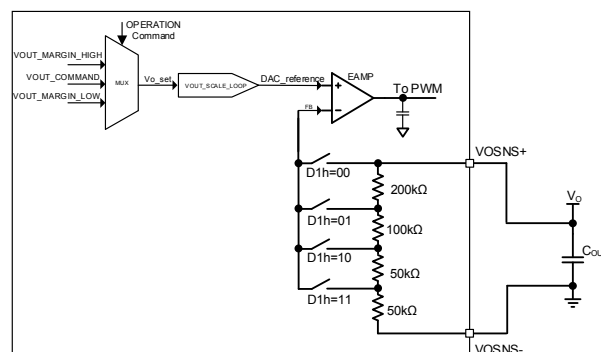
Figure 6: Output Voltage Set by Internal Resistors Divider
