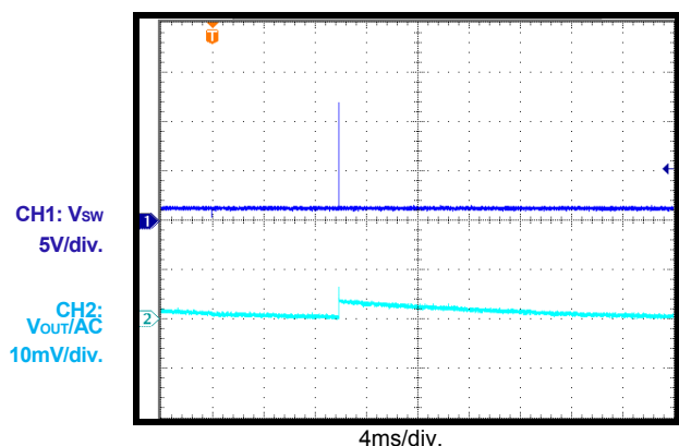
I_{OUT} = 0A , DCM, 1000kHz, Single-Phase
