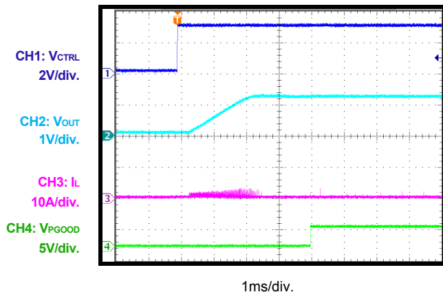
Power-On through CTRL, DCM, I_{OUT} = 0A , Single-Phase
