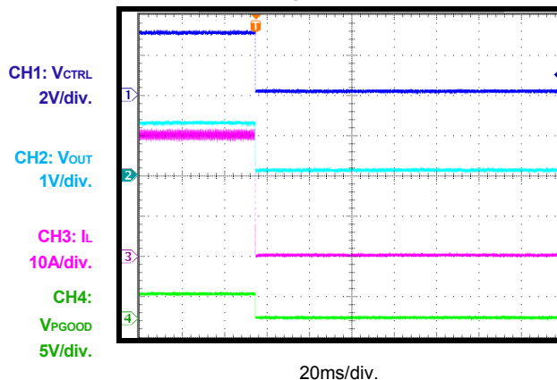
Power-Off through CTRL, DCM, I_{OUT} = 30A , Single-Phase
