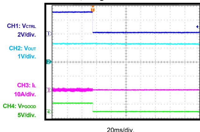
Power-Off through CTRL, CCM, I_{OUT} = 0A , Single-Phase
