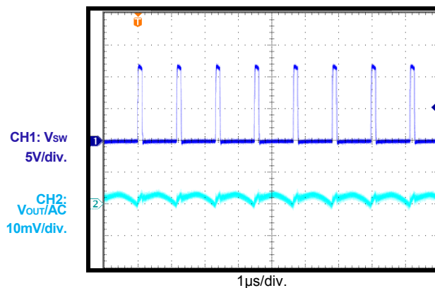
I_{OUT} = 30A , CCM, 1000kHz, Single-Phase
