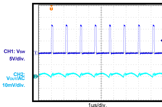
I_{OUT} = 30A , DCM, 1000kHz, Single-Phase
