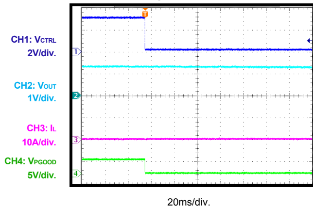
Power-Off through CTRL, DCM, I_{OUT} = 0A , Single-Phase
