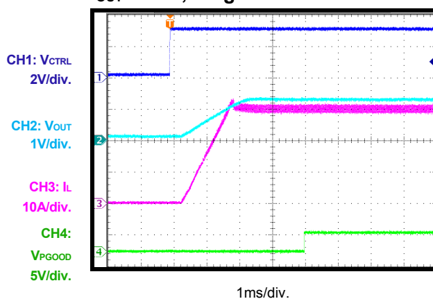
Power-On through CTRL, CCM, I_{OUT} = 30A , Single-Phase
