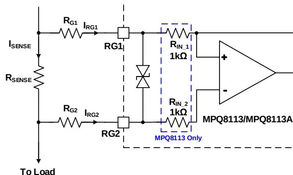
Figure 7: Back-to-Back Diodes
