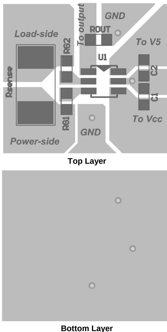
Figure 8: Recommended PCB Layout
