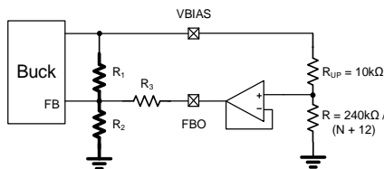
Figure 22: AFC Modulator Network with FBO Open Protection
