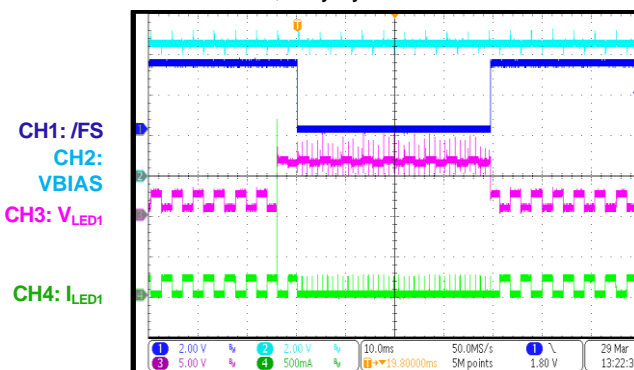
LED Short Entry/Recovery with /FS Non-Latch
