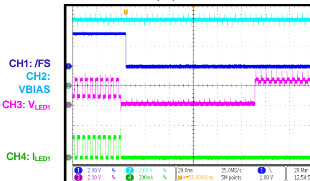
LED Open Entry/Recovery with /FS Latch
