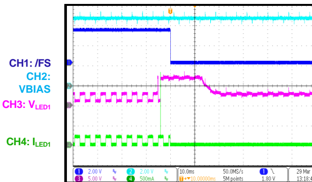
LED Short Entry/Recovery with /FS Latch
