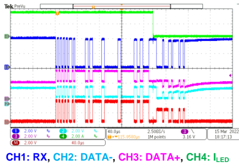
Figure 14: Differential Interface with Write CMD
