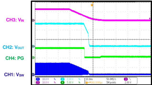
PG in Shutdown through VIN
