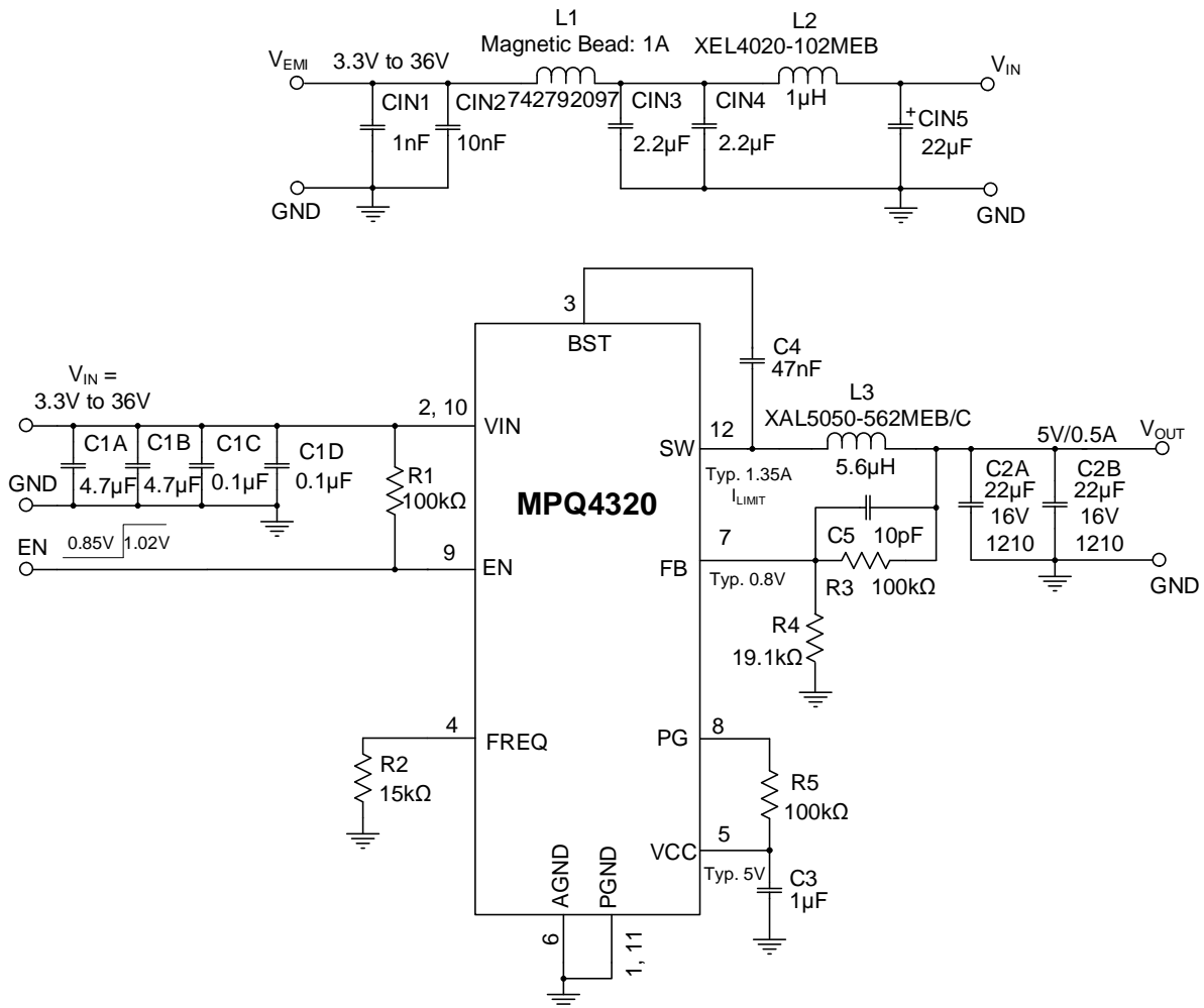
Figure 16: Typical Application Circuit ( V_{OUT} = 5V , f_{sw} = 1.8MHz with EMI Filters)
