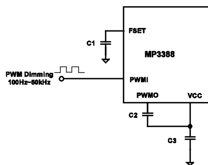
Figure 3—PWM Dimming
