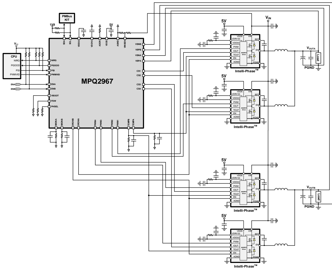
Figure 1: Typical Application Circuit for 2 + 2 Solution
