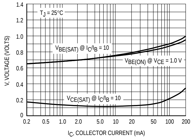
Figure 9. "ON" Voltages
