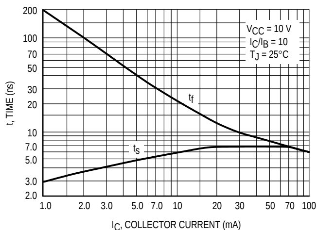
Figure 3. Turn-Off Time
