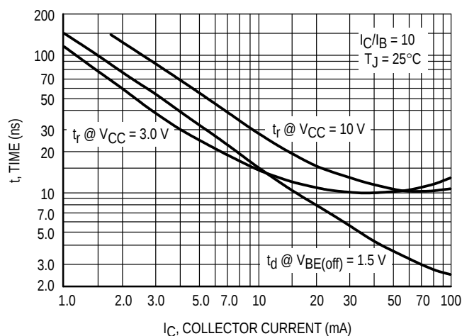
Figure 2. Turn-On Time
