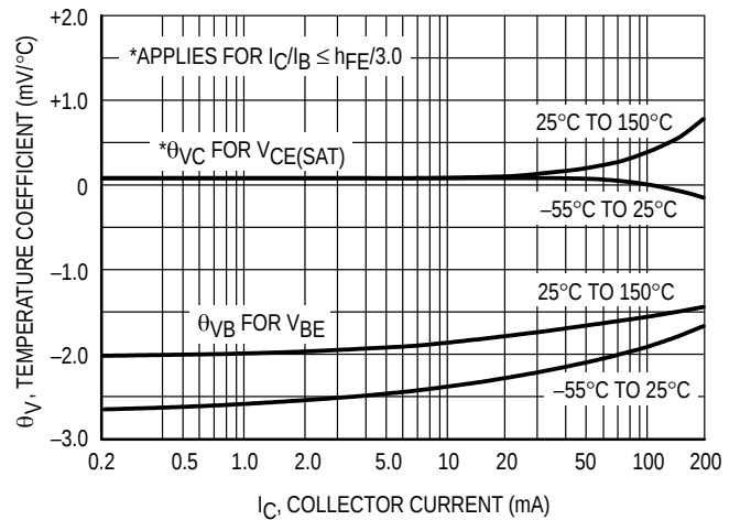
Figure 11. Temperature Coefficients
