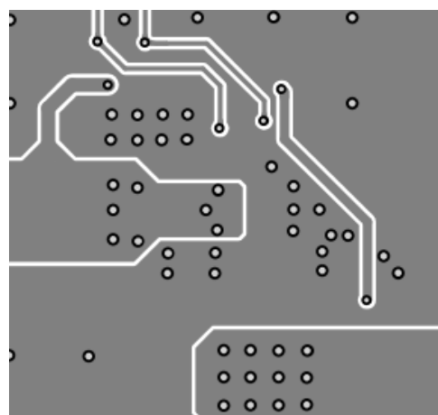
Mid-Layer 2
