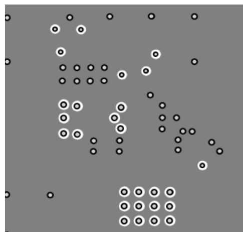
Mid-Layer 1
