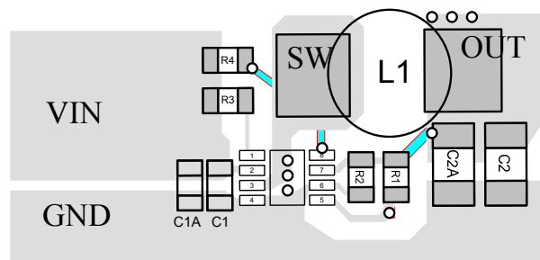
Figure 3: Layout Recommendation
