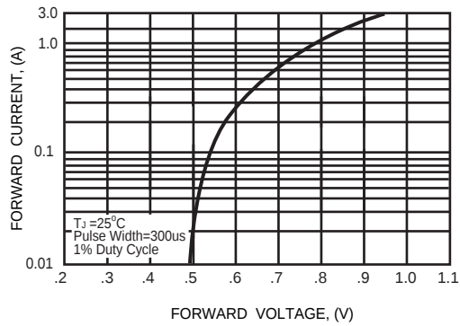
FIG. 1 - FORWARD CHARACTERISTICS
