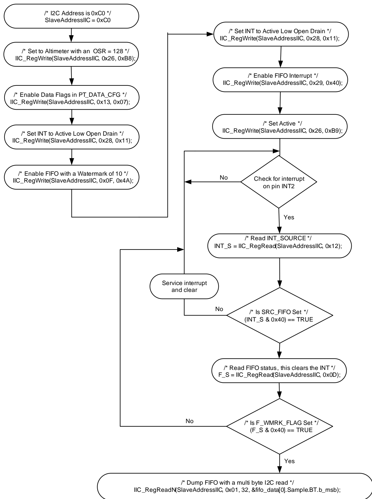
Figure 6. FIFO Setup
