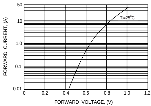
FIG. 1 - FORWARD CHARACTERISTICS
