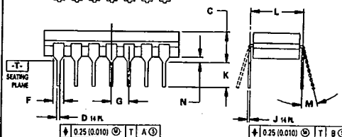
L SUFFIX CERAMIC PACKAGE CASE 632-08
