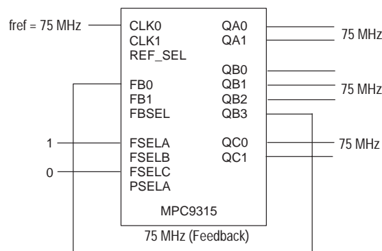
Figure 4. MPC9315 Zero Delay Buffer Configuration
