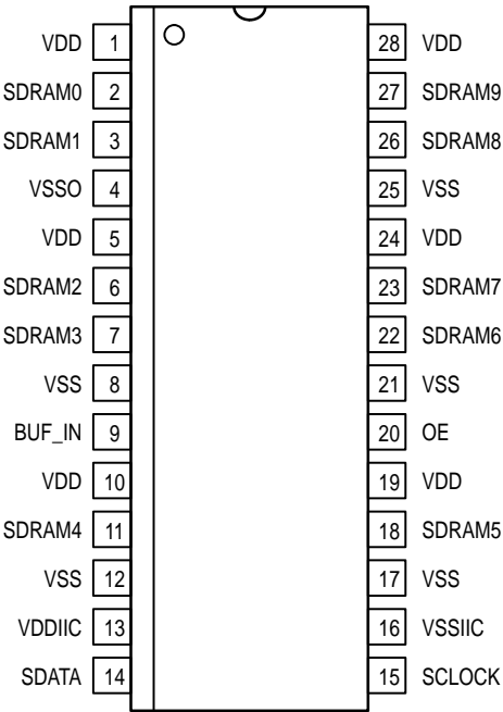
Figure 1. 28-Lead Pinout (Top View)
