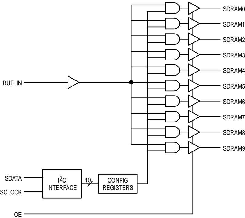
Figure 2. Block Diagram
