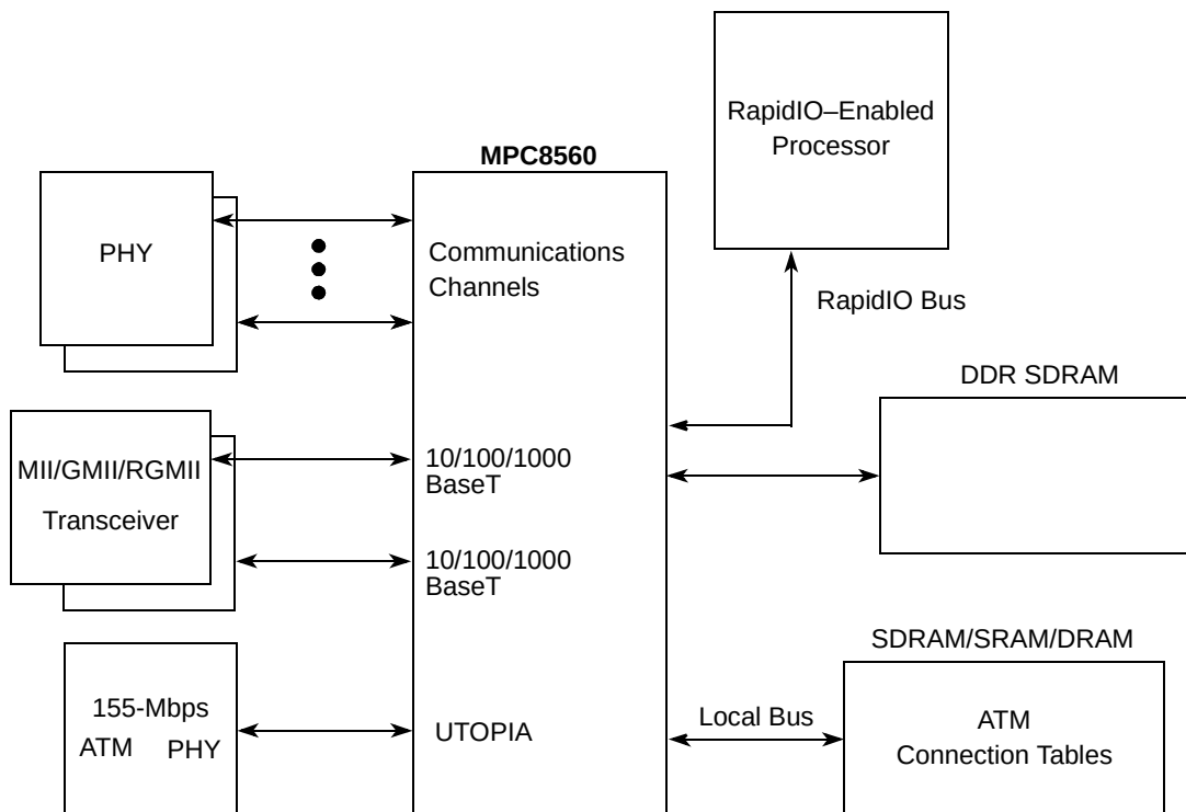
Figure 1-7. High-Performance System Microprocessor Configuration
