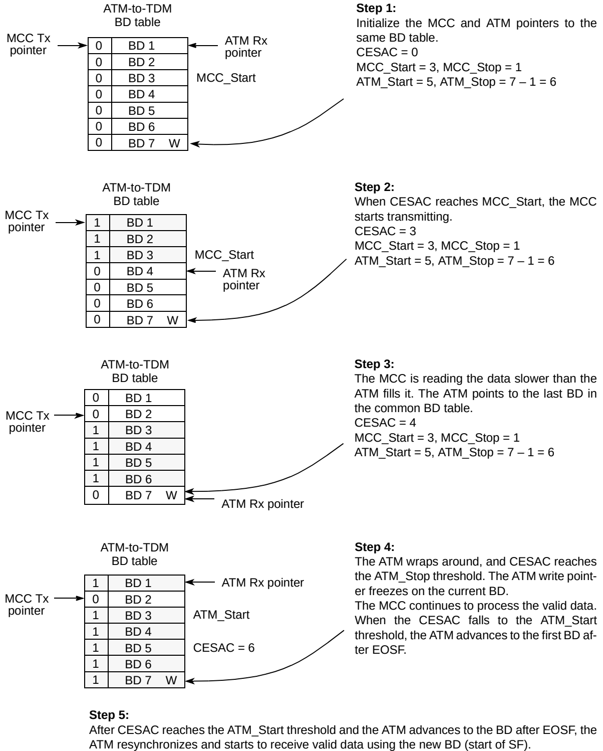
Figure 36-15. Pre-Overrun Sequence
