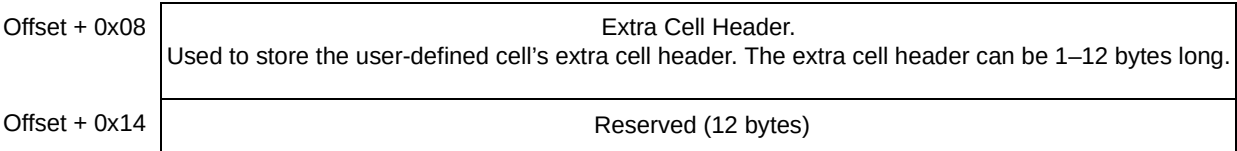
Figure 35-50. User-Defined Cell—RxBD Extension
