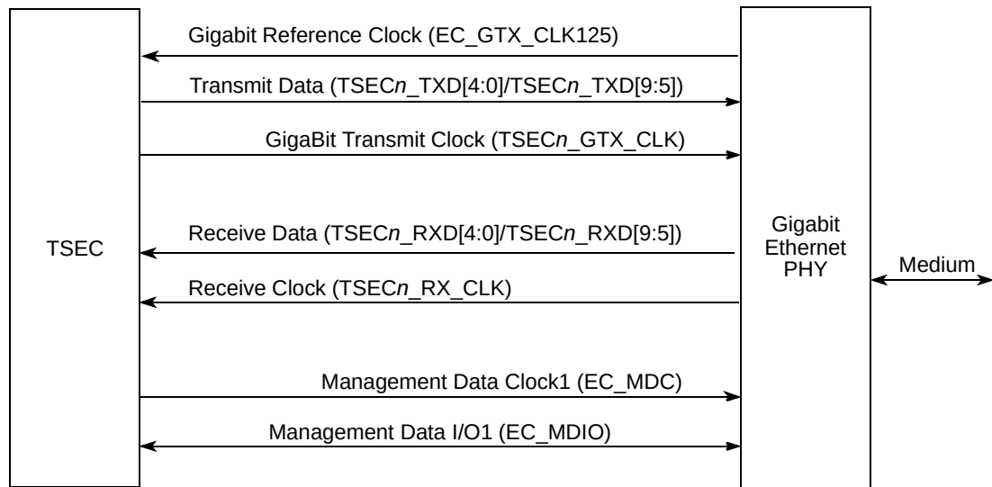
Figure 13-114. TSEC-RTBI Connection
