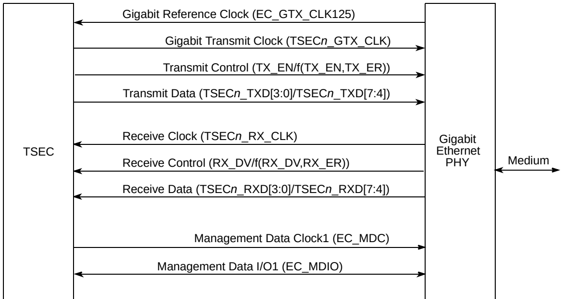
Figure 13-112. TSEC-RGMII Connection
