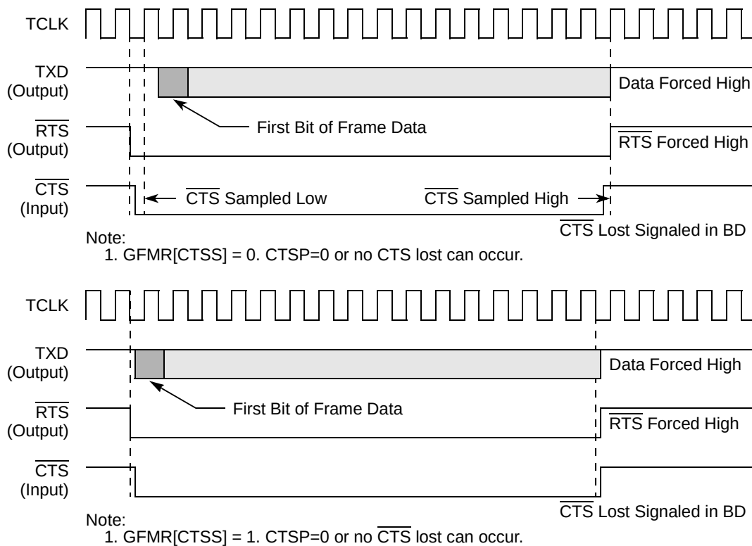
Figure 34-10. CTS Lost
