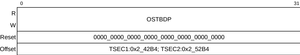
Figure 13-26. OSTBDP Register Definition
