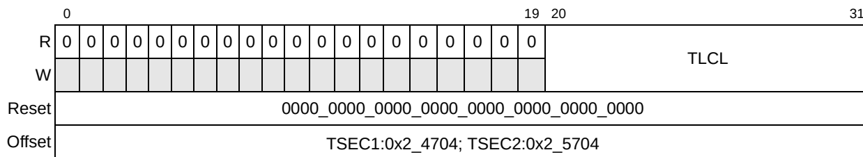
Figure 13-82. Transmit Late Collision Packet Counter Register Definition
