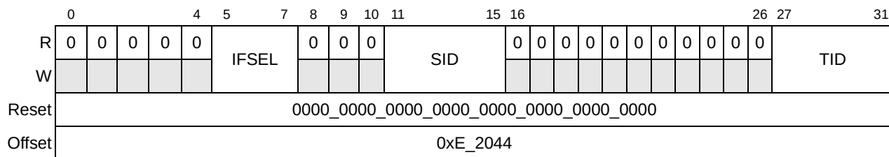
Figure 19-9. Trace Buffer Control Register 1 (TBCR1)
