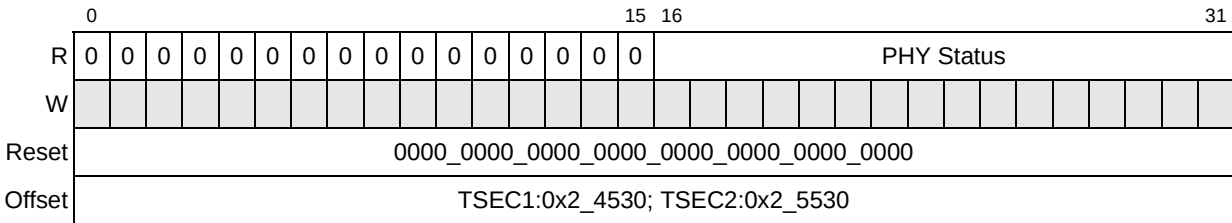
Figure 13-44. MIIMSTAT Register Definition
