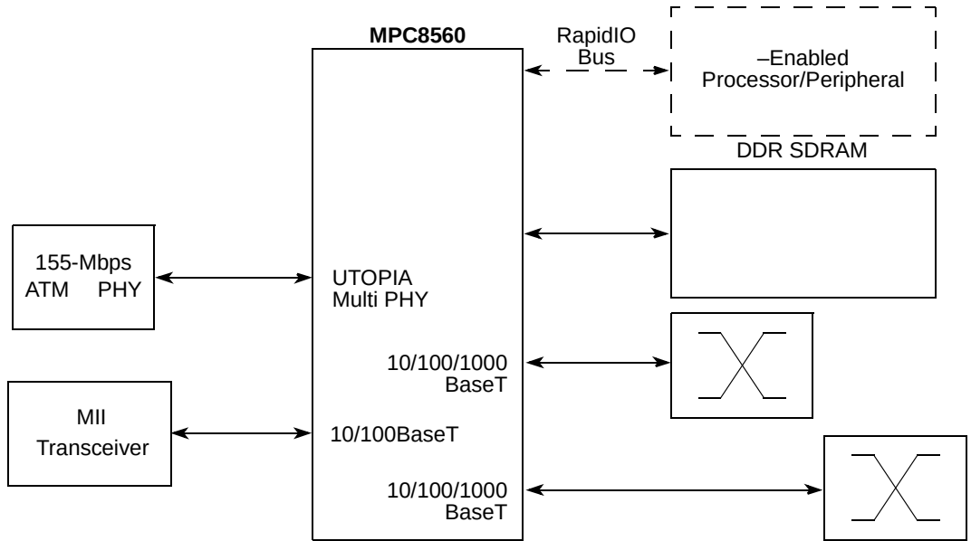
Figure 1-16. ATM Protocol Converter Configuration
