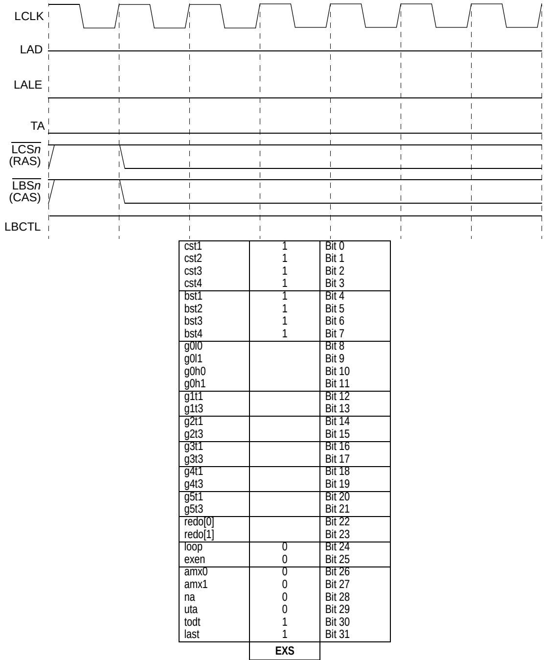
Figure 12-67. Exception Cycle
