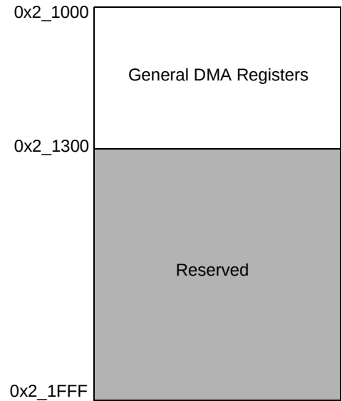
Figure 14-4. DMA Register Space (Memory-Mapped)
