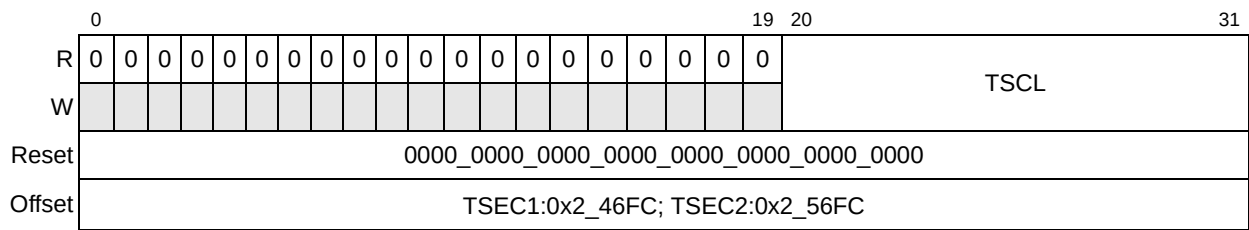
Figure 13-80. Transmit Single Collision Packet Counter Register Definition
