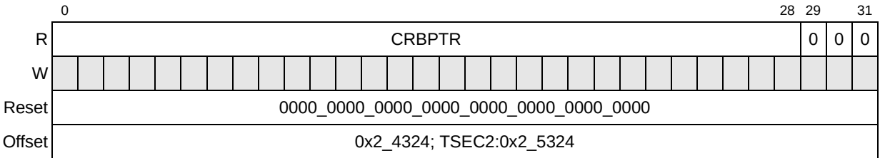
Figure 13-31. CRBPTR Register Definition
