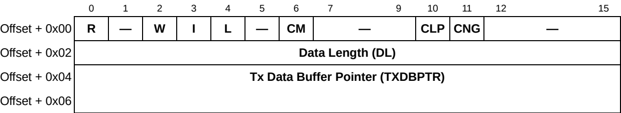
Figure 35-51. AAL5 TxBD
