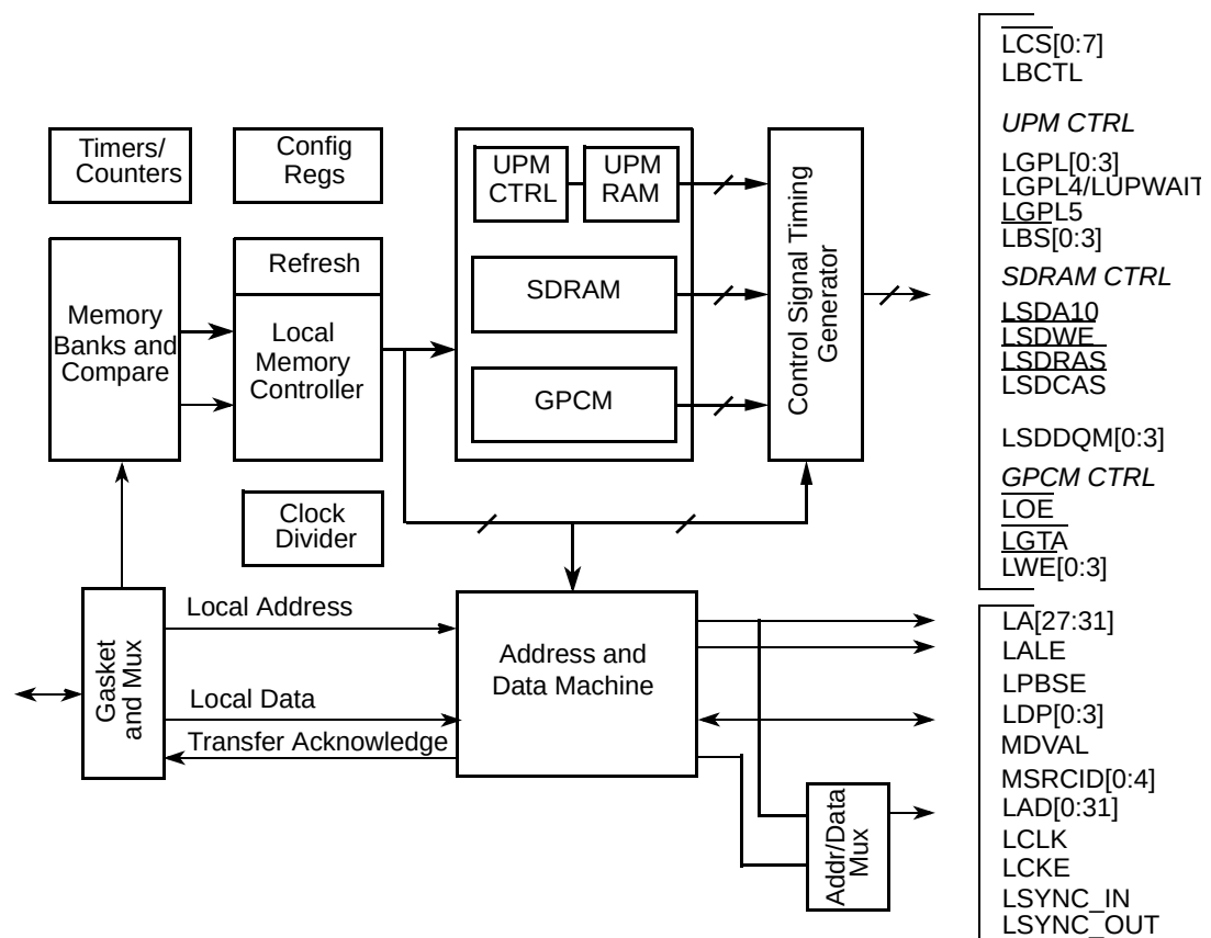
Figure 12-1. Local Bus Controller Block Diagram
