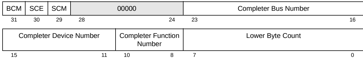
Figure 15-77. AD[31:0] During PCI-X Split Completion Attribute Phase
