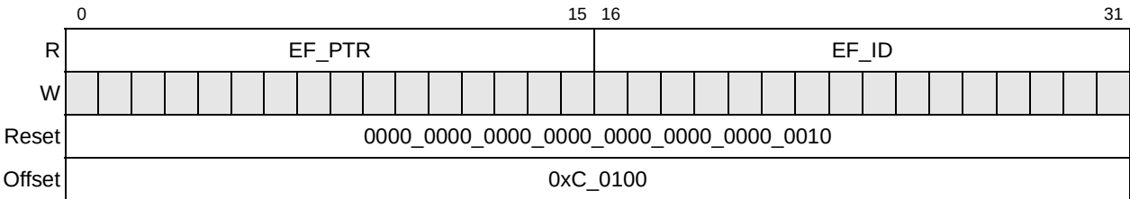
Figure 16-18. 8/16 LP-LVDS Port Maintenance Block Header 0 Command and Status Register (PMBH0CSR)
