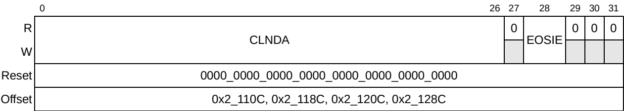
Figure 14-8. Current Link Descriptor Address Registers (CLNDAR n )
