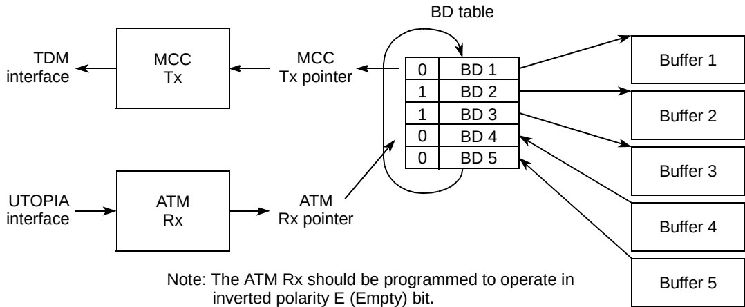
Figure 36-5. ATM-to-TDM Interworking
