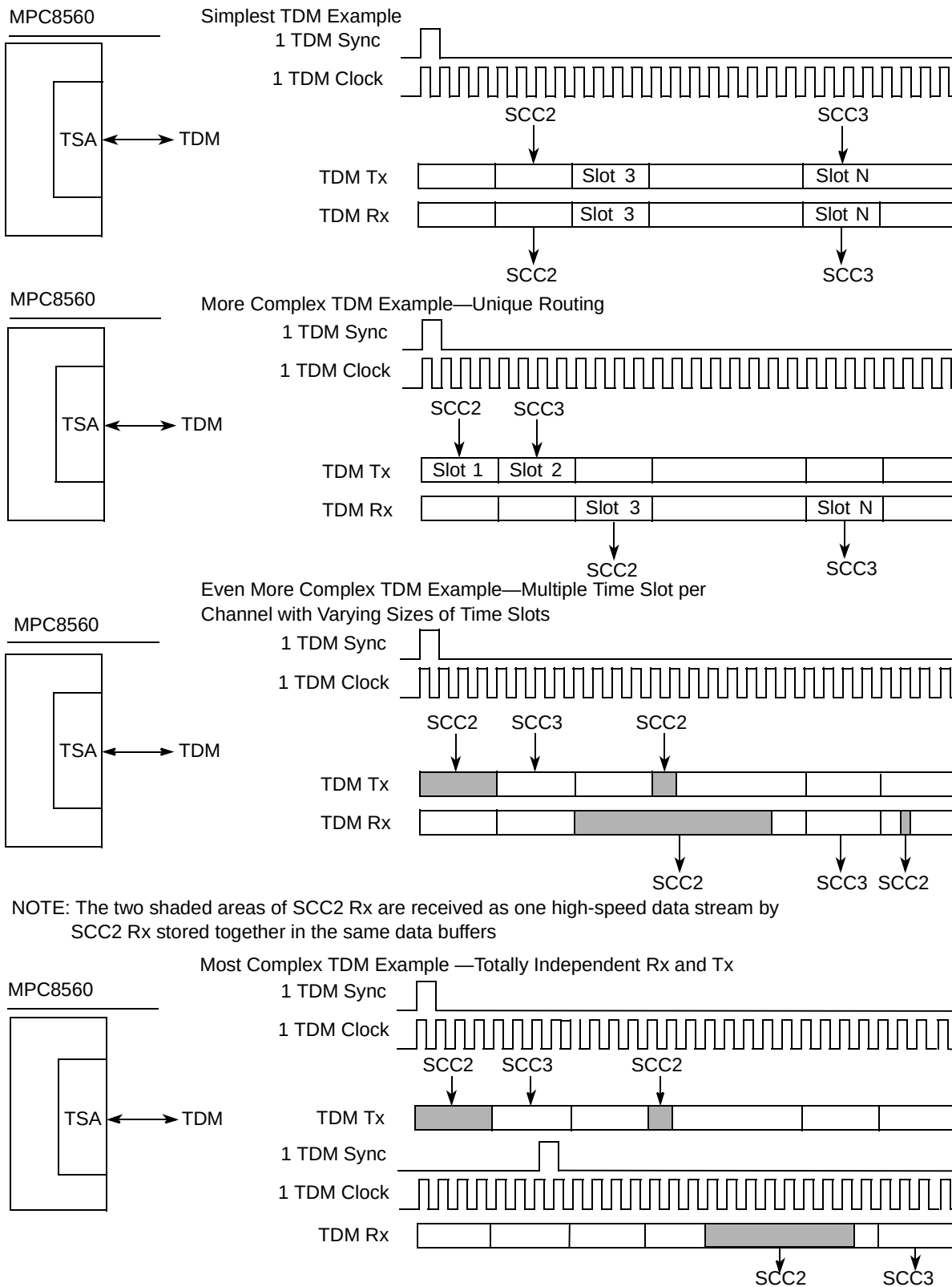
Figure 22-2. Various Configurations of a Single TDM Channel
