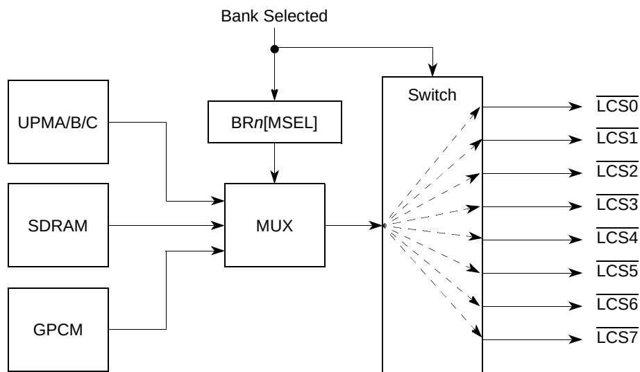
Figure 12-59. \overline{\text{LCS}}_n Signal Selection
