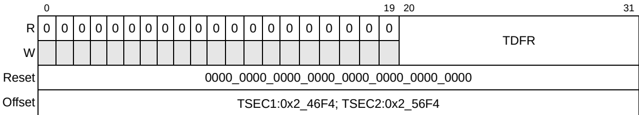
Figure 13-78. Transmit Deferral Packet Counter Register Definition
