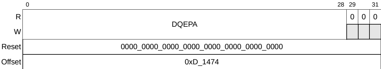
Figure 16-77. Doorbell Queue Enqueue Pointer Address Register (DQEPAR)
