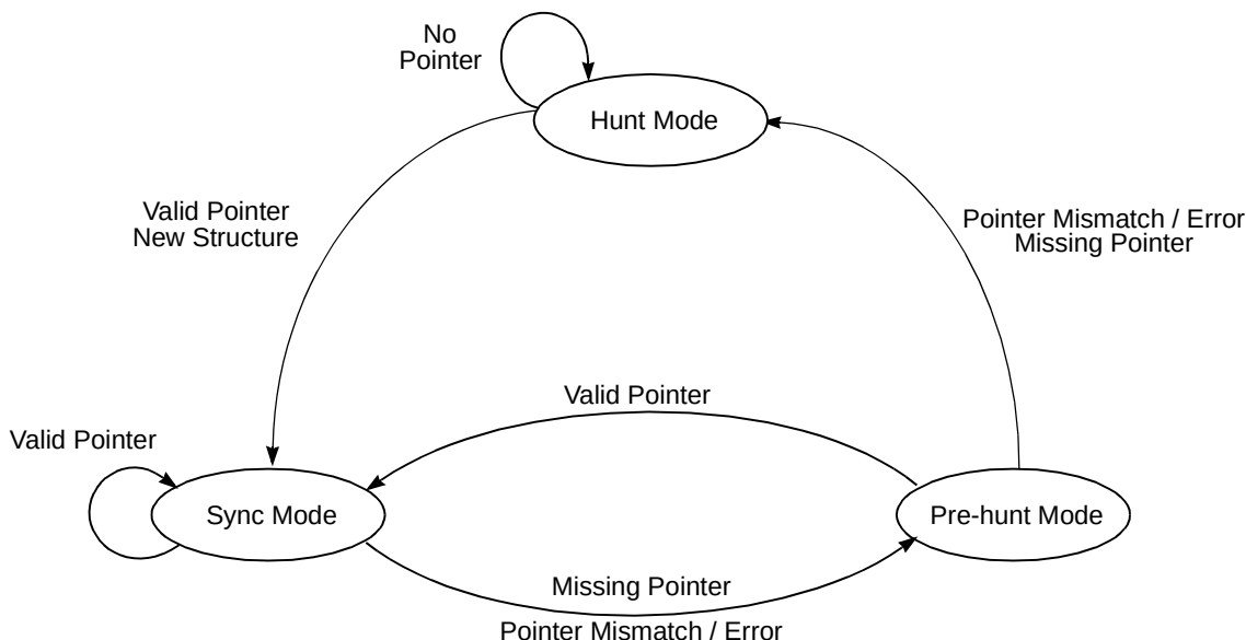
Figure 36-20. Pointer Verification Mechanism
