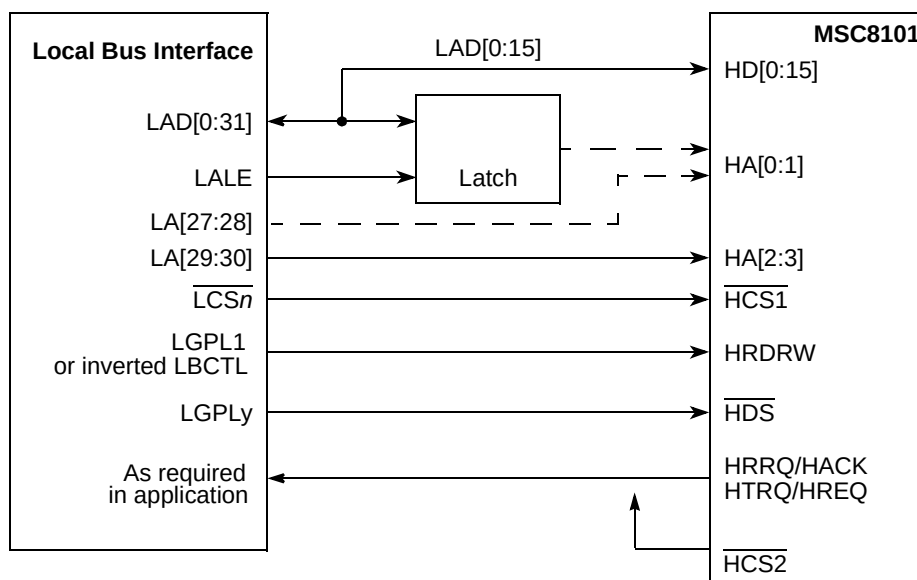
Figure 12-81. Interface to MSC8101 HDI16
