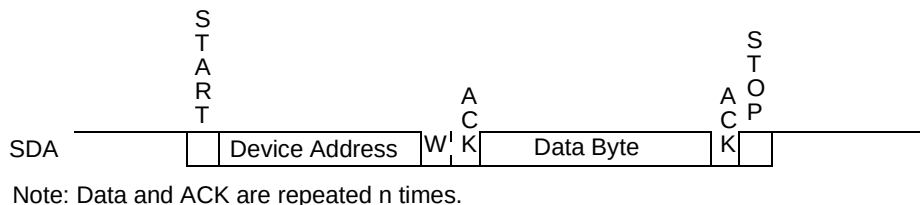
Figure 44-4. I 2 C Master Write Timing
