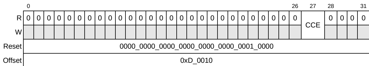
Figure 16-28. Port Configuration Register (PCR)
