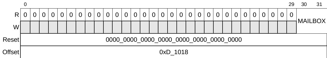
Figure 16-66. Outbound Destination Port Registers (ODPR)
