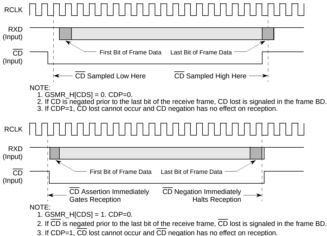
Figure 27-12. Using \overline{\text{CD}} to Control Synchronous Protocol Reception
