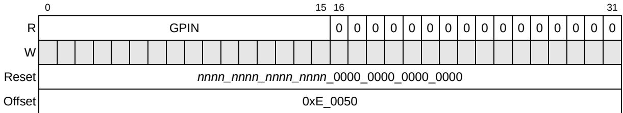
Figure 17-9. General-Purpose Output Data Register (GPINDR)
