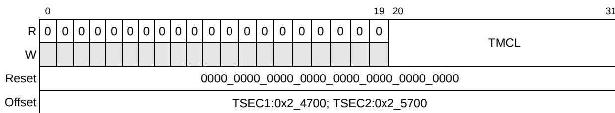
Figure 13-81. Transmit Multiple Collision Packet Counter Register Definition
