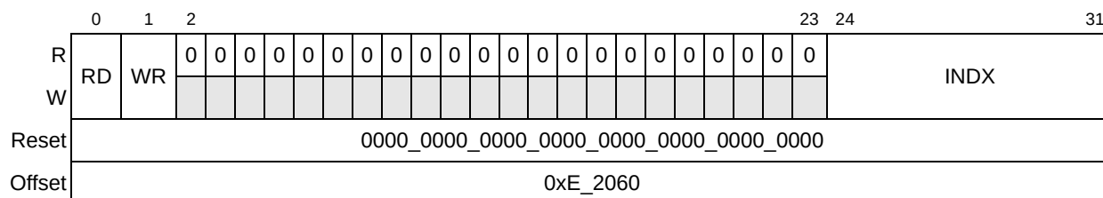
Figure 19-14. Trace Buffer Access Control Register (TBACR)
