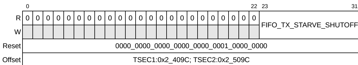
Figure 13-17. FIFO TX STARVE SHUTOFF Register Definition
