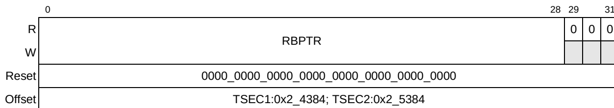
Figure 13-33. RBPTR Register Definition
