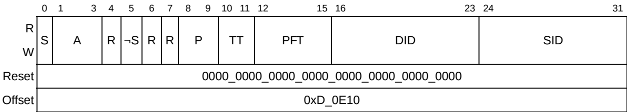
Figure 16-43. Error Packet Capture Register 0 (EPCR0)
