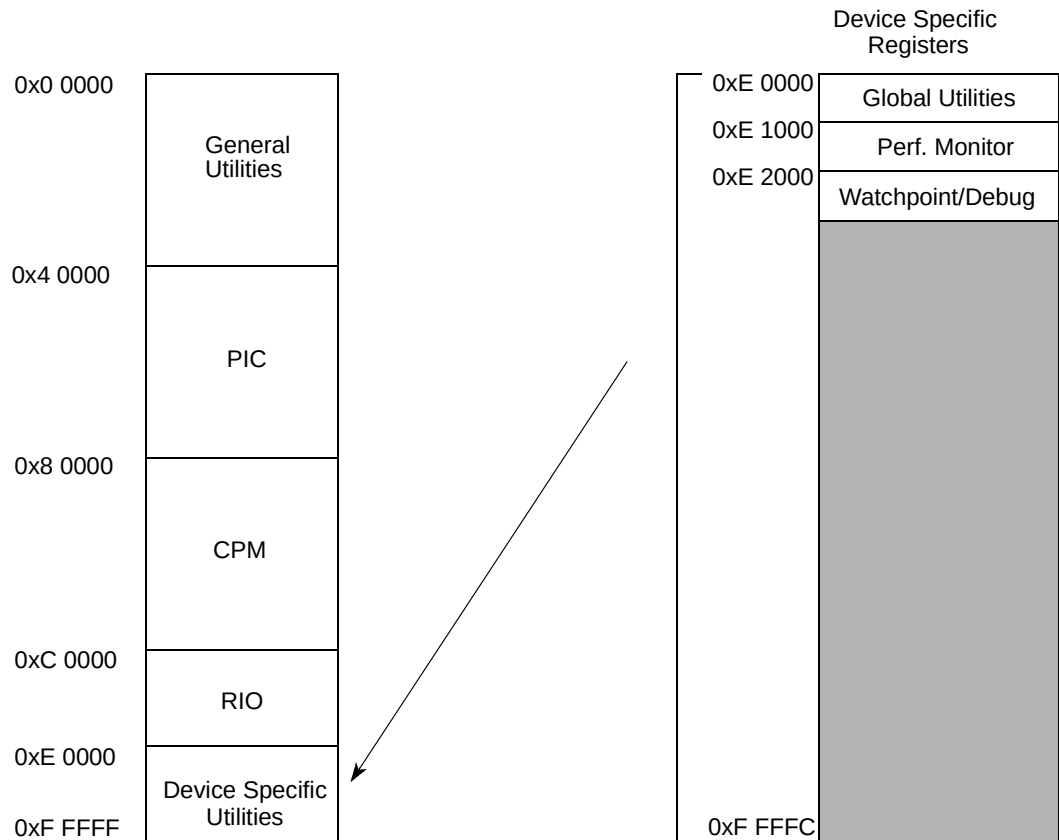
Figure 2-9. Device-Specific Register Mapping to Configuration, Control, and Status Memory Block
