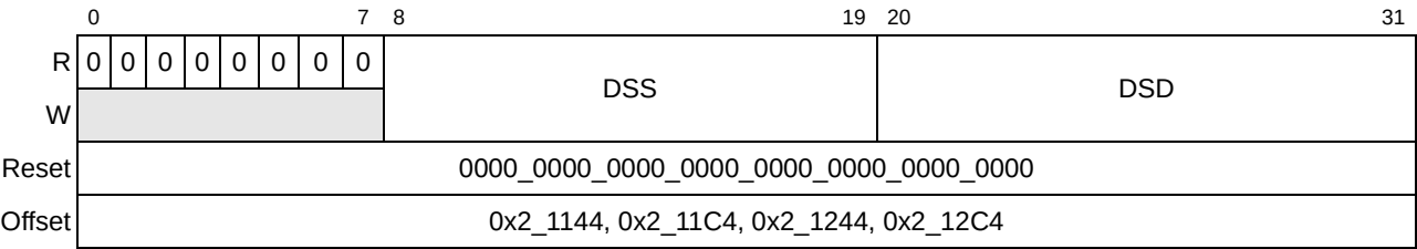
Figure 14-20. Destination Stride Registers (DSR n )
