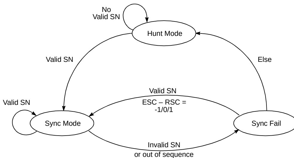
Figure 36-19. 3-Step-SN Algorithm
