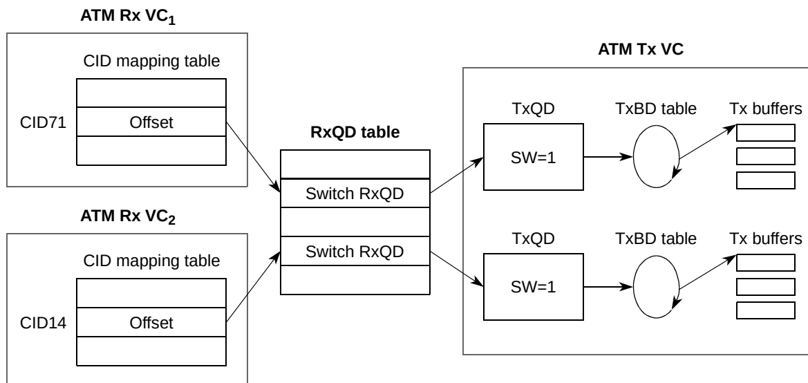
Figure 37-14. AAL2 Switching
