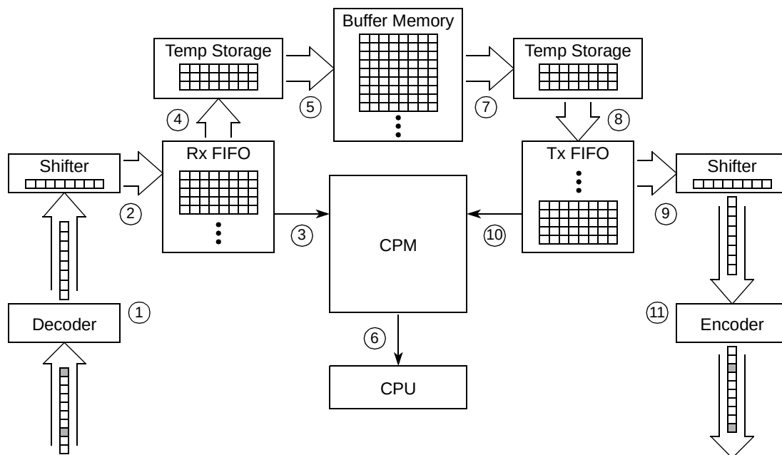
Figure 1-3. Data Processing in the CPM
