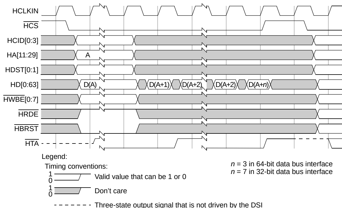
Figure 12-89. Synchronous Burst Write to MSC8102 DSI
