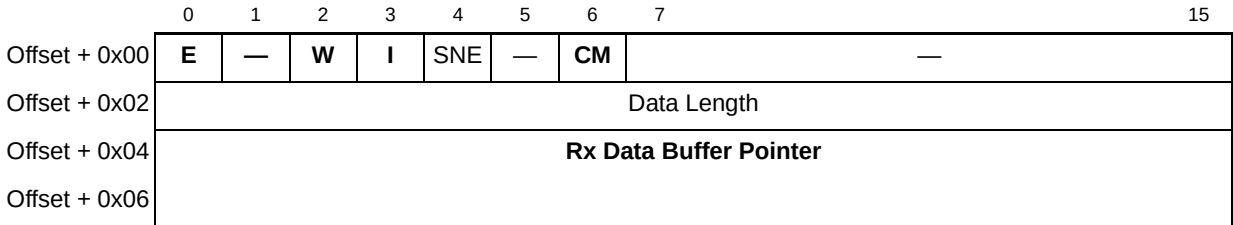
Figure 35-48. AAL1 RxBD
