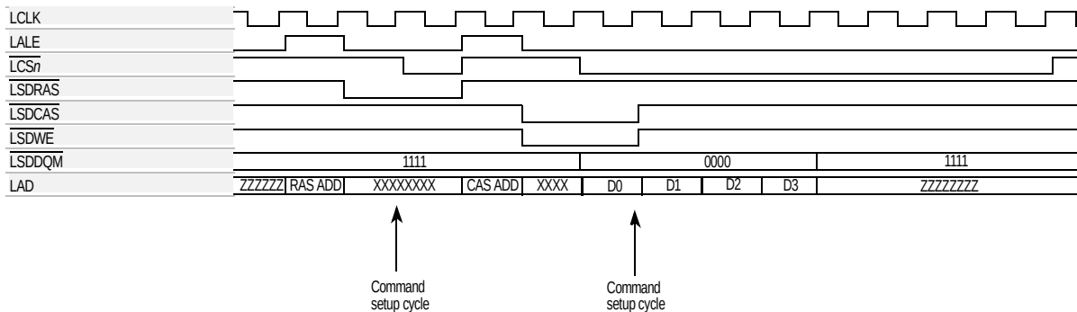
Figure 12-40. BUFCMD = 1, LCRR[BUFCMDC] = 2
