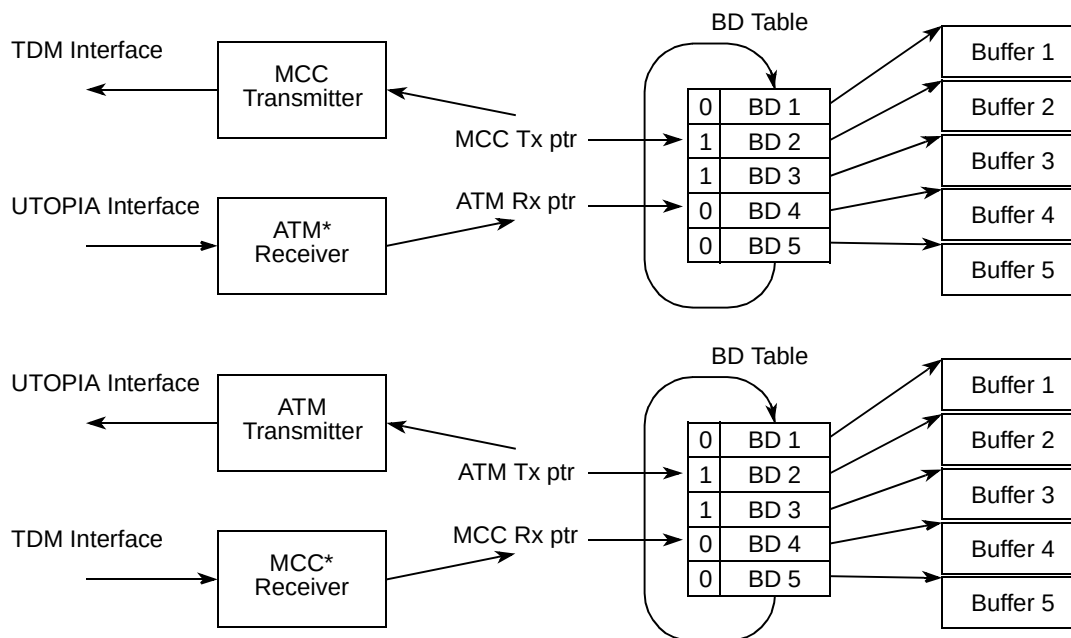
Figure 35-21. ATM-to-TDM Interworking
