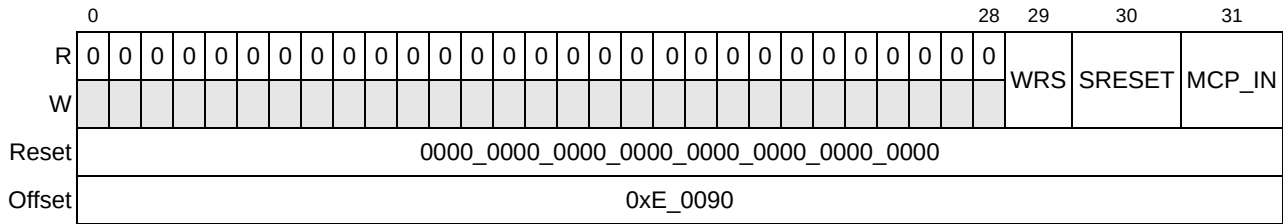
Figure 17-13. Machine Check Summary Register (MCPSUMR)
