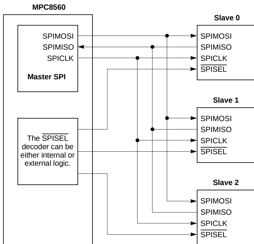
Figure 43-2. Single-Master/Multi-Slave Configuration
