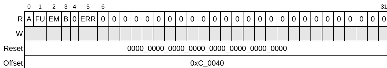
Figure 16-11. Mailbox Status Register (MSR)
