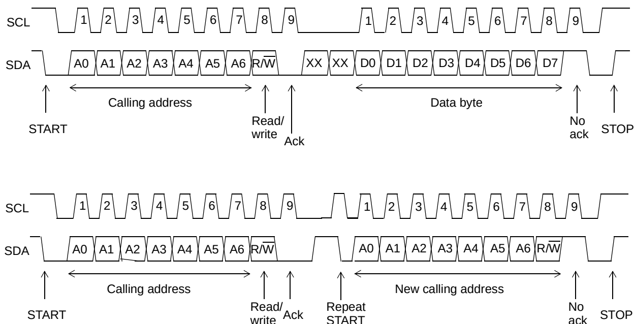
Figure 11-8. I²C Interface Transaction Protocol
