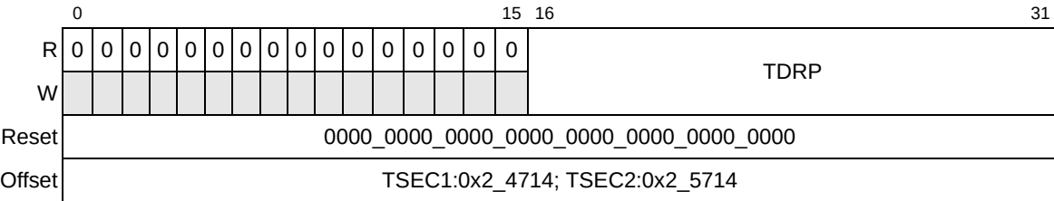
Figure 13-85. Transmit Drop Frame Counter Register Definition
