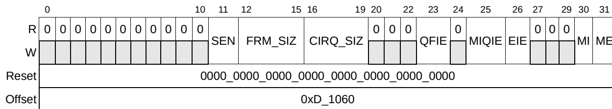
Figure 16-70. Inbound Mode Register (IMR)
