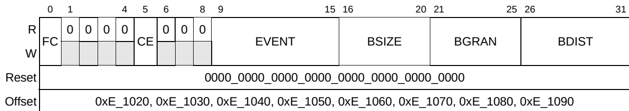
Figure 18-4. Performance Monitor Local Control Registers A1–A8 (PMLCA1–PMLCA8)
