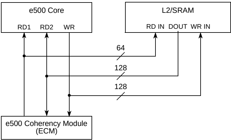
Figure 7-5. Data Bus Connection of CCB
