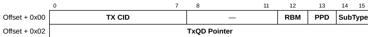
Figure 37-18. CPS Switch Rx Queue Descriptor
