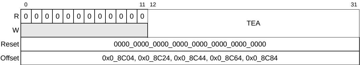
Figure 15-7. PCI/X Outbound Translation Extended Address Registers
