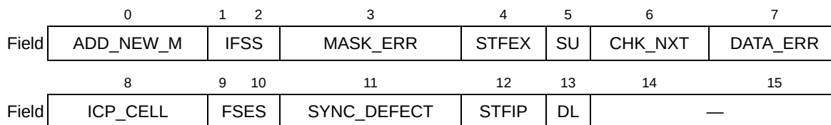
Figure 39-25. IMA Link Receive State (ILRSTATE)
