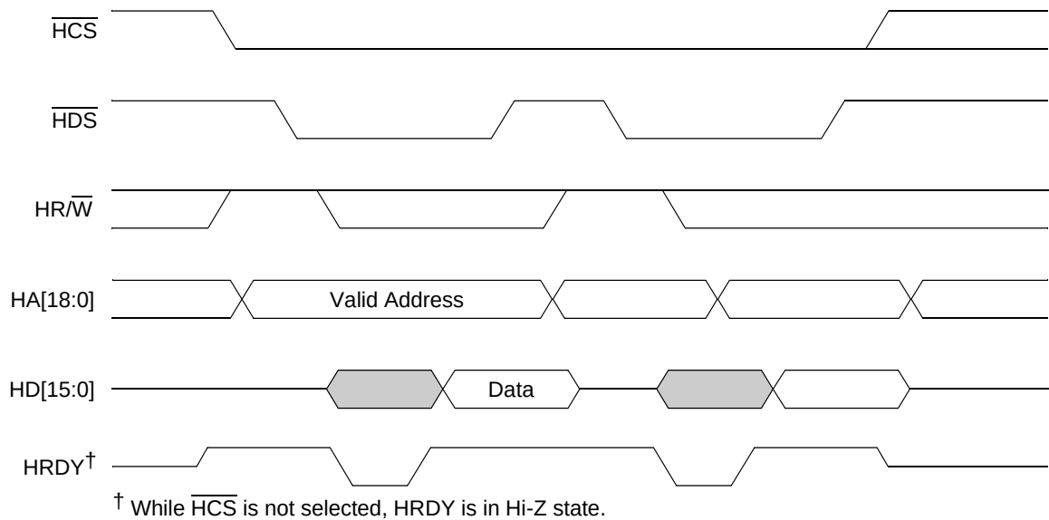
Figure 12-92. EHPI Non-Multiplexed Read Timings
