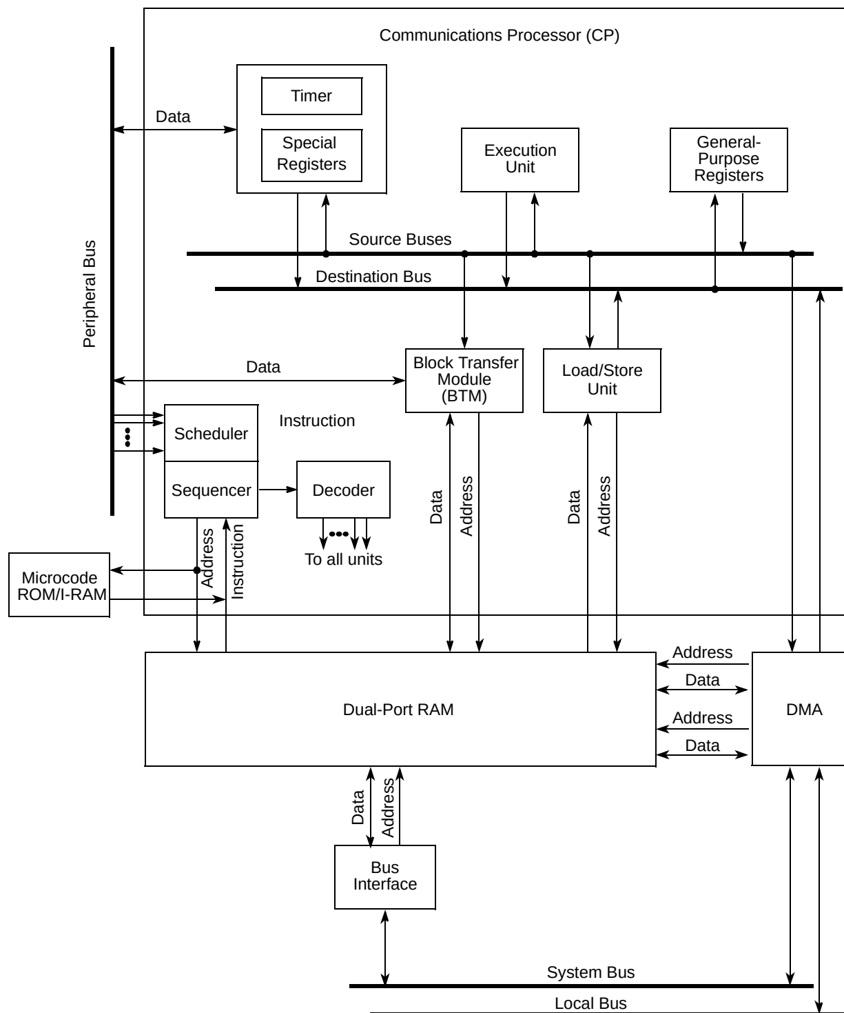
Figure 20-2. Communications Processor (CP) Block Diagram
