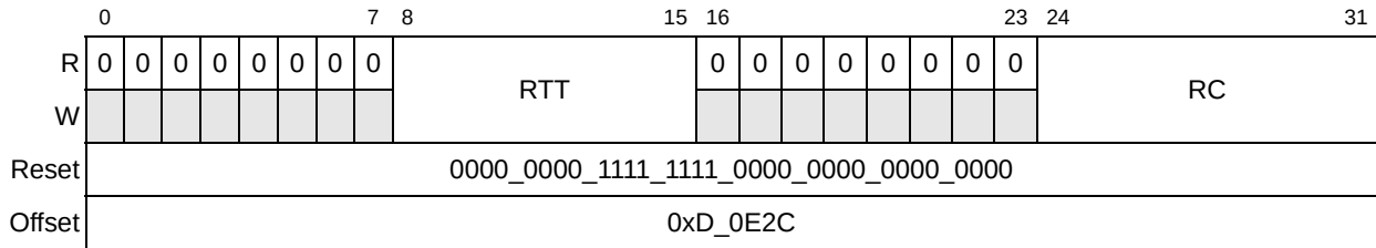
Figure 16-61. Port Retry Threshold Register (PRTR)
