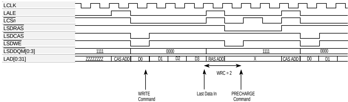
Figure 12-38. WRC = 2 (2 Clock Cycles)
