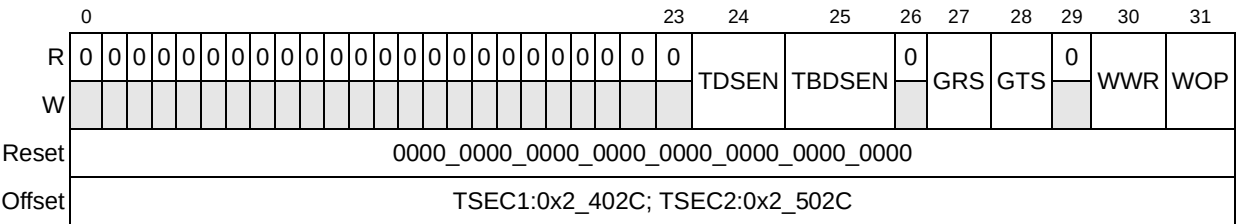
Figure 13-12. DMACTRL Register Definition
