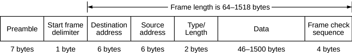
Figure 13-3. Ethernet/IEEE 802.3 Frame Structure
