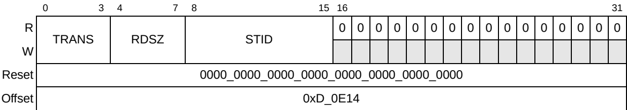
Figure 16-45. Error Packet Capture Register 1 (EPCR1)—Type 2 Packet Format
