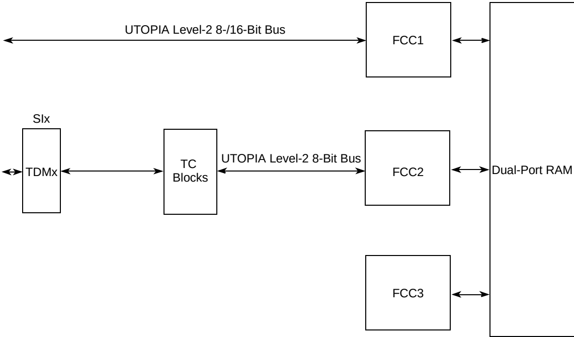
Figure 38-1. Serial ATM Using FCC2 and TC Blocks (Single Channel)
