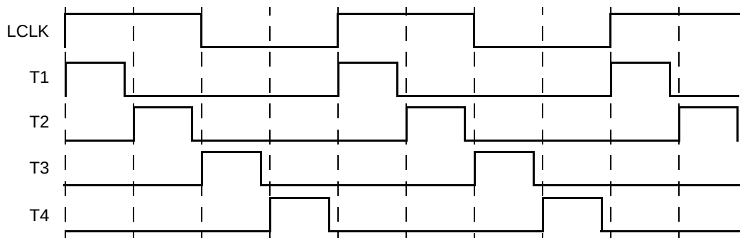
Figure 12-56. UPM Clock Scheme for \text{LCRR}[\text{CLKDIV}] = 4 or 8
