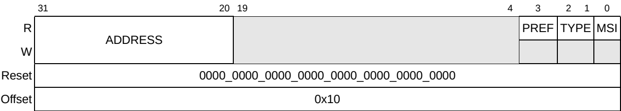
Figure 15-37. PCI Configuration and Status Register Base Address Register (PCSRBAR)
