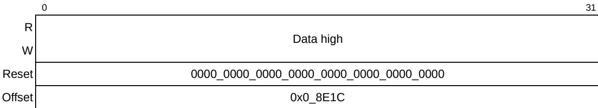
Figure 15-22. PCI/X Error Data High Capture Register (ERR_DH)
