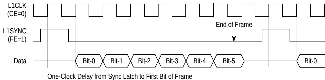
Figure 22-13. One-Clock Delay from Sync to Data (xFSD = 01)
