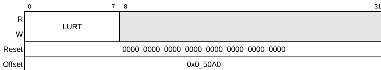
Figure 12-11. UPM Refresh Timer (LURT)
