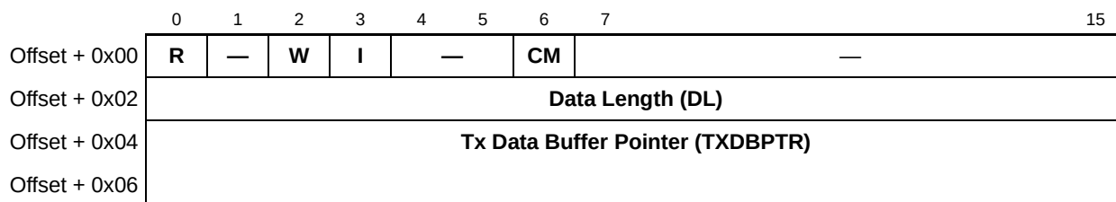
Figure 35-52. AAL1 TxBD
