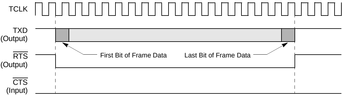
Figure 27-9. Output Delay from \overline{\text{RTS}} Asserted for Synchronous Protocols
