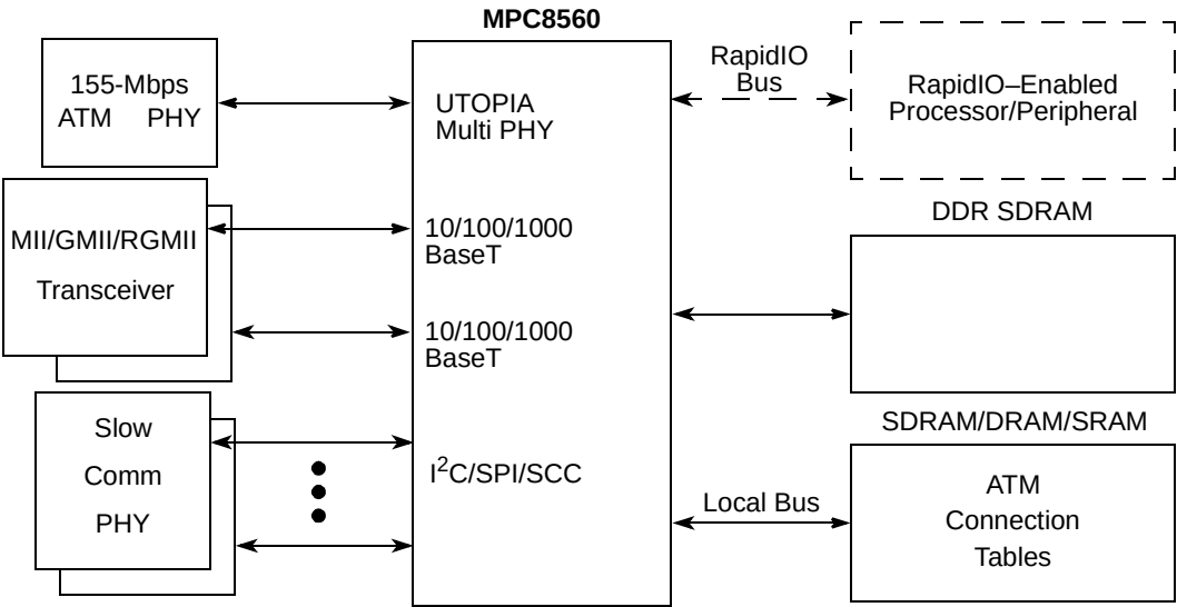
Figure 1-13. Telecommunications Switch Controller Configuration
