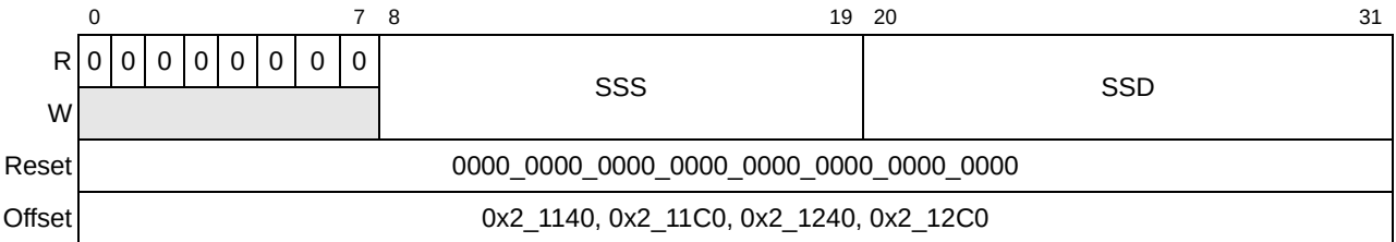
Figure 14-19. Source Stride Registers (SSR n )
