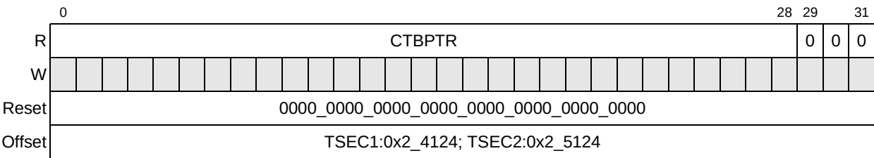
Figure 13-22. CTBPTR Register Definition
