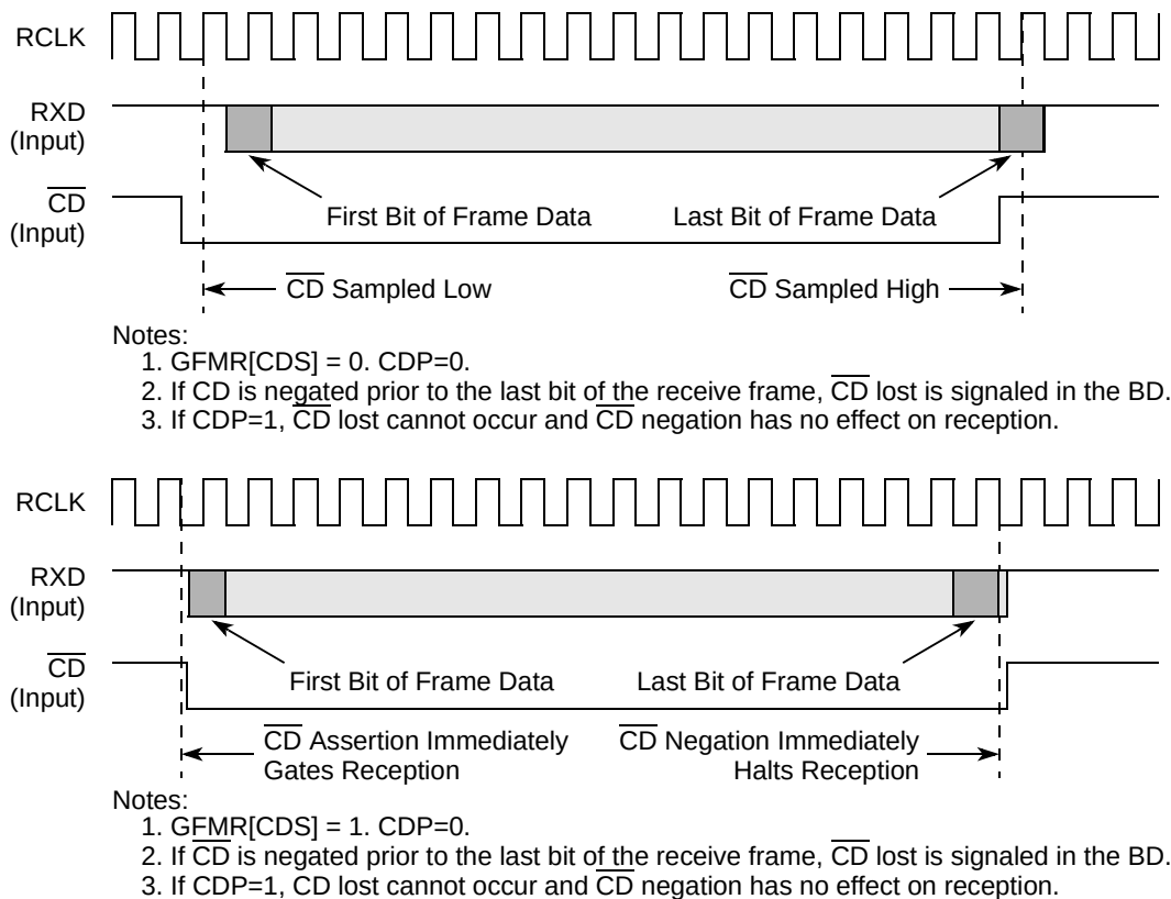
Figure 34-11. Using \overline{CD} to Control Reception
