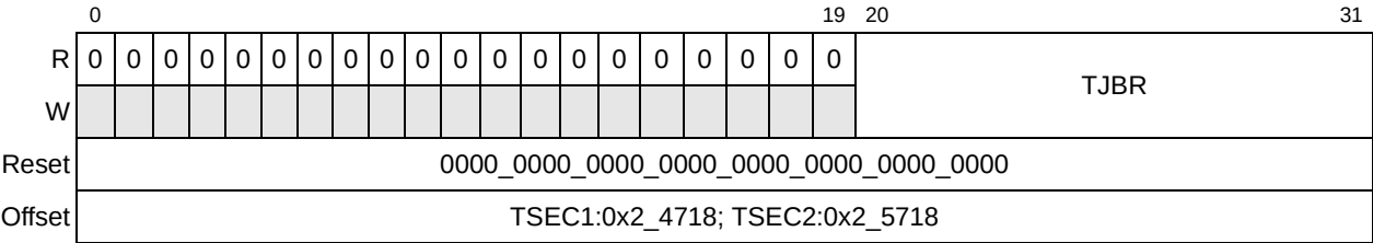
Figure 13-86. Transmit Jabber Frame Counter Register Definition
