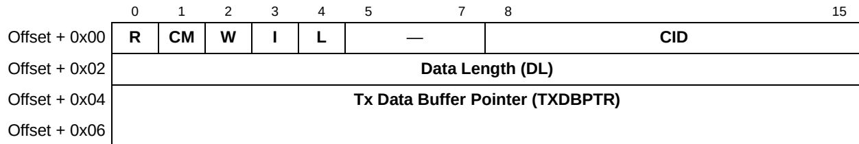
Figure 37-12. SSSAR TxBD
