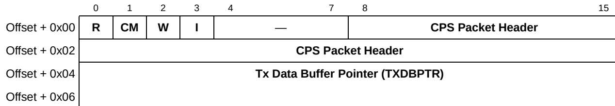
Figure 37-9. CPS TxBD
