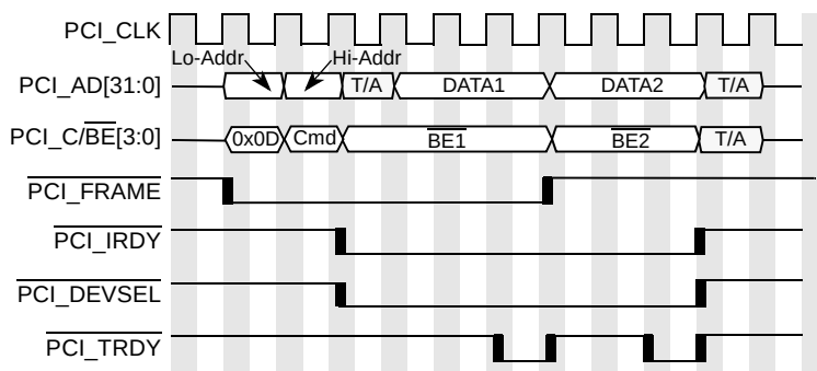
Figure 15-61. DAC Burst Read Example
