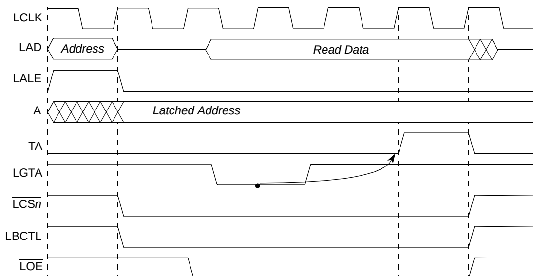
Figure 12-32. External Termination of GPCM Access
