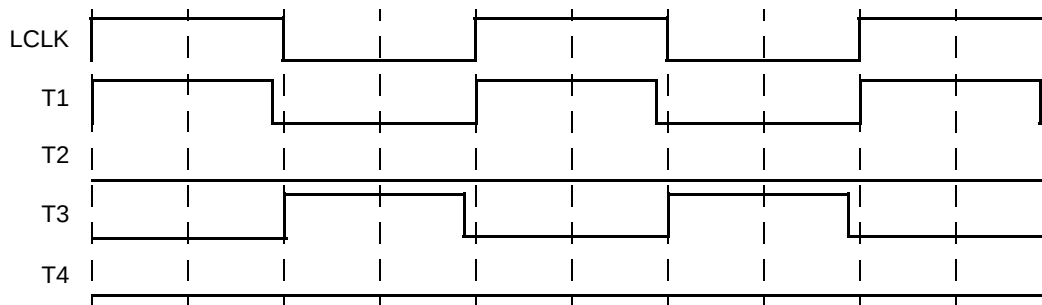
Figure 12-55. UPM Clock Scheme for \text{LCRR}[\text{CLKDIV}] = 2
