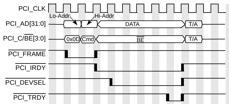
Figure 15-62. DAC Single-Beat Write Example
