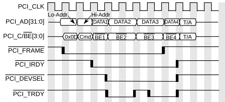
Figure 15-63. DAC Burst Write Example
