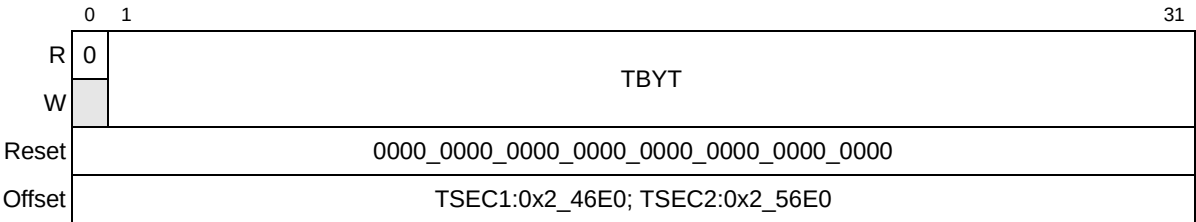
Figure 13-73. Transmit Byte Counter Register Definition
