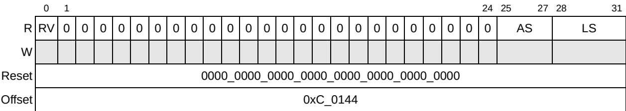
Figure 16-23. Port Link Maintenance Response Command and Status Register (PLMRESPCSR)
