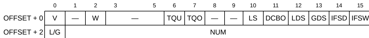
Figure 39-29. IMA Interrupt Queue Entry
