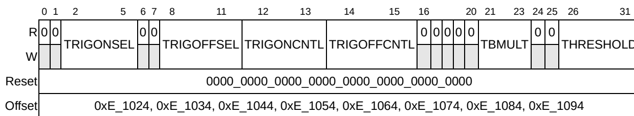
Figure 18-6. Performance Monitor Local Control Registers B1–B8 (PMLCB1–PMLCB8)
