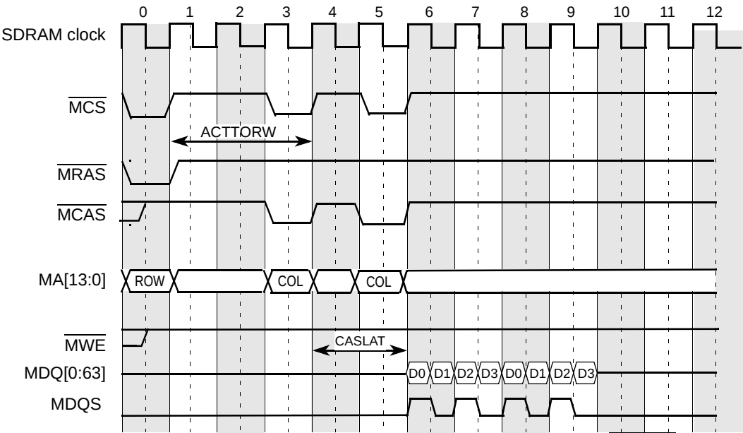
Figure 9-26. DDR SDRAM Burst Read Timing—ACTTORW = 3, MCAS Latency = 2
