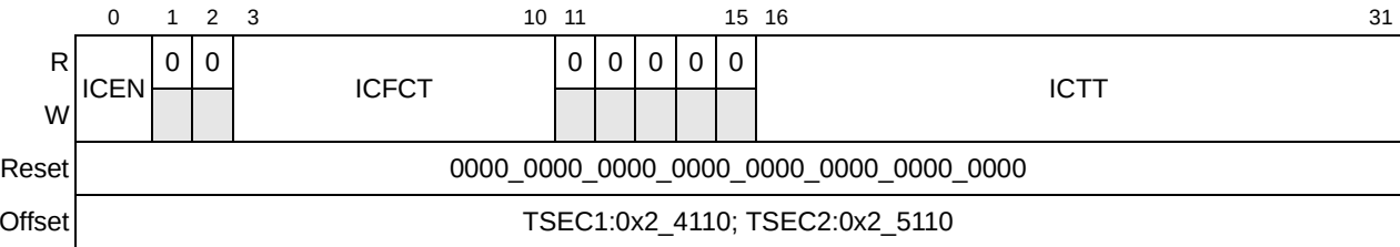
Figure 13-21. TXIC Register Definition
