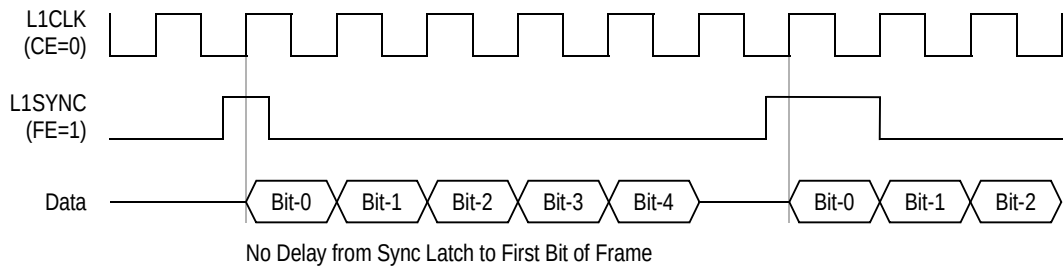
Figure 22-14. No Delay from Sync to Data (xFSD = 00)
