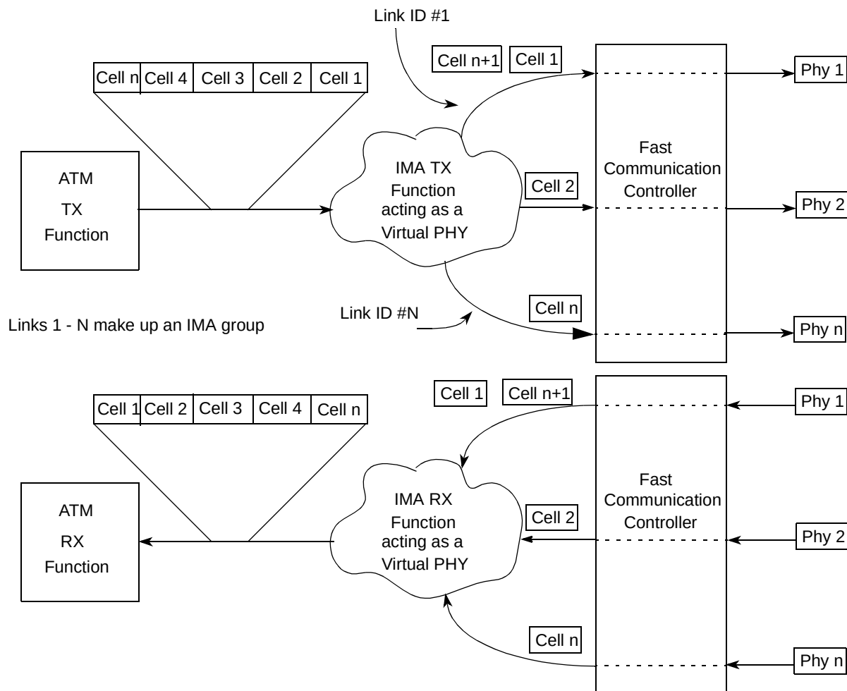
Figure 39-3. IMA Overview
