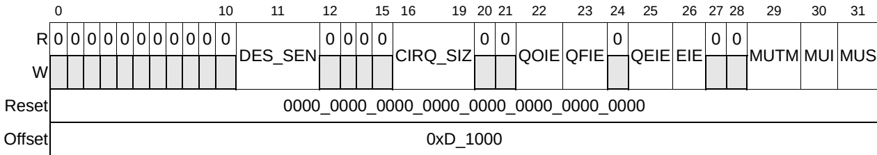
Figure 16-62. Outbound Mode Register (OMR)
