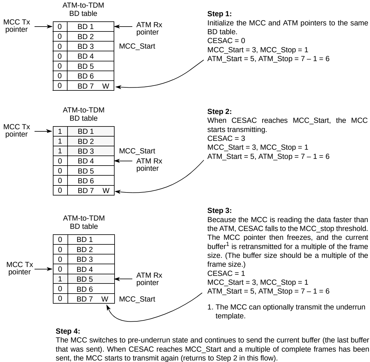
Figure 36-14. Pre-Underrun Sequence
