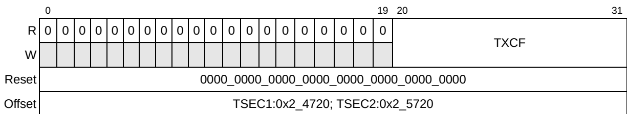
Figure 13-88. Transmit Control Frame Counter Register Definition
