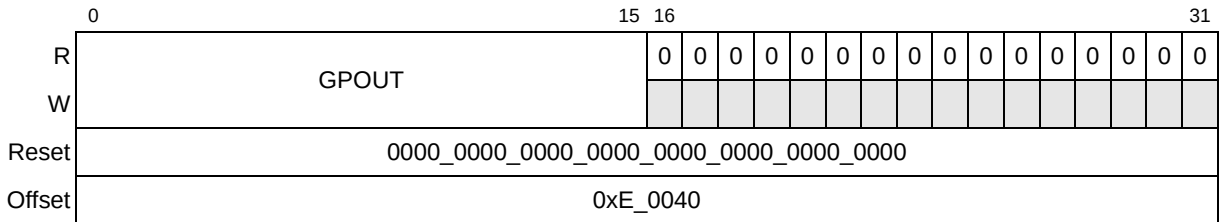
Figure 17-8. General-Purpose Output Data Register (GPOUTDR)
