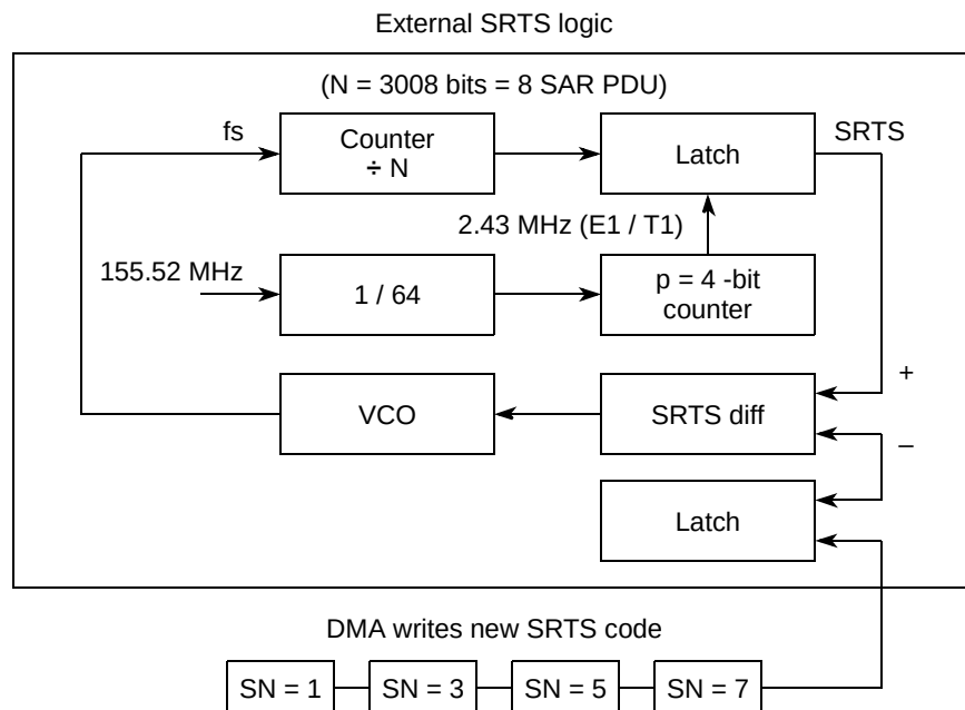
Figure 36-32. AAL1 SRTS Clock Recovery Using External Logic
