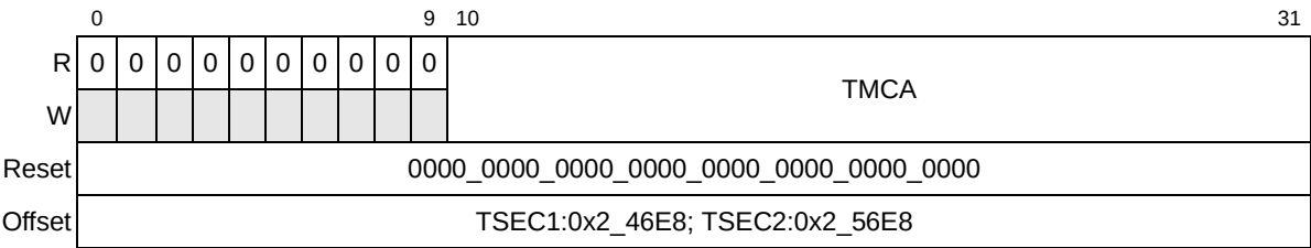
Figure 13-75. Transmit Multicast Packet Counter Register Definition
