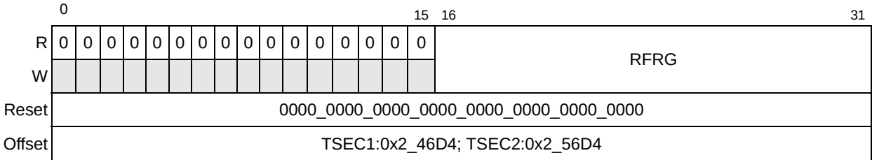
Figure 13-70. Receive Fragments Counter Register Definition
