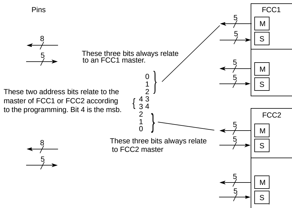
Figure 23-5. Connection of the Master Address
