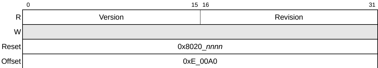
Figure 17-14. Processor Version Register (PVR)
