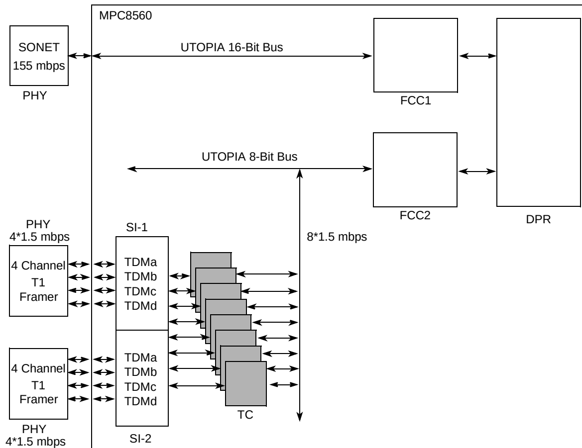
Figure 38-14. Example of Serial ATM Application
