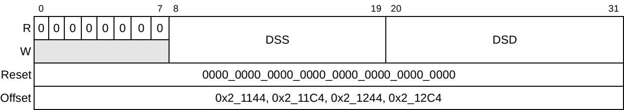
Figure 15-20. Destination Stride Registers (DSR n )
