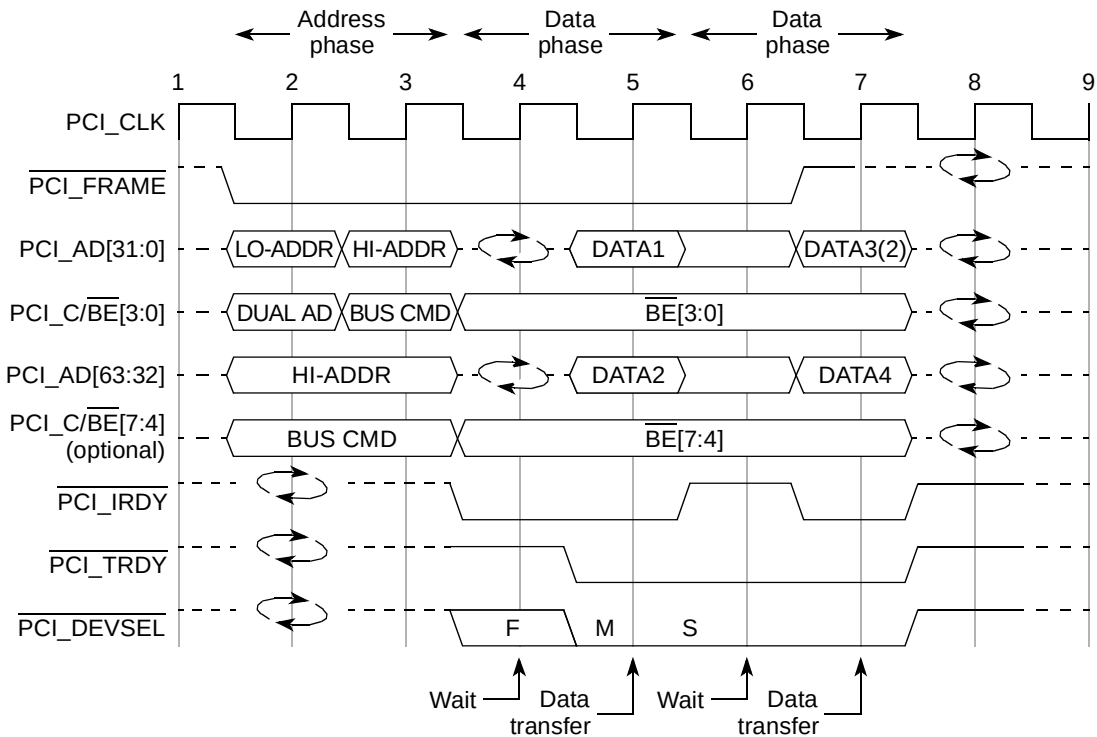
Figure 16-64. 64-Bit Dual Address Read Cycle
