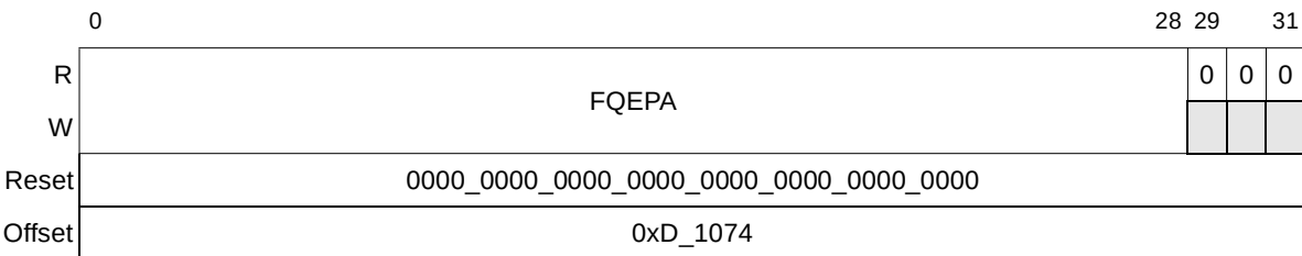
Figure 17-73. Inbound Frame Queue Enqueue Pointer Address Registers (IFQEPAR)
