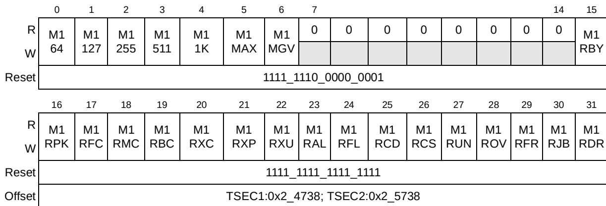
Figure 14-94. Carry Mask Register 1 (CAM1) Register Definition
