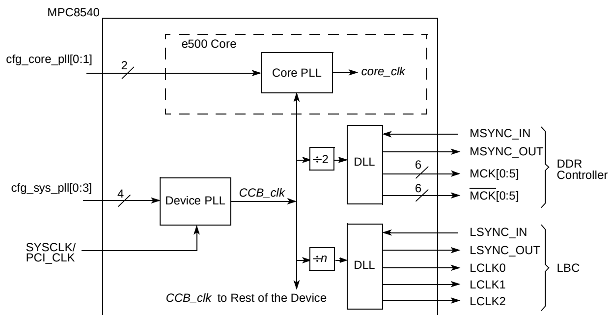
Figure 4-6. Clock Subsystem Block Diagram
