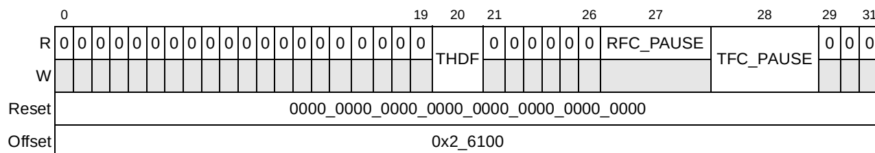
Figure 21-15. TCTRL Register Definition
