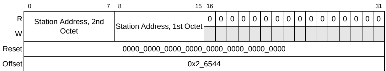
Figure 21-37. Station Address Part 2 Register Definition
