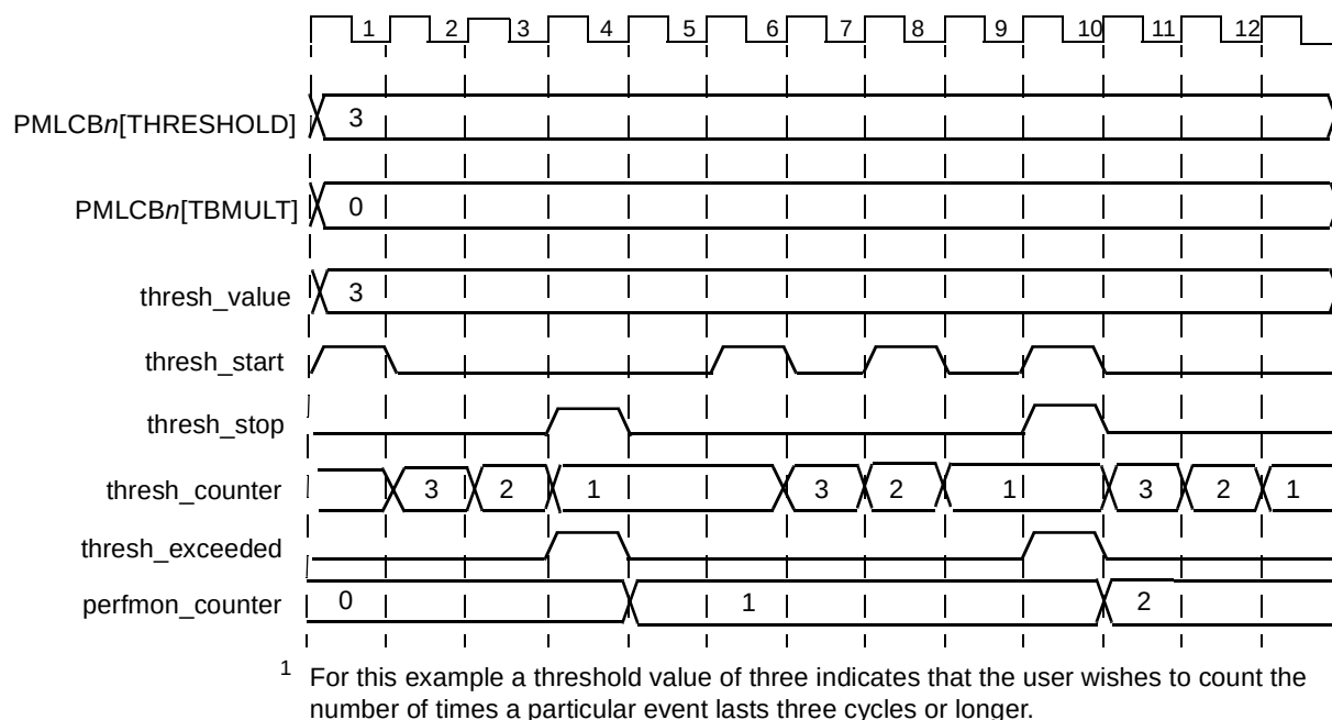
Figure 19-9. Duration Threshold Event Sequence Timing Diagram
