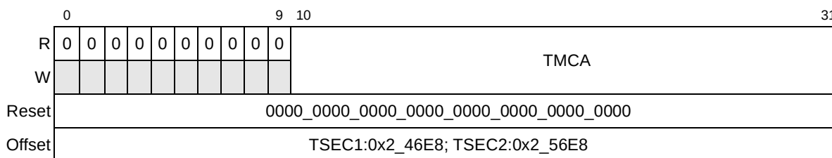
Figure 14-75. Transmit Multicast Packet Counter Register Definition
