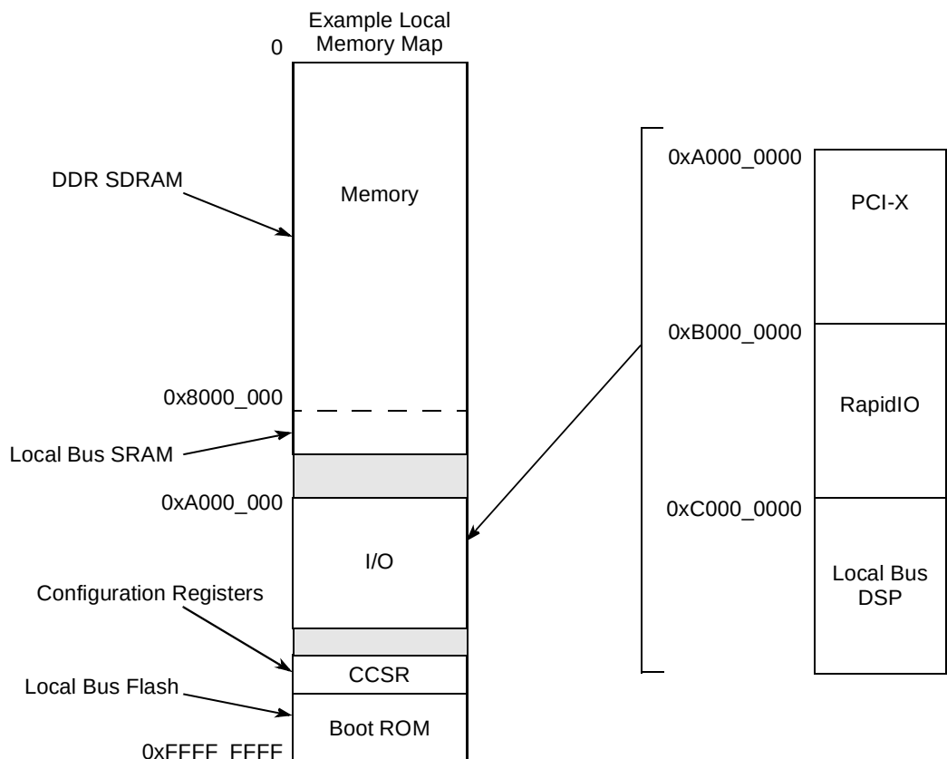
Figure 2-1. Local Memory Map Example
