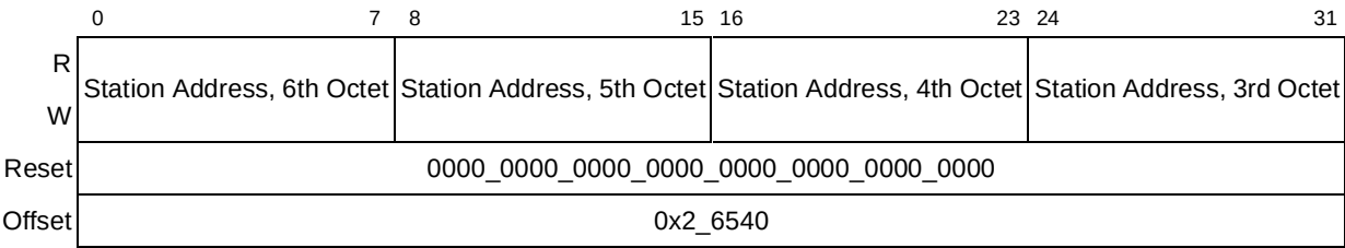
Figure 21-36. Station Address Part 1 Register Definition
