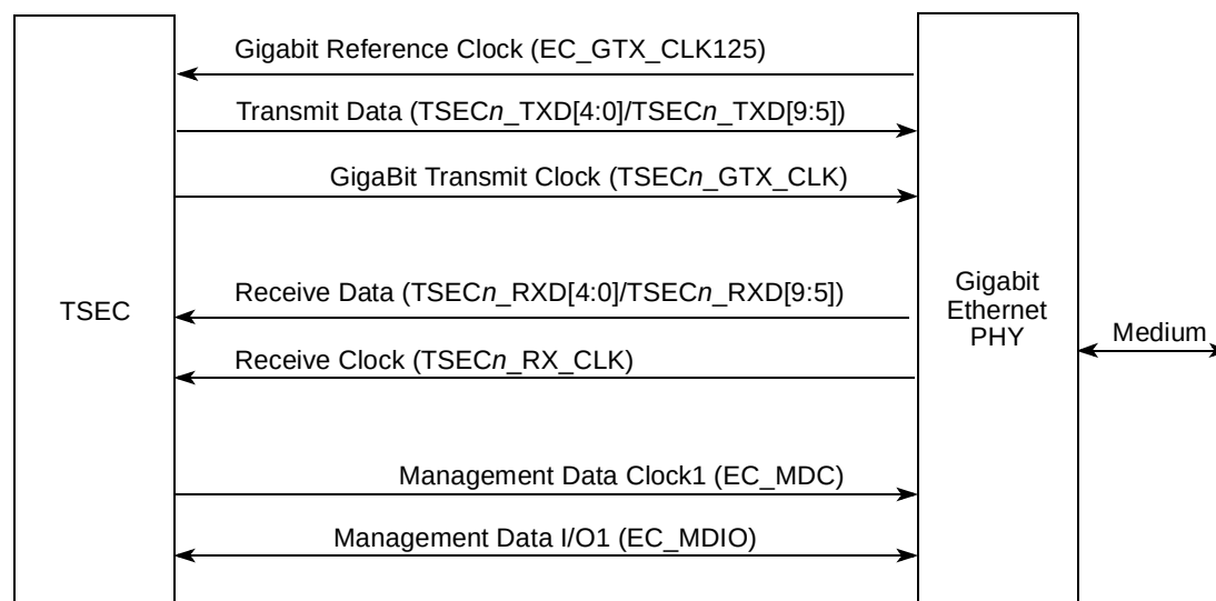
Figure 14-114. TSEC-RTBI Connection
