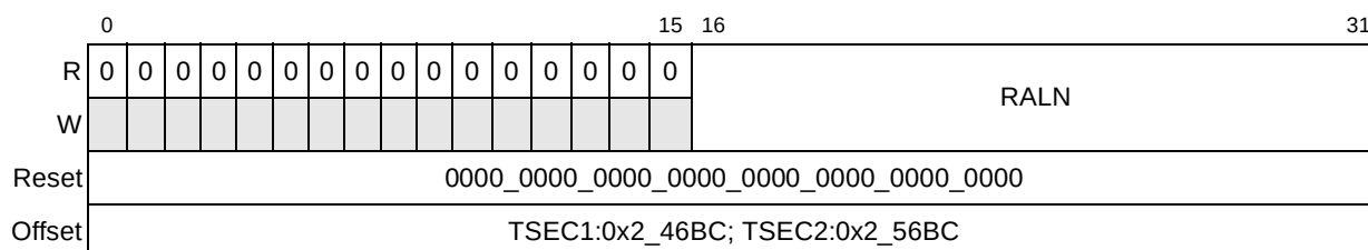
Figure 14-64. Receive Alignment Error Counter Register Definition
