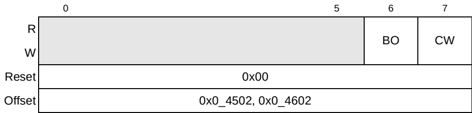
Figure 12-14. Alternate Function Register (UAFR)
