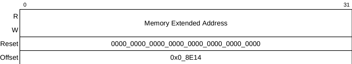
Figure 16-20. PCI/X Error Extended Address Capture Register (ERR_EXT_ADDR)
