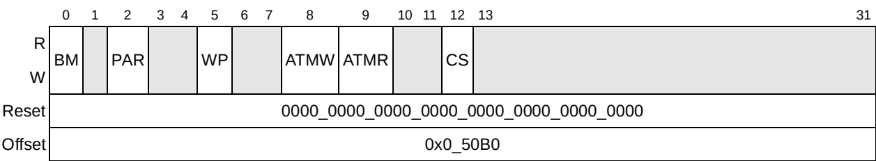
Figure 13-13. Transfer Error Status Register (LTESR)
