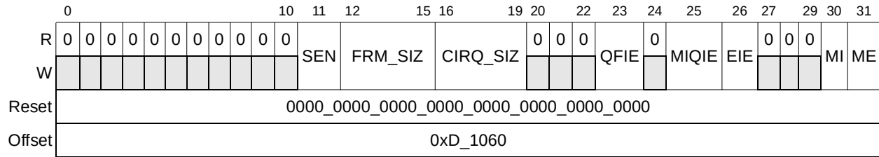
Figure 17-70. Inbound Mode Register (IMR)
