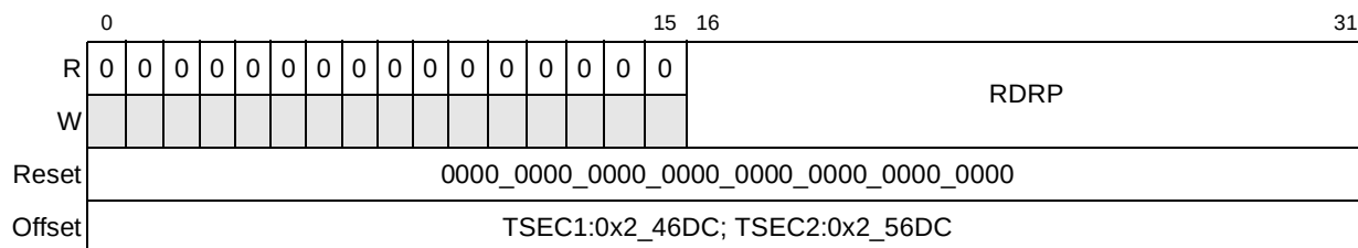
Figure 14-72. Receive Dropped Packet Counter Register Definition
