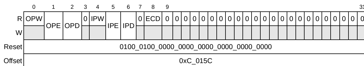
Figure 17-26. Port Control Command and Status Register (PCCSR)
