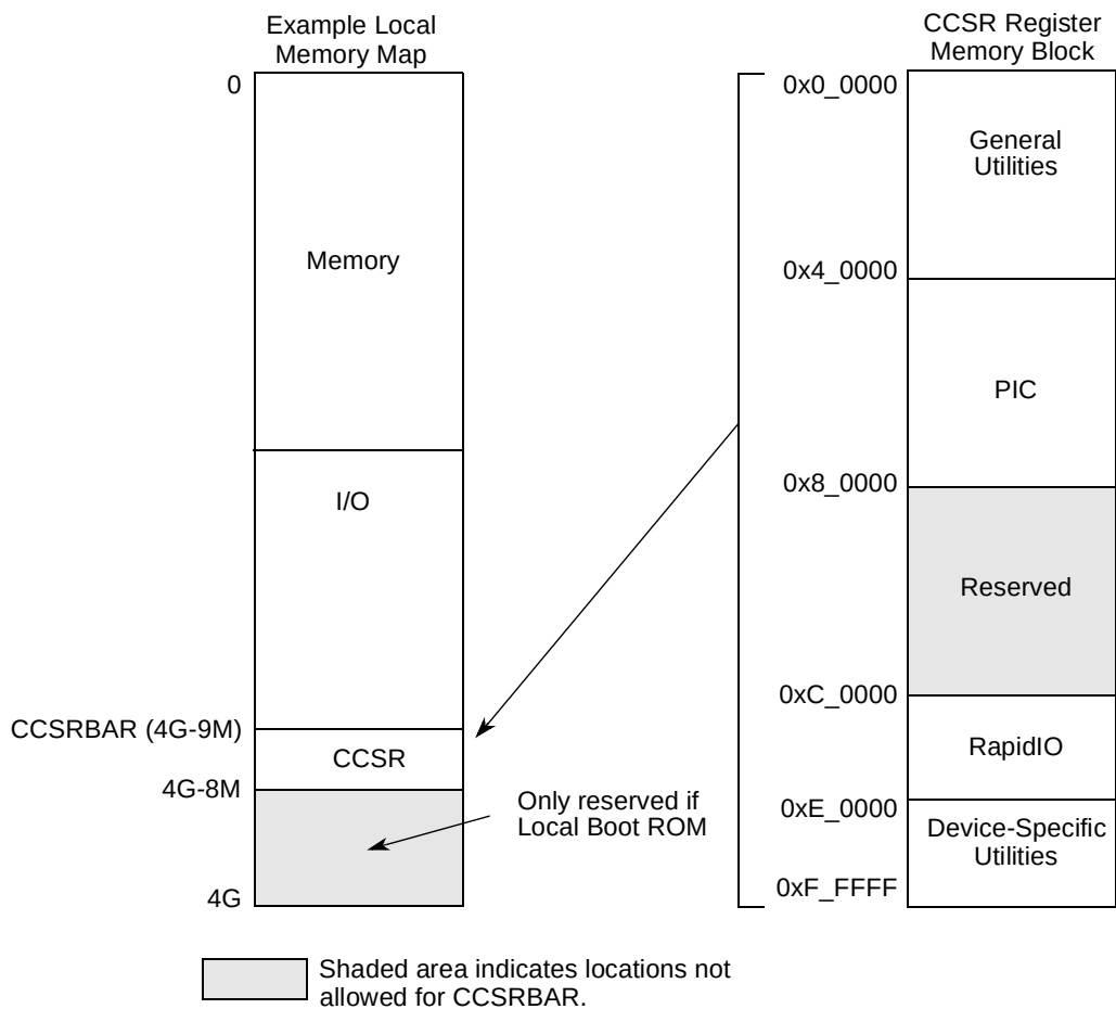
Figure 2-4. Top-Level Register Map Example
