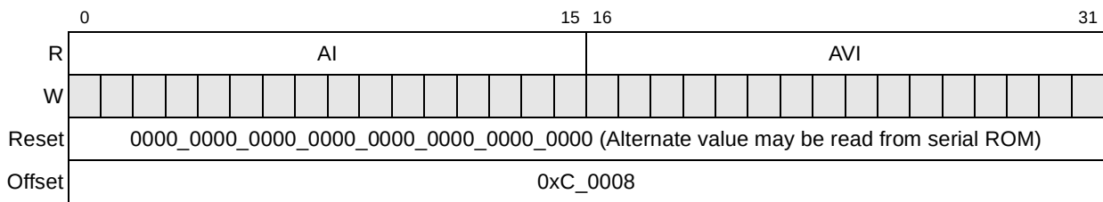
Figure 17-5. Assembly Identity Capability Register (AIDCAR)
