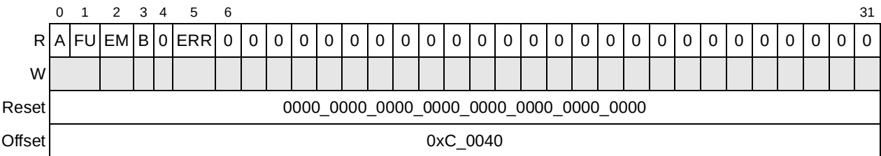
Figure 17-11. Mailbox Status Register (MSR)
