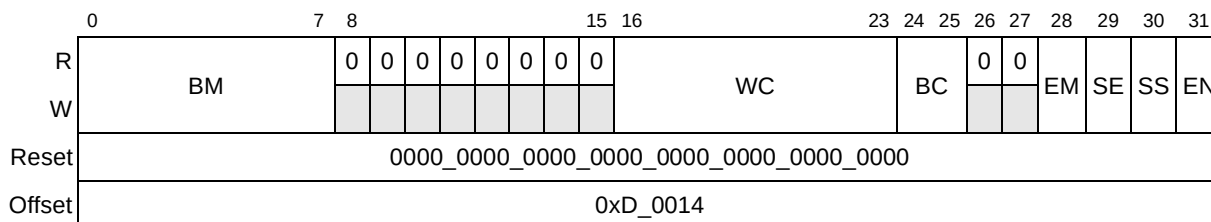
Figure 17-29. Port Error Injection Register (PEIR)
