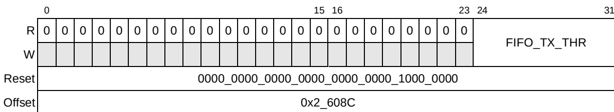
Figure 21-12. FIFO_TX_THR Register Definition
