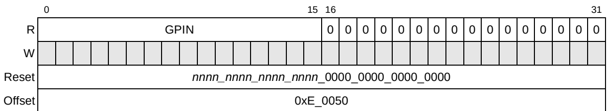
Figure 18-9. General-Purpose Output Data Register (GPINDR)
