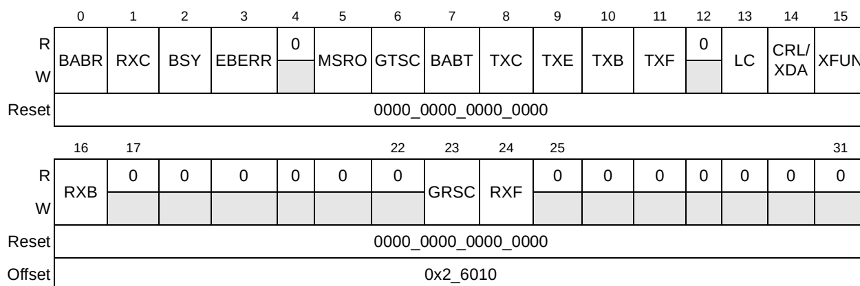
Figure 21-5. IEVENT Register Definition
