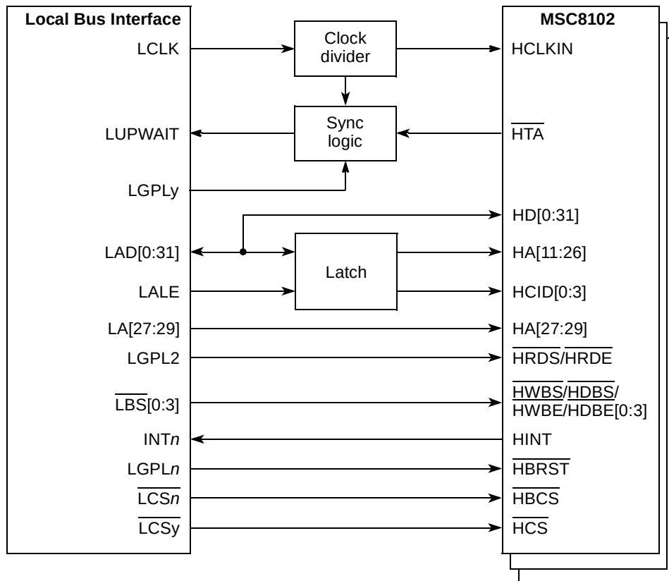
Figure 13-85. Interface to MSC8102 DSI in Synchronous Mode
