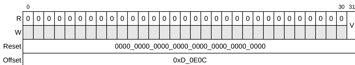
Figure 17-42. Port Error Capture Status Register (PECSR)
