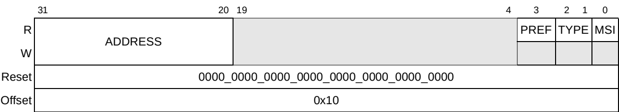
Figure 16-37. PCI Configuration and Status Register Base Address Register (PCSRBAR)
