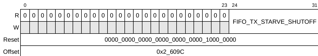
Figure 21-14. FIFO_TX_STARVE_SHUTOFF Register Definition
