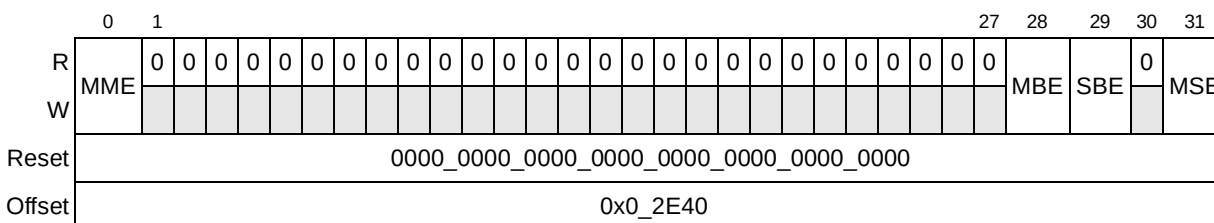
Figure 9-15. Memory Error Detect Register (ERR_DETECT)
