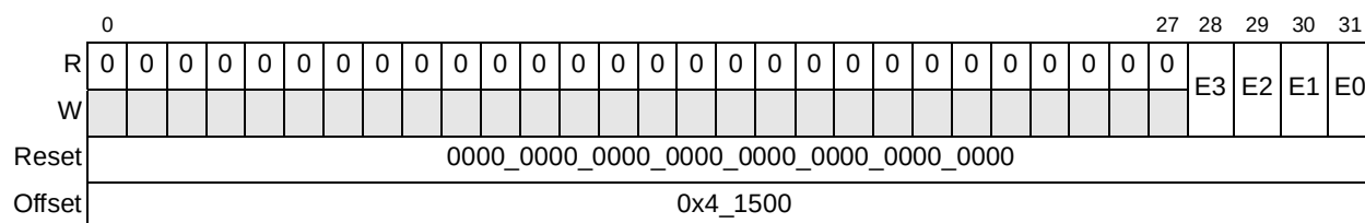
Figure 10-23. Message Enable Register (MER)
