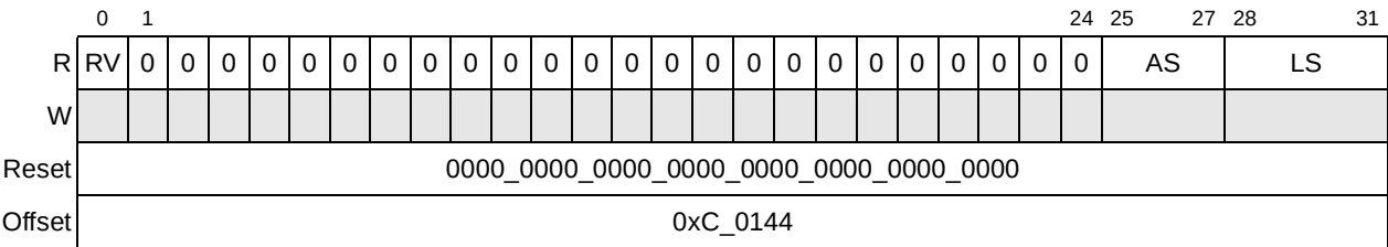
Figure 17-23. Port Link Maintenance Response Command and Status Register (PLMRESPCSR)
