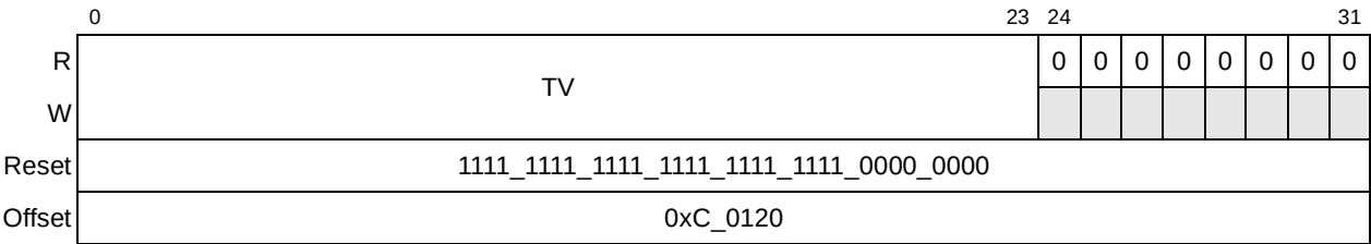
Figure 17-19. Port Link Time-Out Control Command and Status Register (PLTOCCSR)
