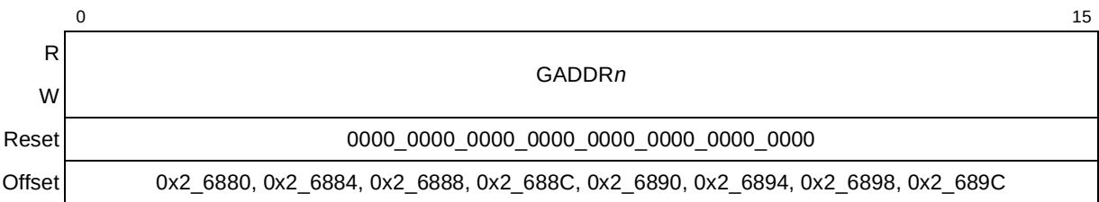
Figure 21-39. GADDR n Register Definition
