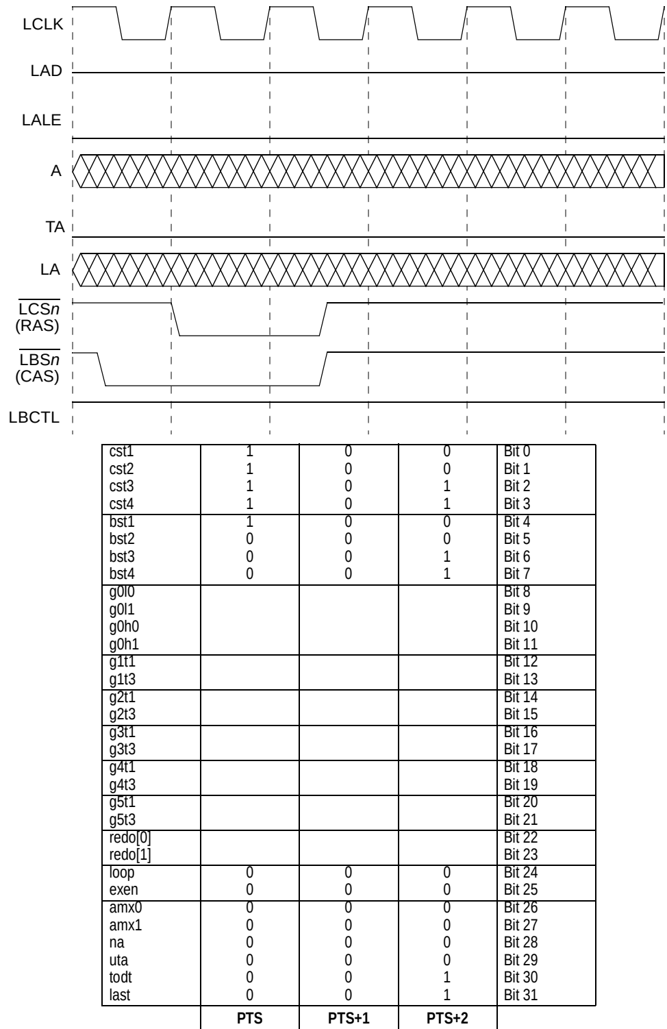
Figure 13-66. Refresh Cycle (CBR) to FPM DRAM
