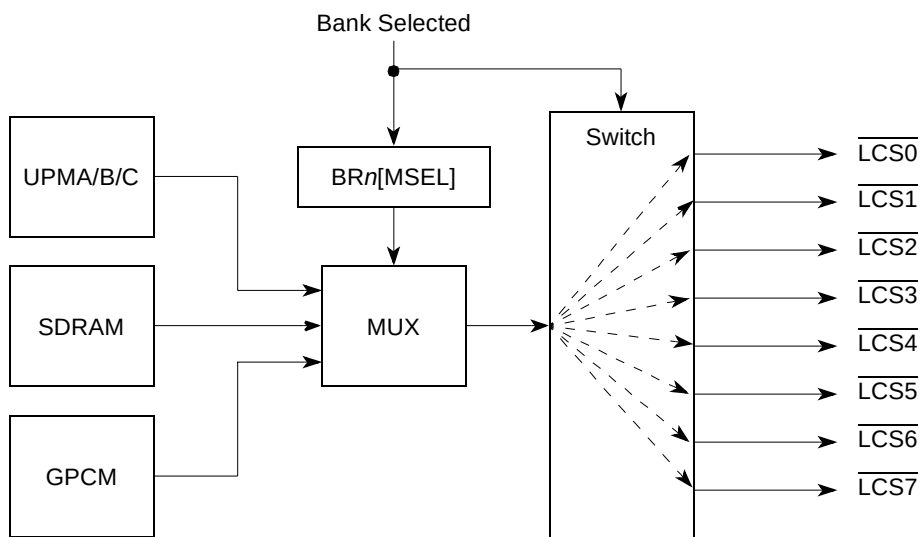
Figure 13-59. \overline{\text{LCS}}_n Signal Selection
