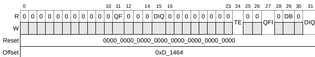
Figure 17-75. Doorbell Status Register (DSR)
