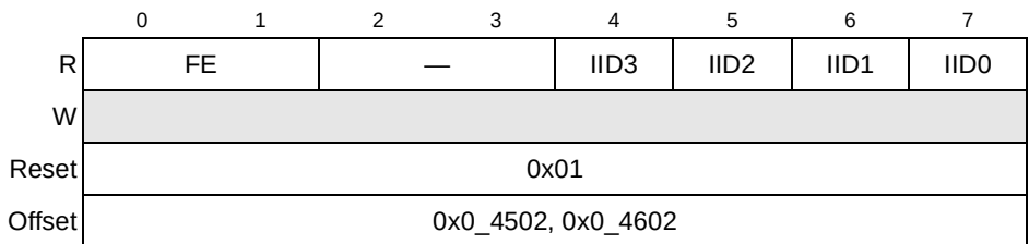
Figure 12-7. Interrupt ID Registers (UIIR)
