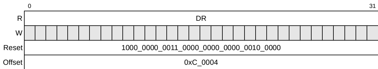
Figure 17-4. Device Information Capability Register (DICAR)
