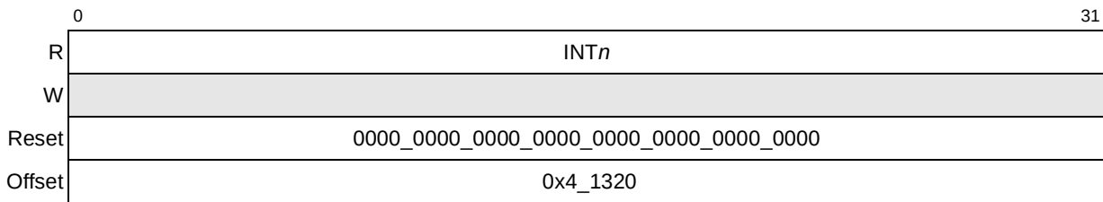
Figure 10-17. IRQ_OUT Summary Register 1 (IRQSR1)
