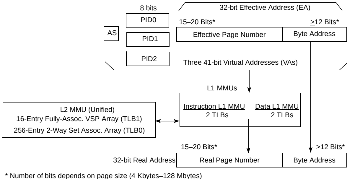
Figure 5-8. Effective-to-Real Address Translation Flow
