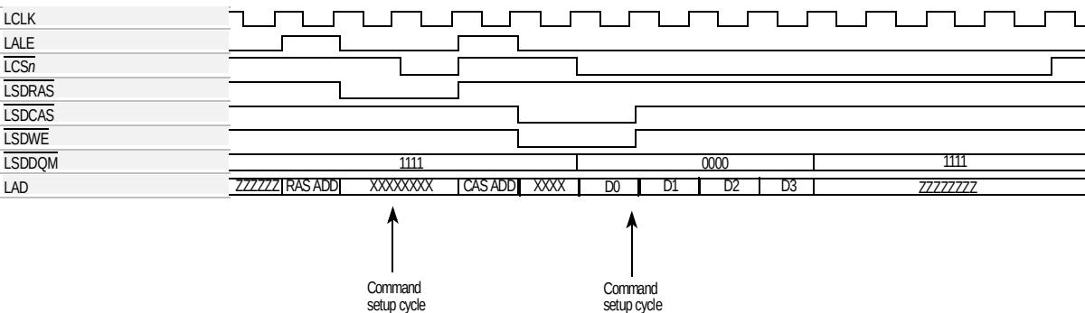
Figure 13-40. BUFCMD = 1, LCRR[BUFCMDC] = 2
