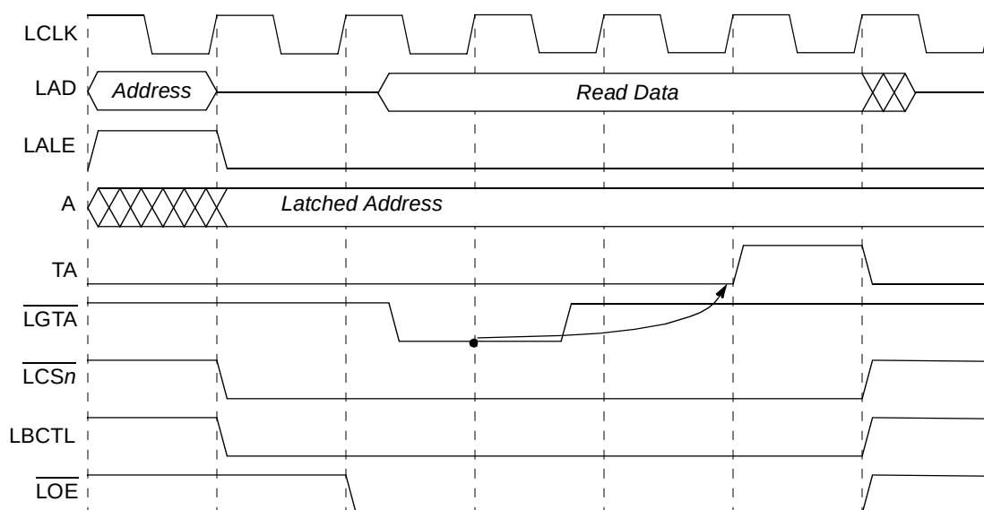
Figure 13-32. External Termination of GPCM Access
