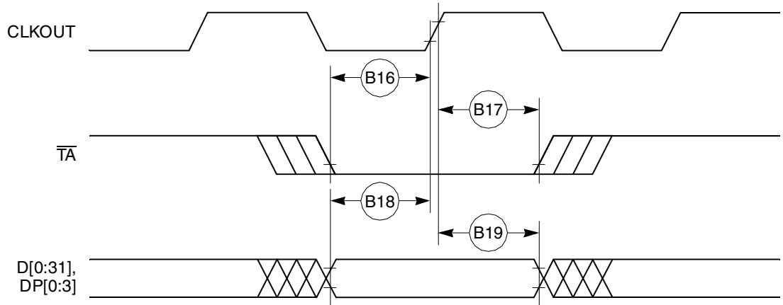
Figure 8. Input Data Timing in Normal Case
