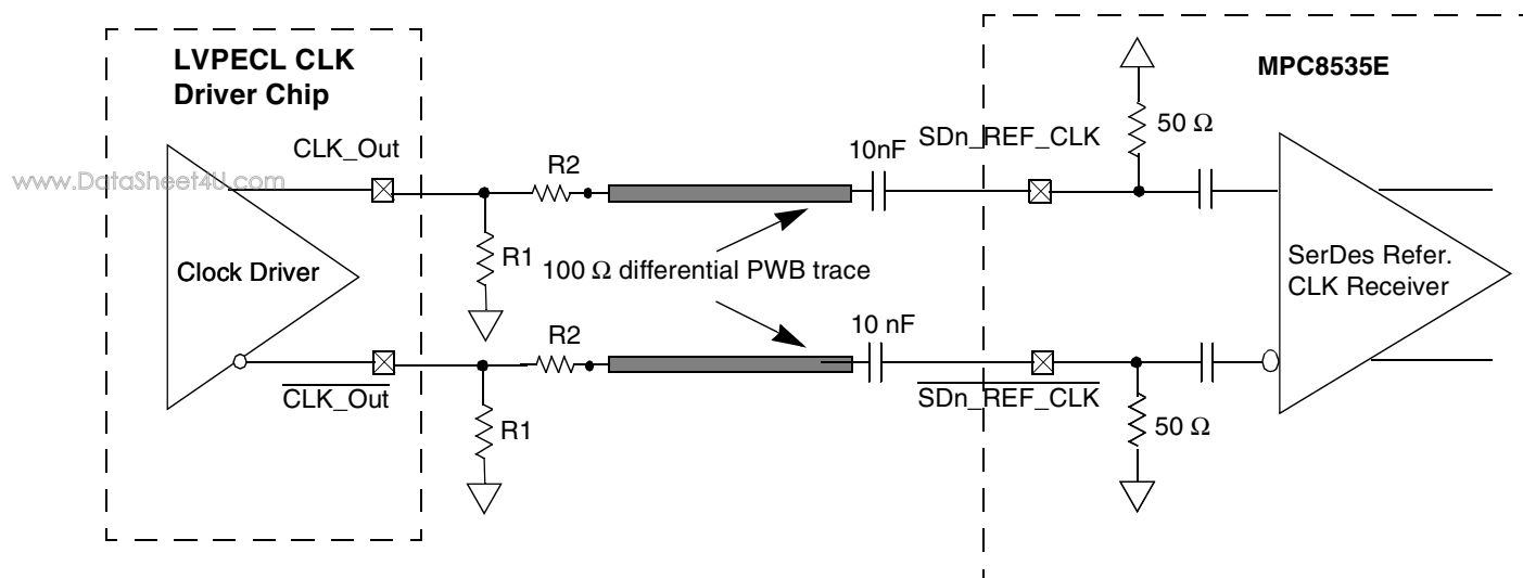
Figure 64. AC-Coupled Differential Connection with LVPECL Clock Driver (Reference Only)
