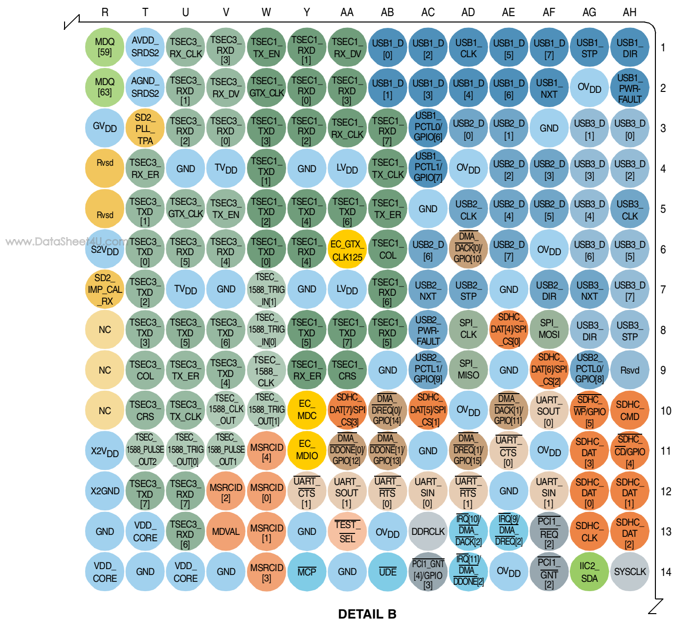
Figure 4. MPC8535E Pin Map Detail B
