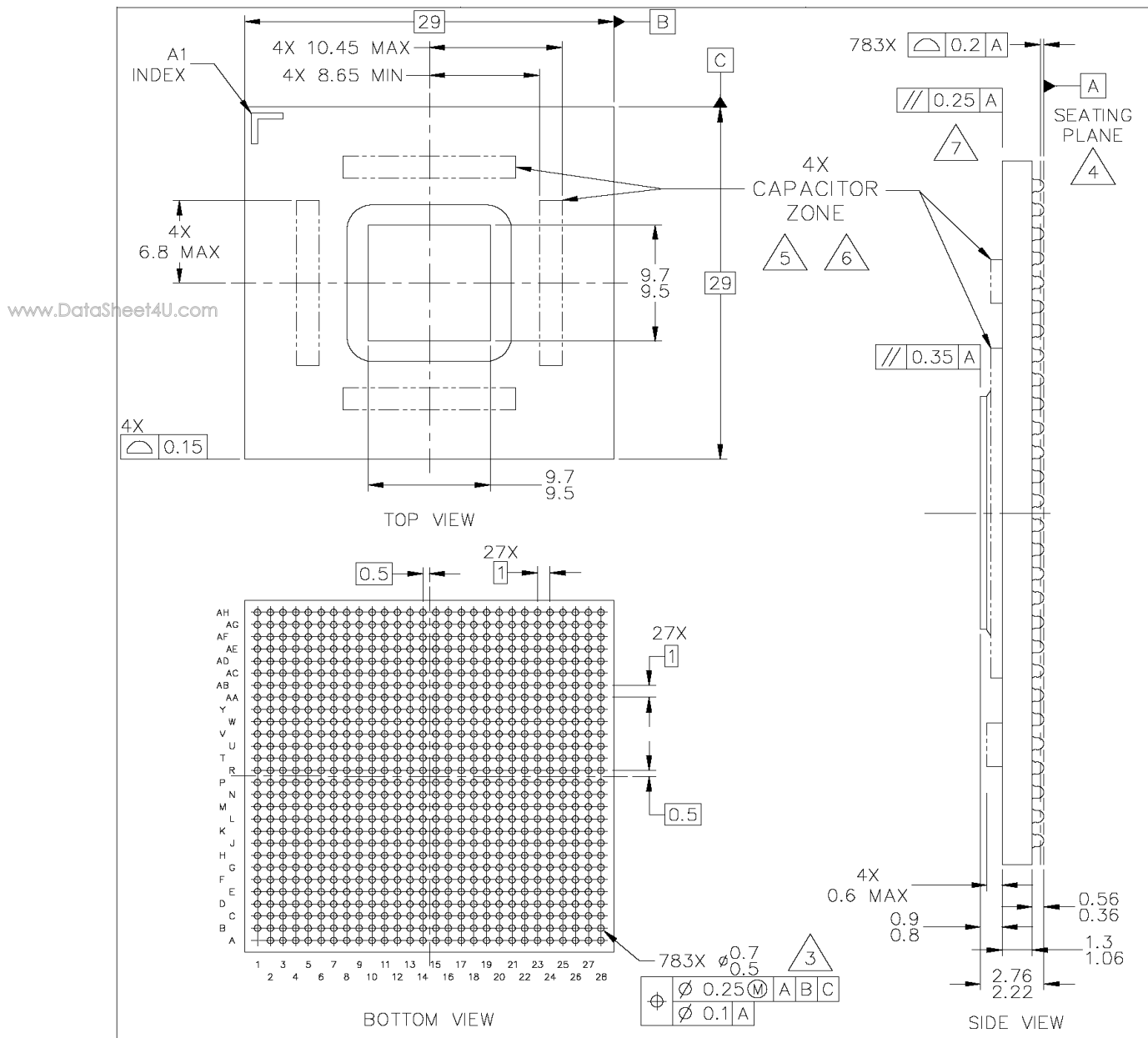
Figure 81. Mechanical Dimensions and Bottom Surface Nomenclature of the MPC8535E FC-PBGA
