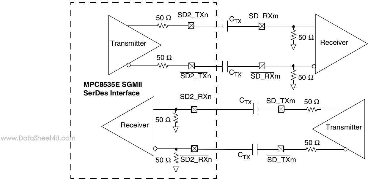
Figure 29. 4-Wire AC-Coupled SGMII Serial Link Connection Example
