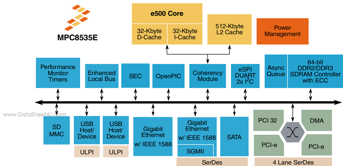
Figure 1. MPC8535E Block Diagram
