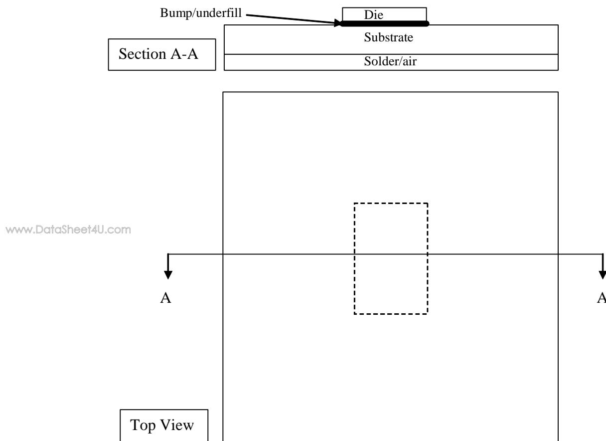
Figure 72. System Level Thermal Model for MPC8535E (Not to Scale)
