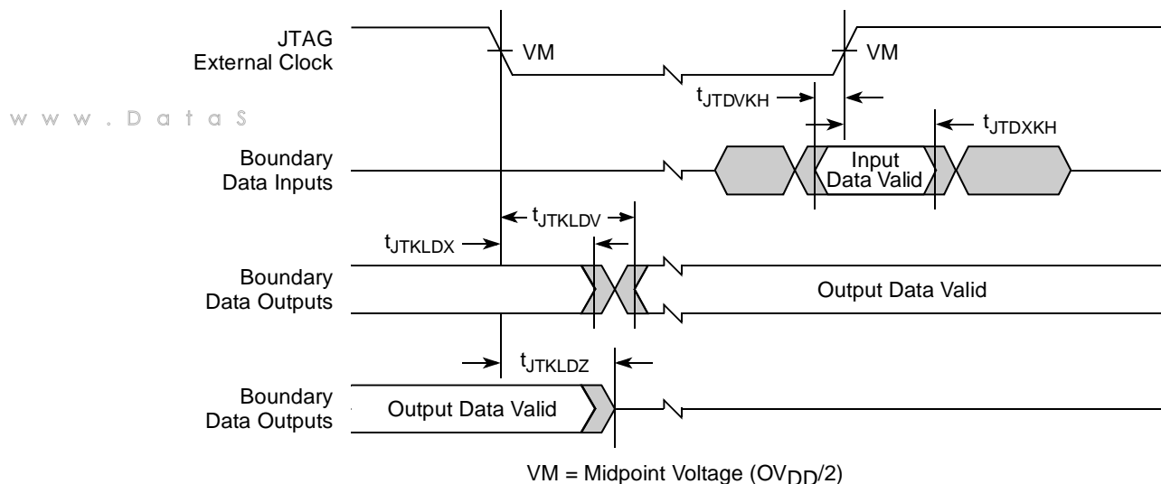
Figure 33. Boundary-Scan Timing Diagram
