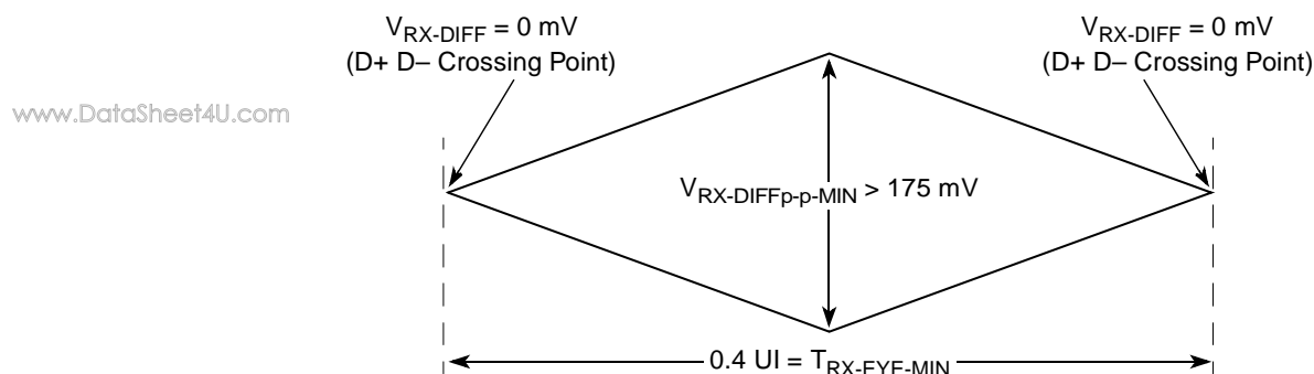
Figure 53. Minimum Receiver Eye Timing and Voltage Compliance Specification
