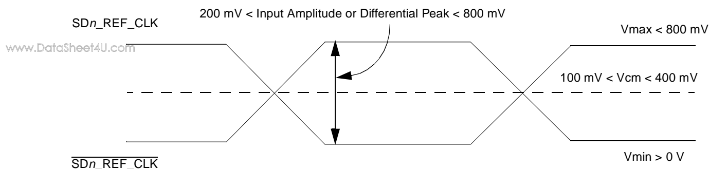
Figure 42. Differential Reference Clock Input DC Requirements (External DC-Coupled)
