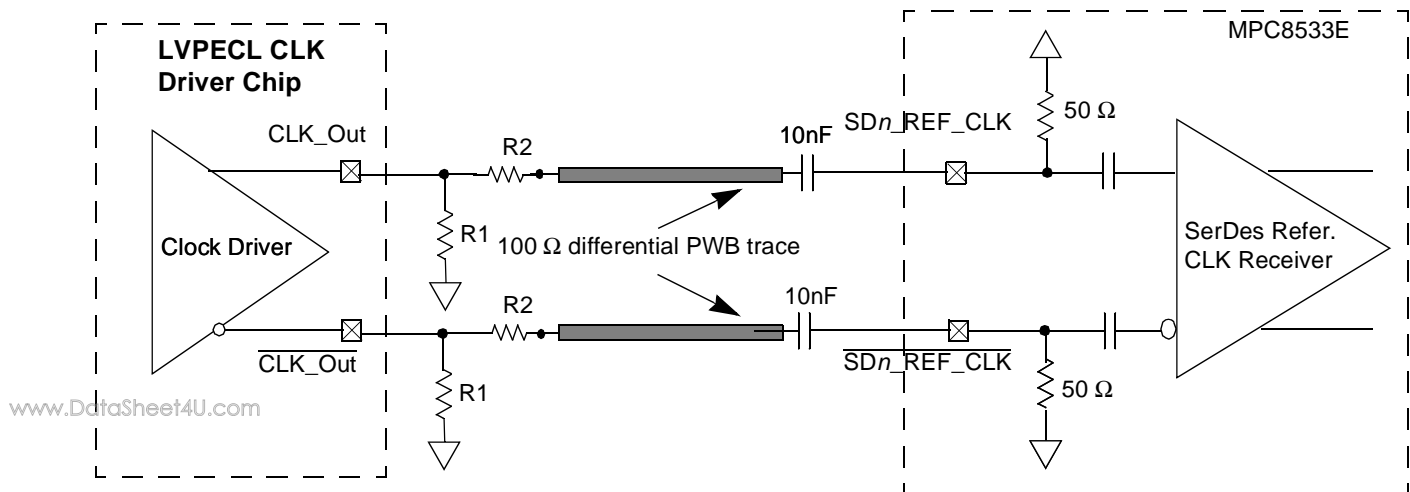
Figure 47. AC-Coupled Differential Connection with LVPECL Clock Driver (Reference Only)
