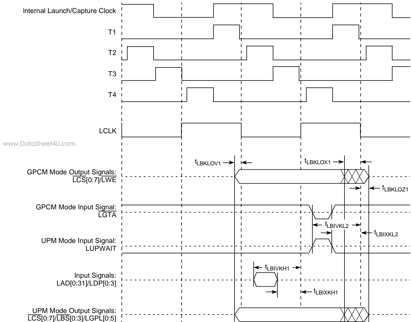
Figure 29. Local Bus Signals, GPCM/UPM Signals for LCCR[CLKDIV] = 8 or 16 (PLL Bypass Mode)
