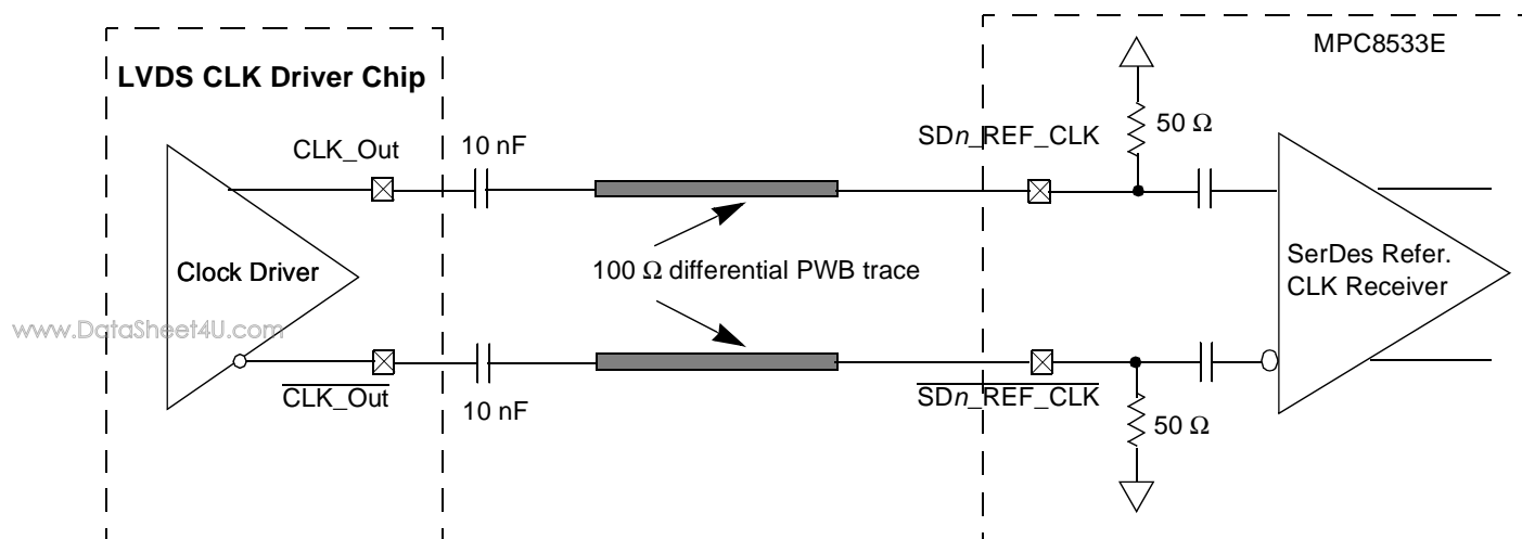
Figure 46. AC-Coupled Differential Connection with LVDS Clock Driver (Reference Only)
