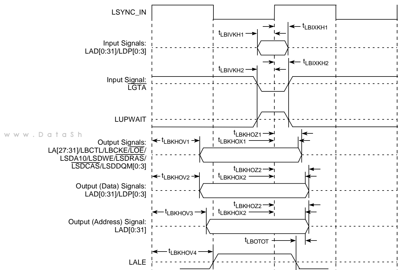
Figure 24. Local Bus Signals (PLL Enabled)
