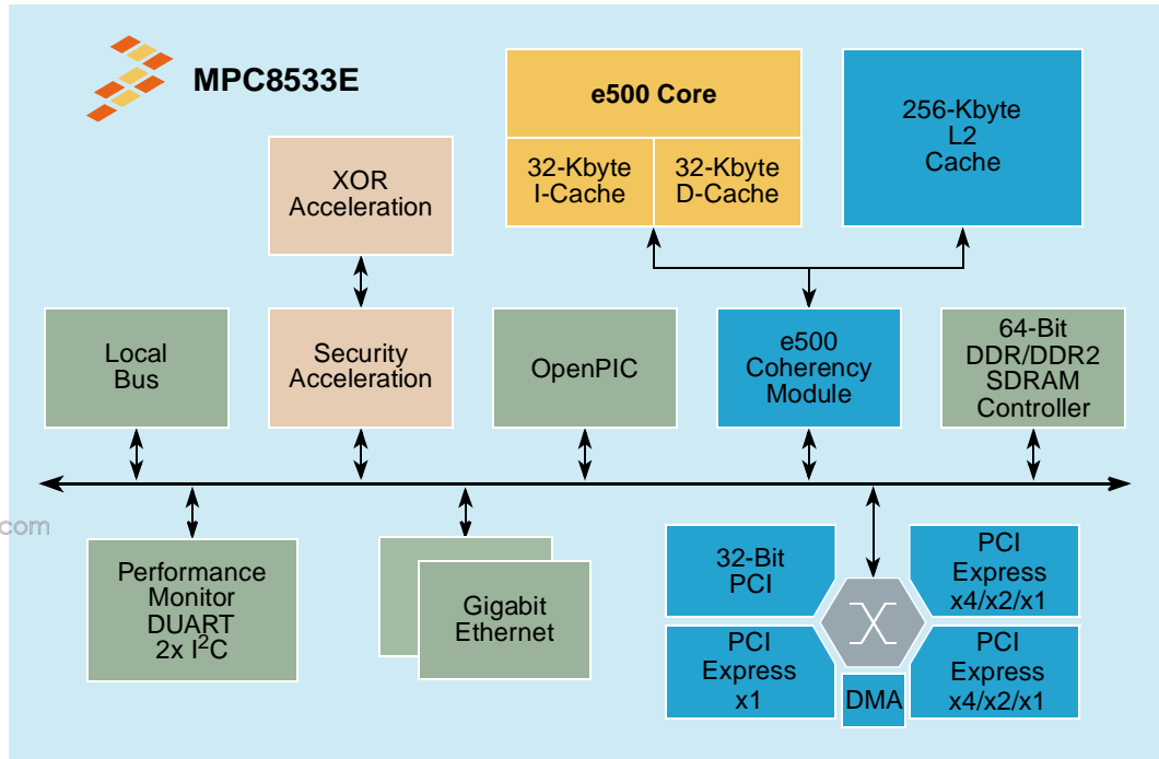
Figure 1. MPC8533E Block Diagram
