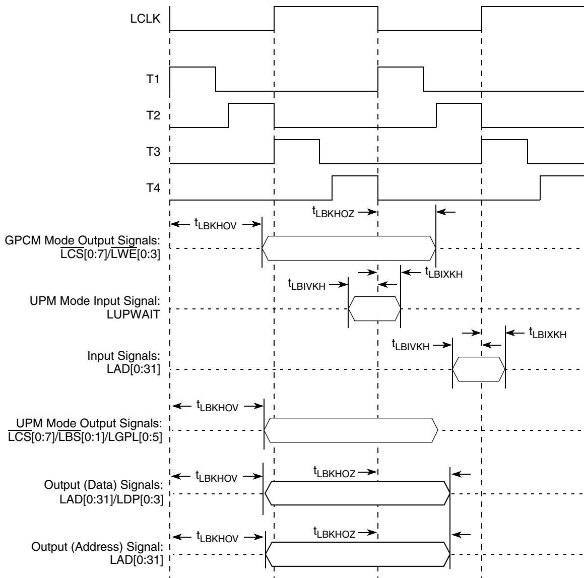
Figure 25. Local Bus Signals, GPCM/UPM Signals for \text{LCRR}[\text{CLKDIV}] = 4 (PLL Bypass Mode)
