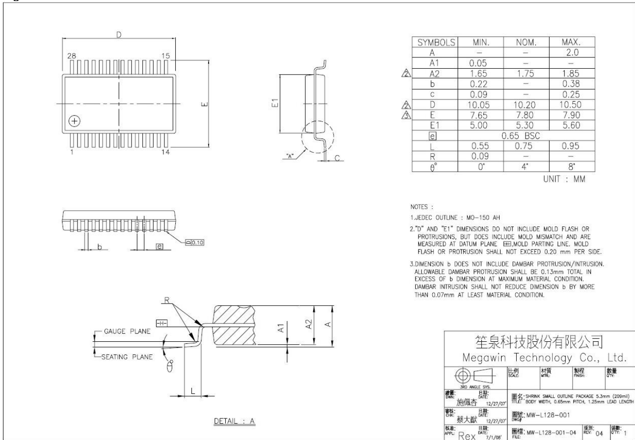
Figure 25–4. SSOP-28
