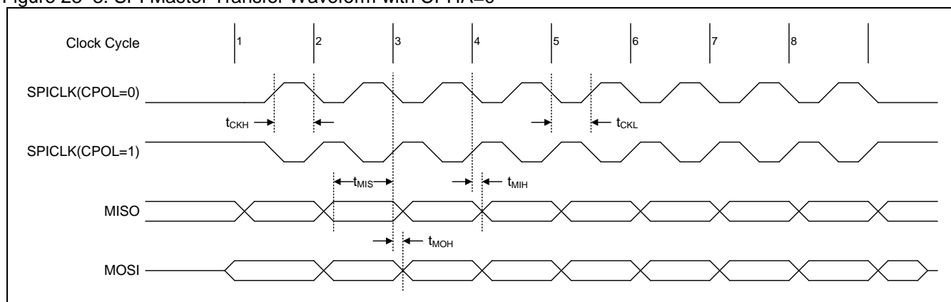
Figure 23–3. SPI Master Transfer Waveform with CPHA=0
