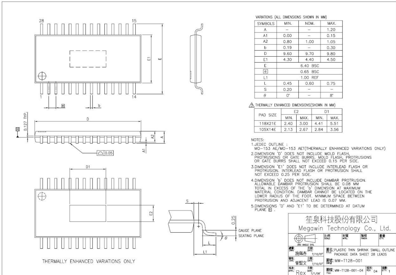
Figure 25–5. TSSOP-28
