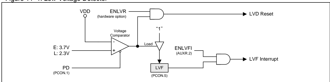
Figure 11–1. Low-Voltage Detector
