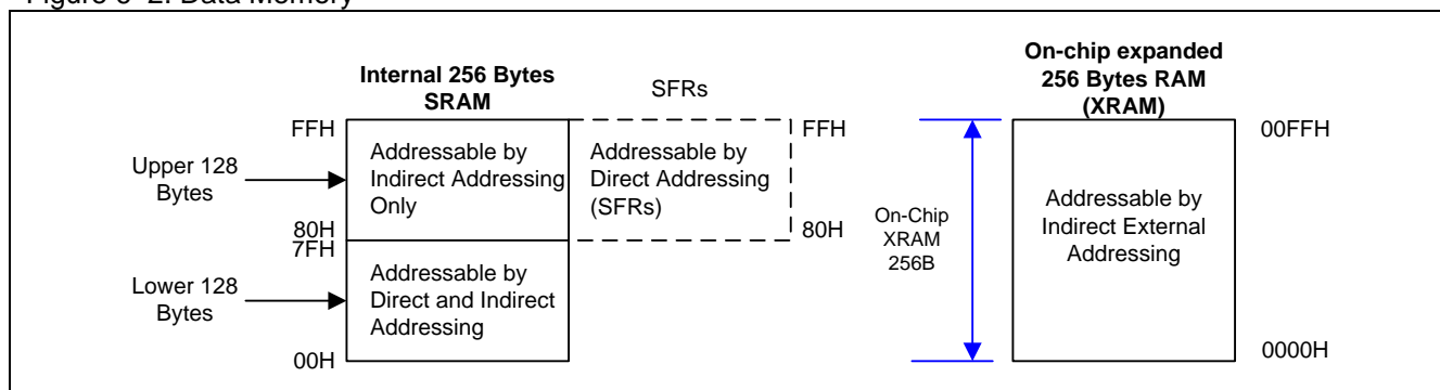
Figure 6–2. Data Memory
