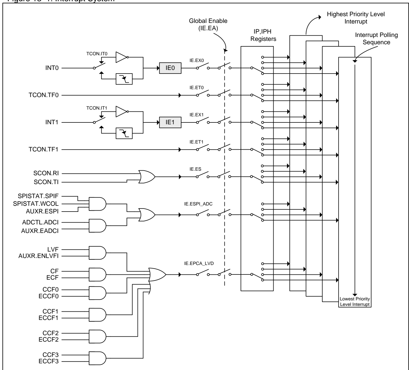
Figure 13–1. Interrupt System
