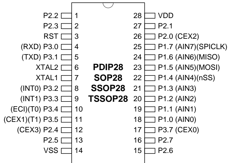
Figure 4–1. MPC82E/L54 28-Pin Top View
