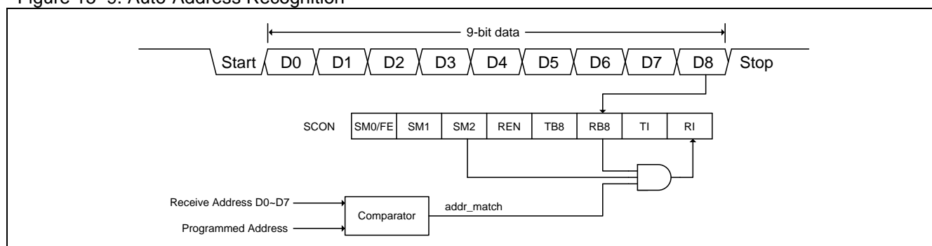
Figure 15–9. Auto-Address Recognition
