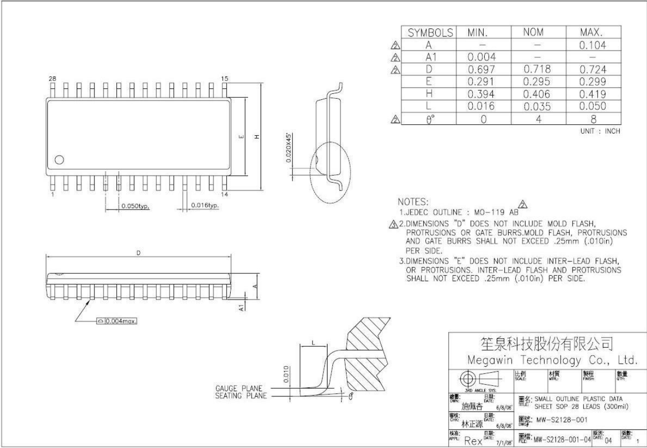
Figure 25–3. SOP-28
