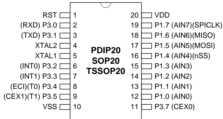
Figure 4–2. MPC82E/L54 20-Pin Top View
