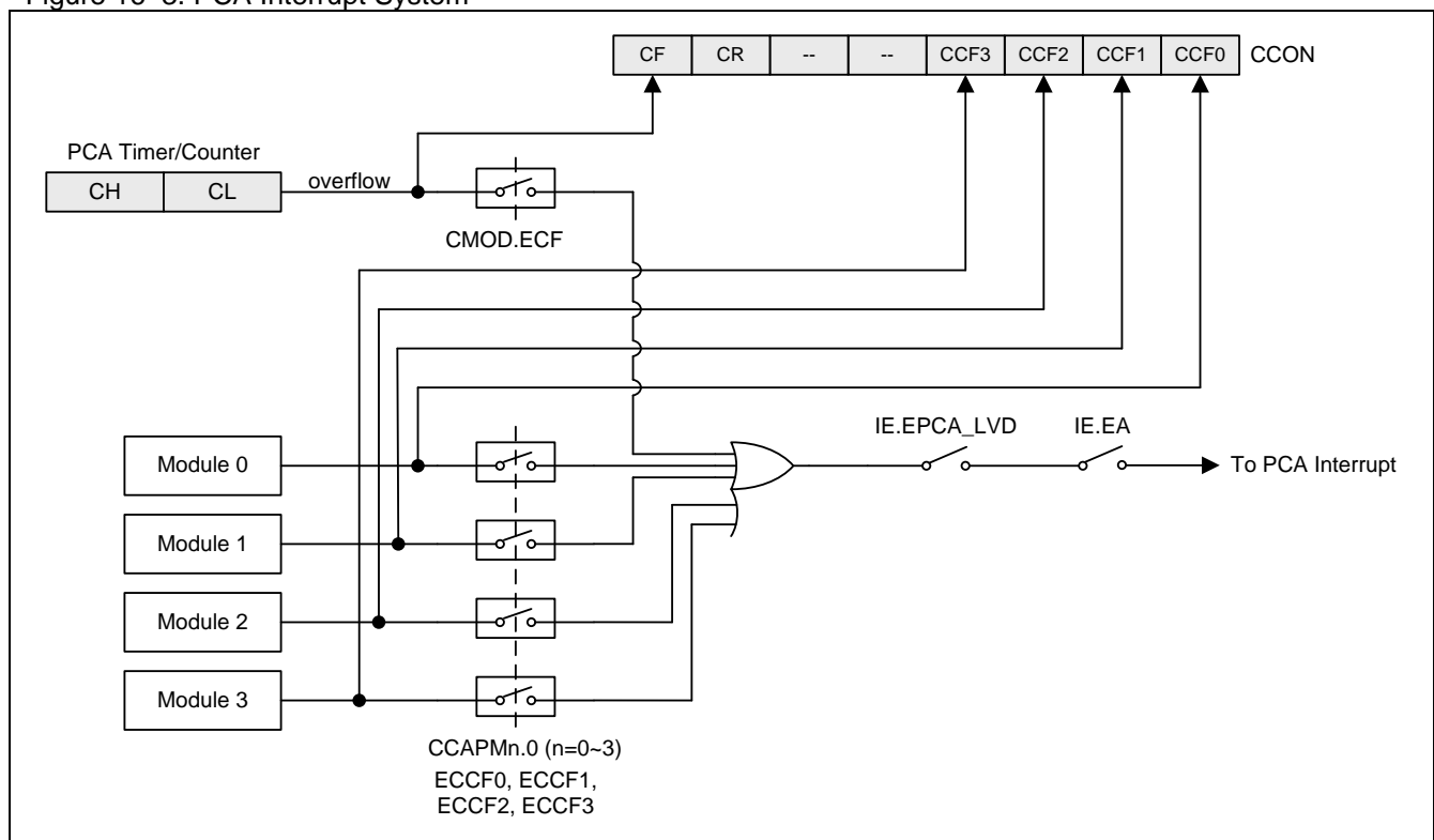
Figure 16–3. PCA Interrupt System
