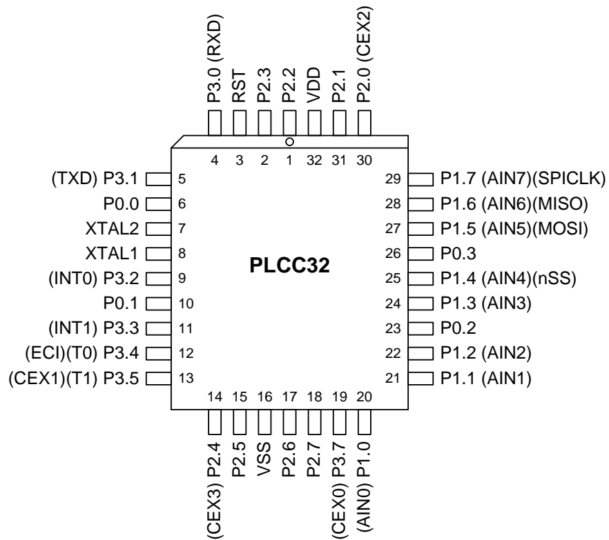
Figure 4–3. MPC82E/L54AP Top View
