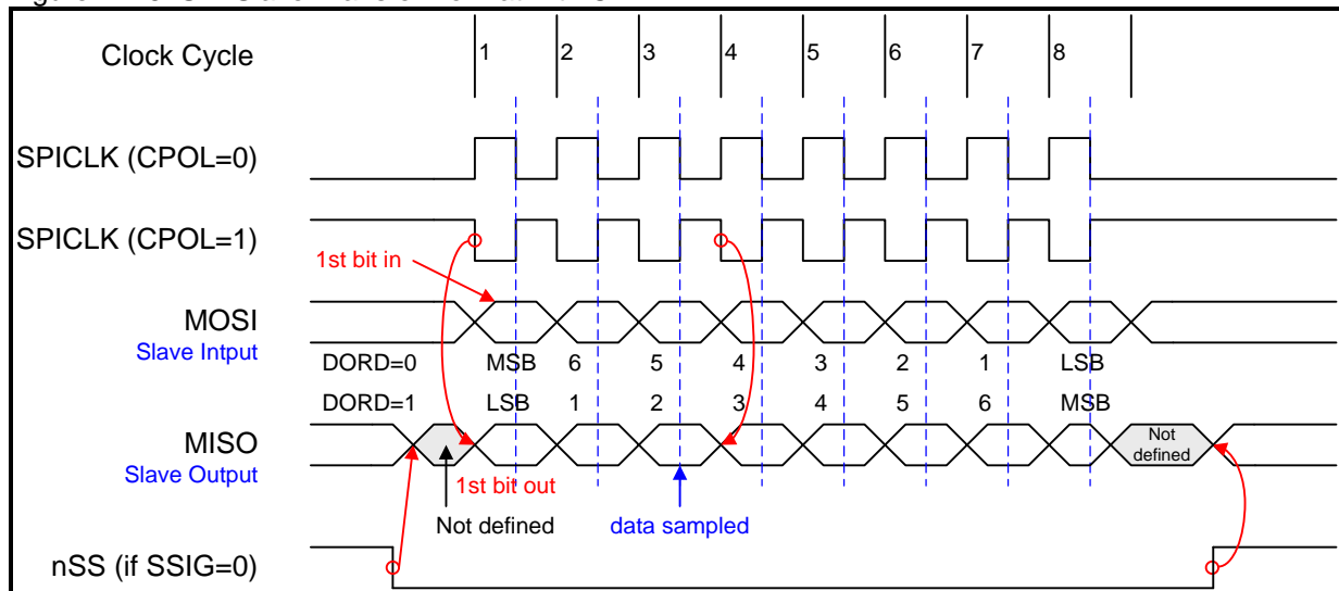
Figure 17–6. SPI Slave Transfer Format with CPHA=1
