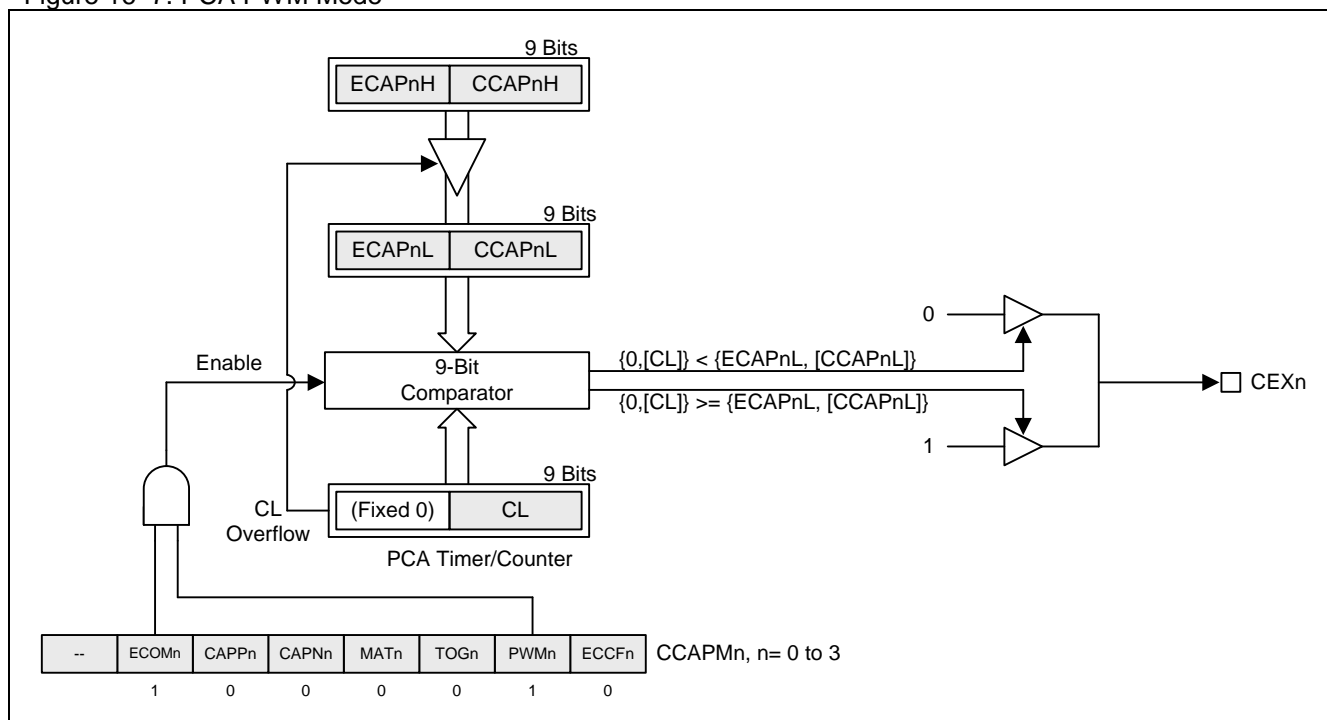
Figure 16–7. PCA PWM Mode
