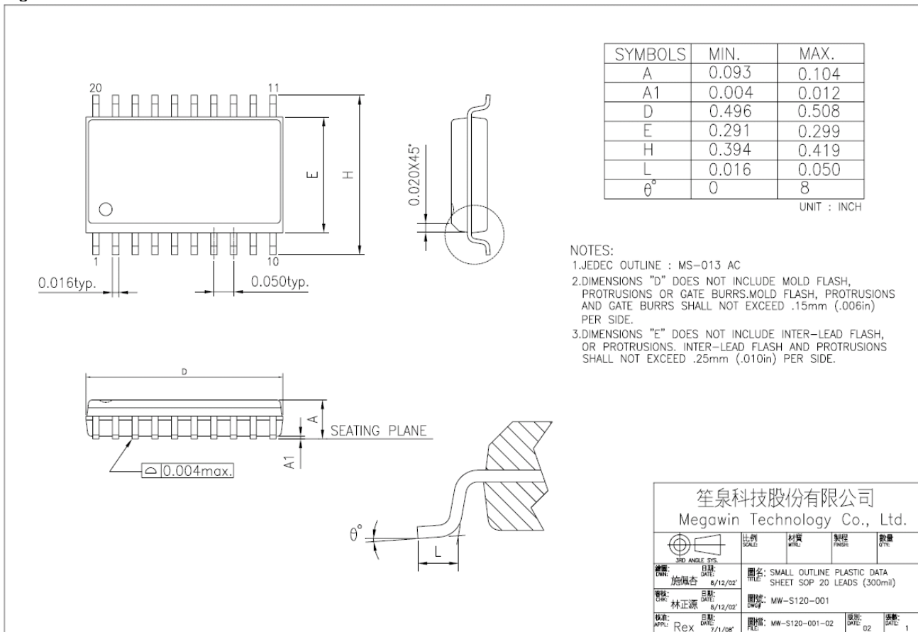
Figure 25–7. SOP-20
