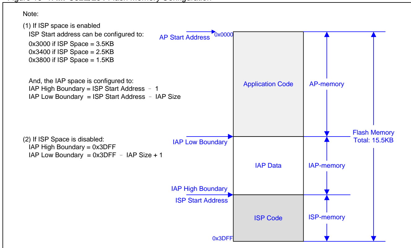
Figure 19–1. MPC82E/L54 Flash Memory Configuration
