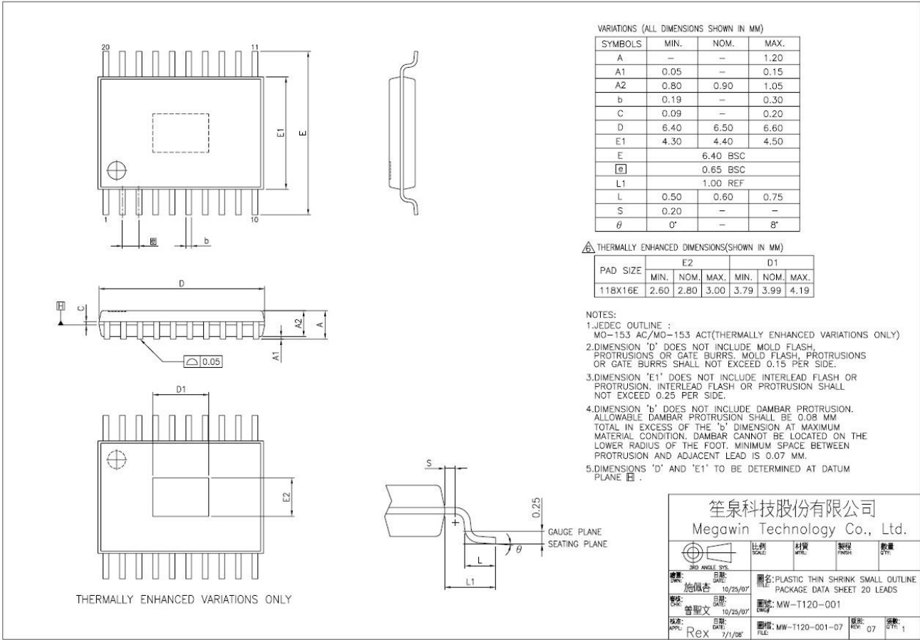
Figure 25–8. TSSOP-20
