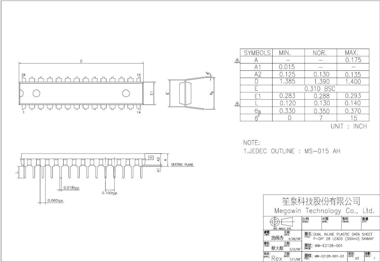
Figure 25–2. DIP-28
