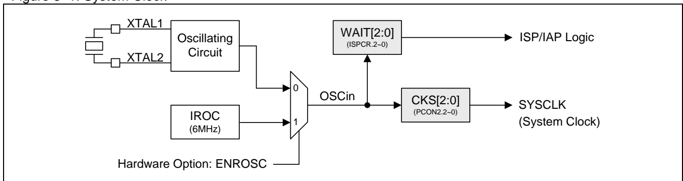
Figure 8–1. System Clock
