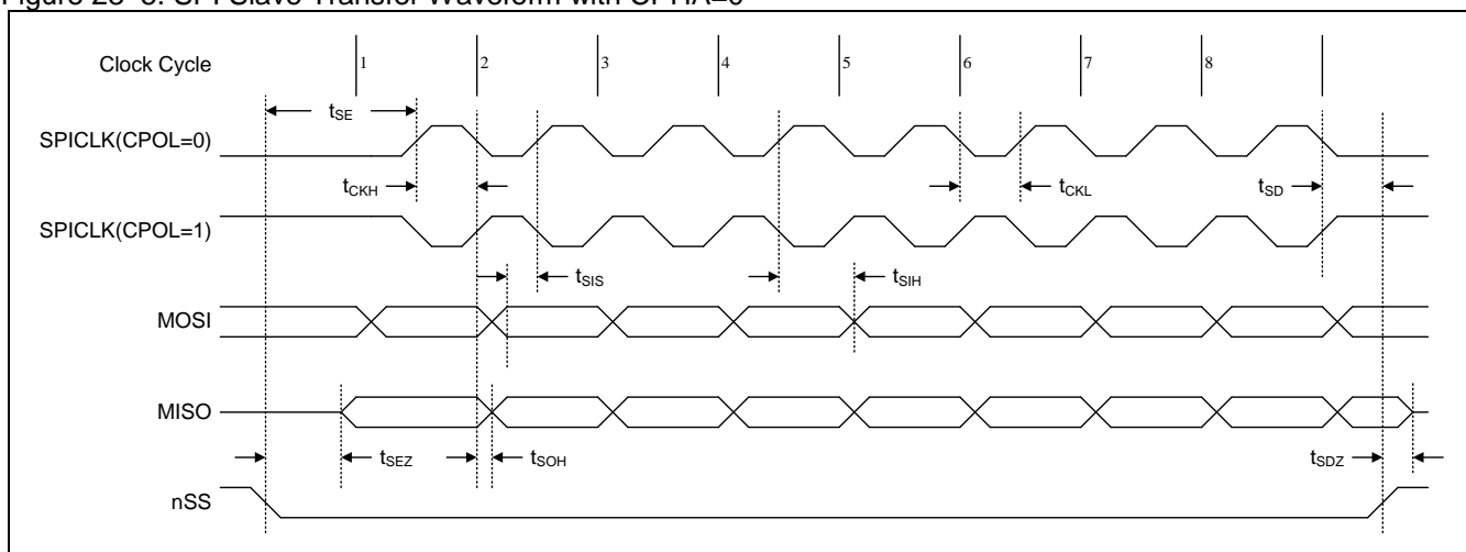
Figure 23–5. SPI Slave Transfer Waveform with CPHA=0
