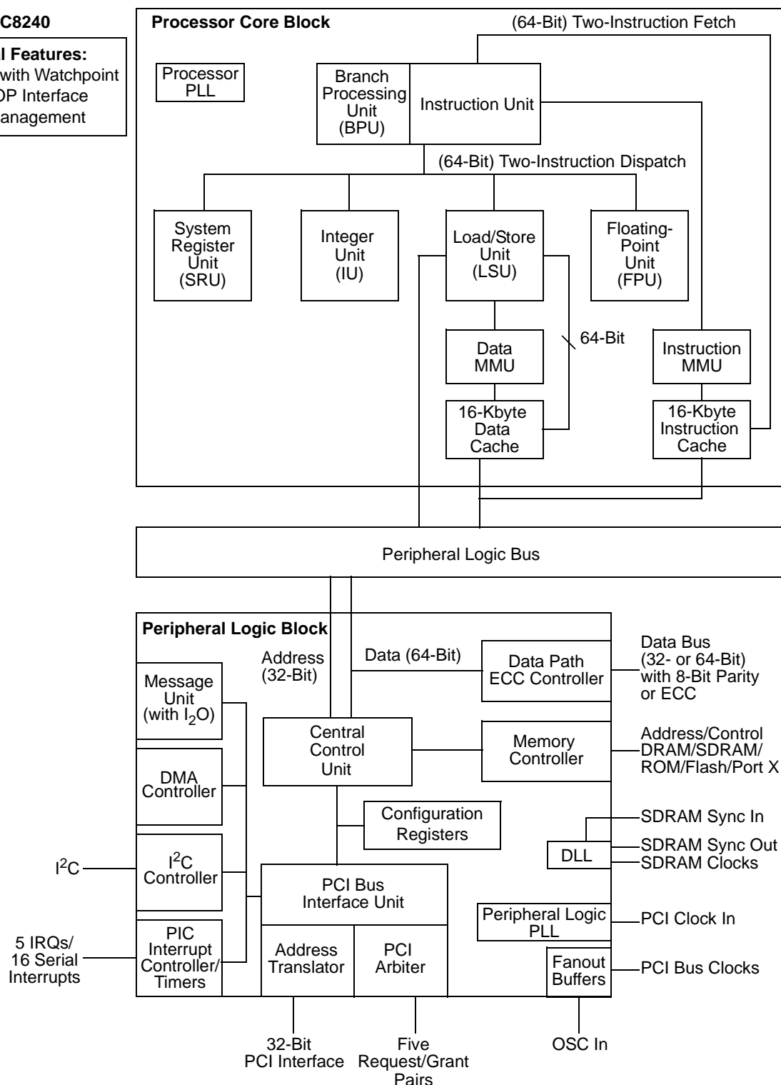
Figure 1. MPC8240 Block Diagram
