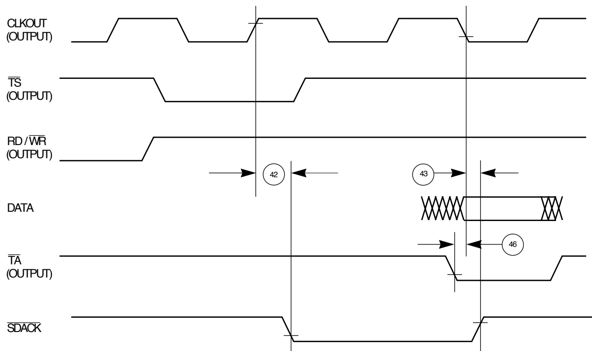
Figure 39. \overline{\text{SDACK}} Timing Diagram—Peripheral Write, \overline{\text{TA}} Sampled Low at the Falling Edge of the Clock
