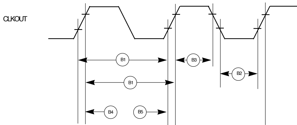
Figure 1. External Clock Timing Diagram
