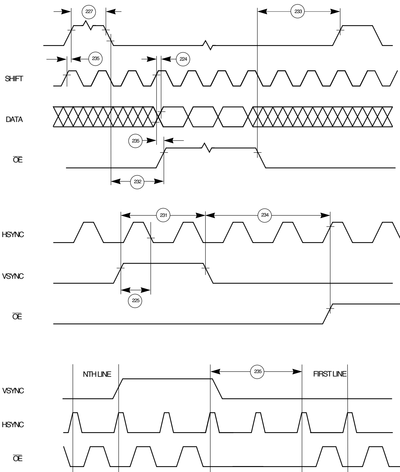
Figure 59. TFT Panel Timing Diagram
