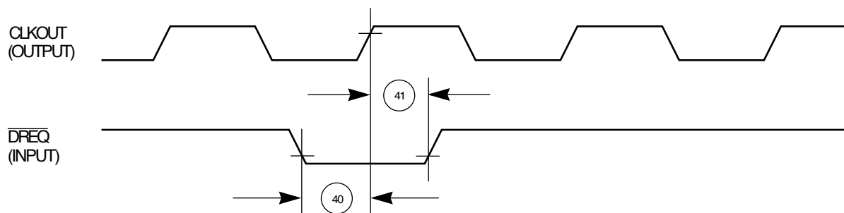
Figure 38. IDMA External Requests Timing Diagram
