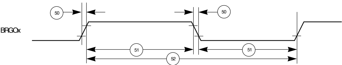
Figure 42. Baud Rate Generator Timing Diagram
