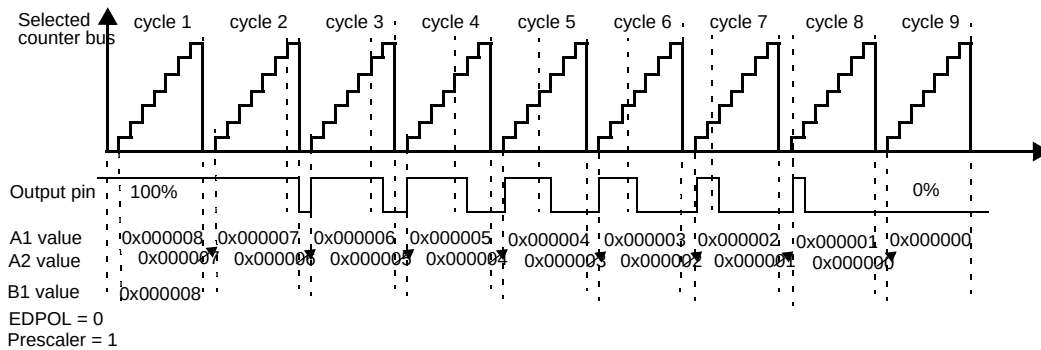
Figure 17-33. OPWMB Mode from 100% to 0% Duty Cycle
