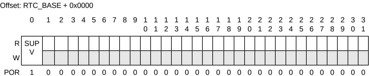
Figure 36-3. RTC Supervisor Control Register (RTCSUPV)
