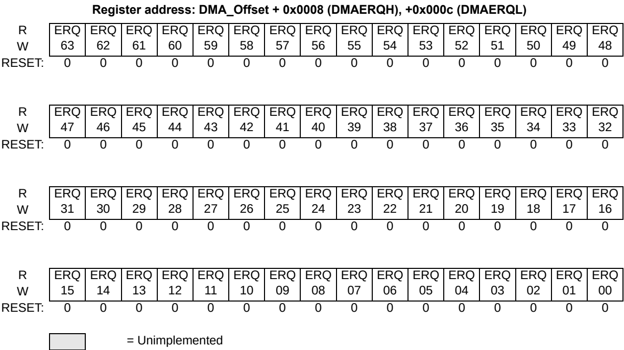
Figure 2. eDMA Enable Request (DMAERQH, DMAERQL) Registers
