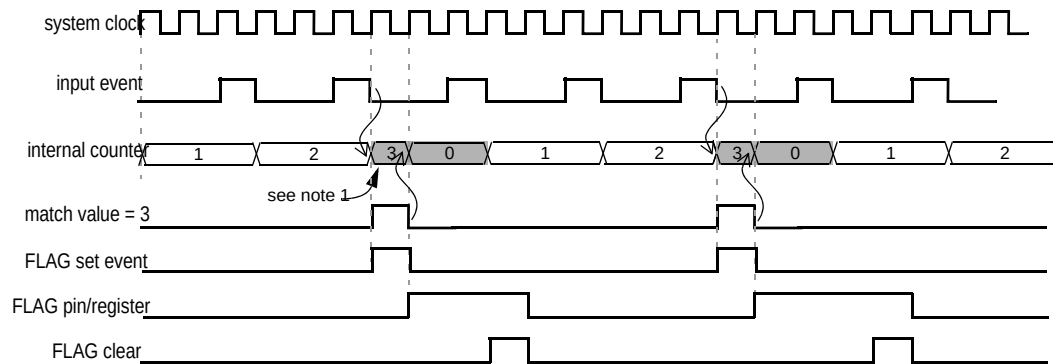
Figure 17-39. Time base generation with external clock and clear on match start
