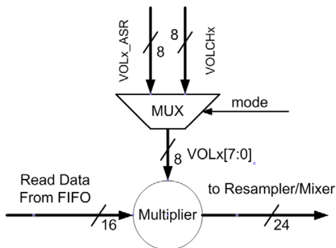
Figure 39-46. Volume Controller for One Channel
