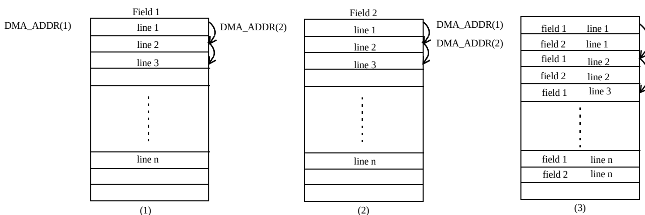
Figure 47-21. Implementation of De-interlace
