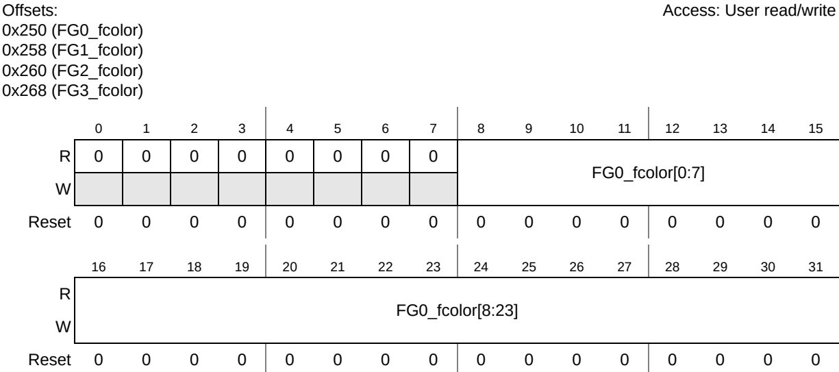
Figure 12-46. FG0_fcolor Register
