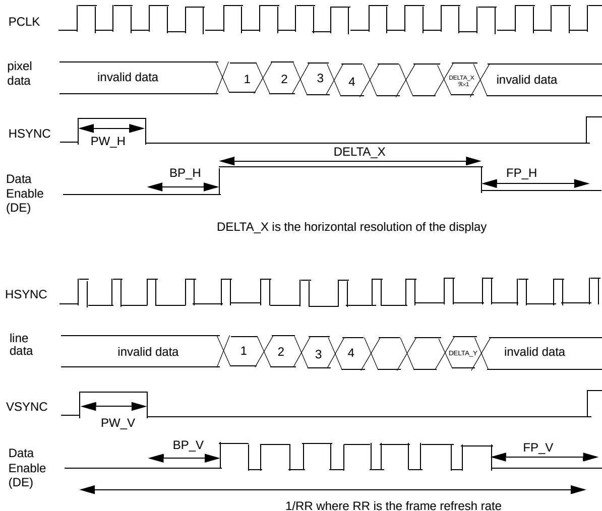
Figure 12-62. HSYNC and VSYNC timing diagram
