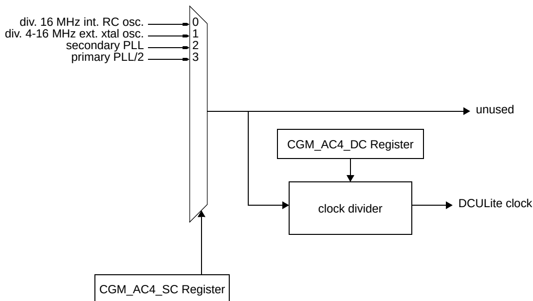
Figure 8-23. MC_CGM Auxiliary Clock 4 Generation Overview
