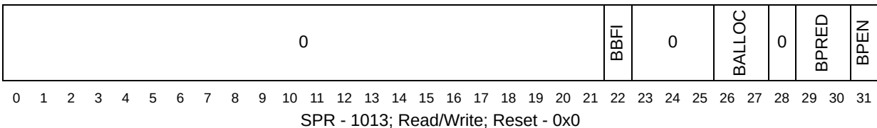
Figure 50-1. Branch Unit Control and Status Register (BUCSR)
