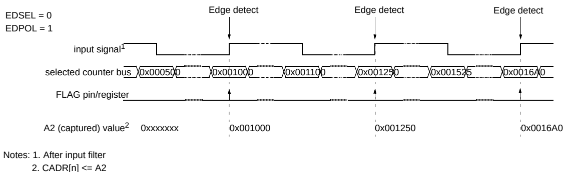
Figure 17-17. Single Action Input Capture with rising edge triggering example
