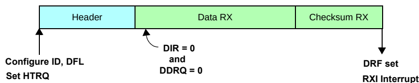
Figure 27-58. Programming consideration: master node, receiver
