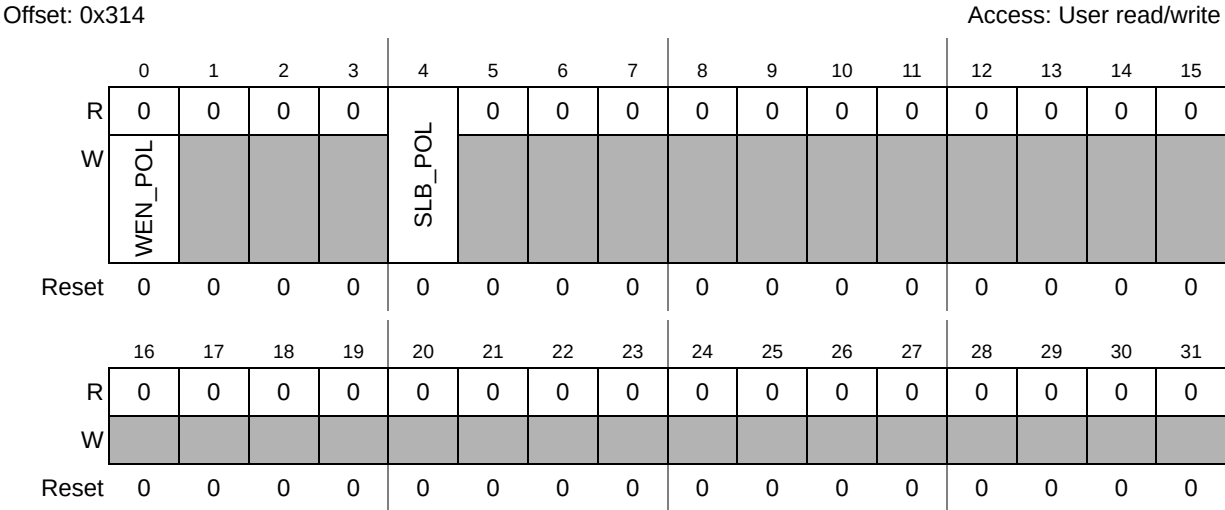
Figure 11-60. Soft Lock POL Register
