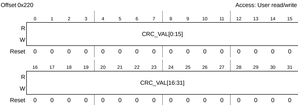
Figure 12-35. CRC_VAL register
