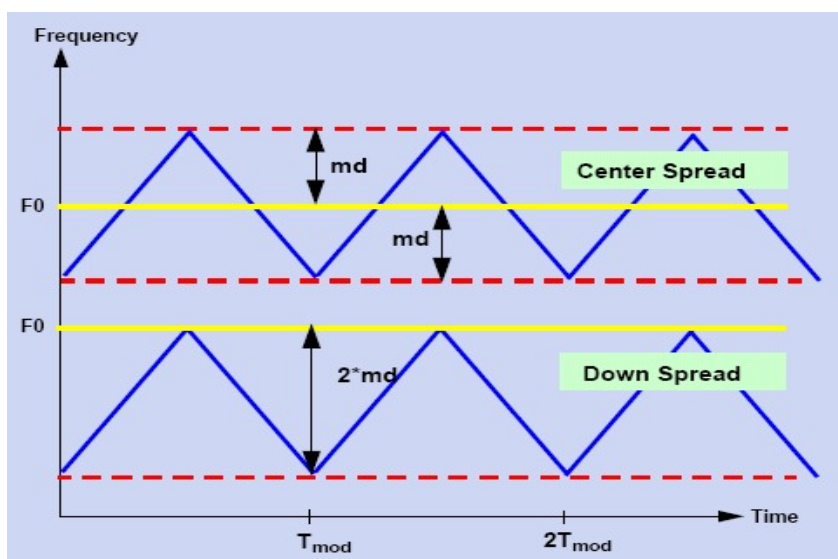
Figure 8-31. PLL frequency modulation modes
