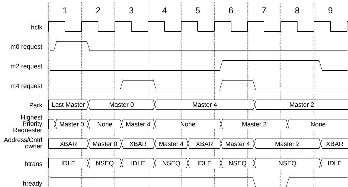
Figure 9-12. Parking on last master
