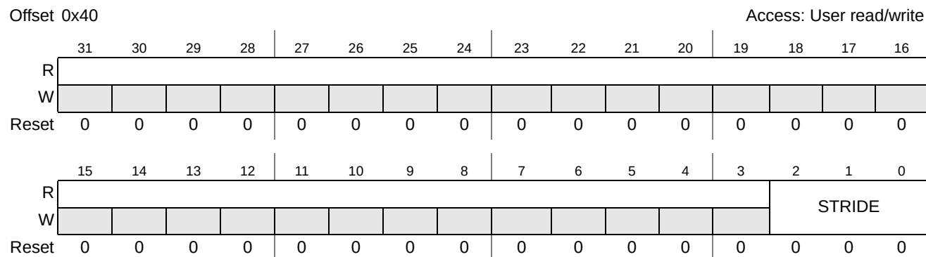
Figure 22-6. GFX2D Stride Setting (GXGSTRIDE)
