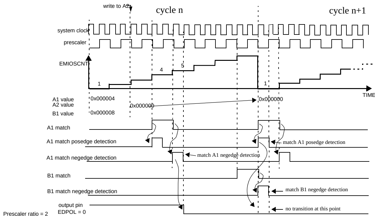
Figure 17-26. OPWFMB Mode with A1 = 0 (0% duty cycle)
