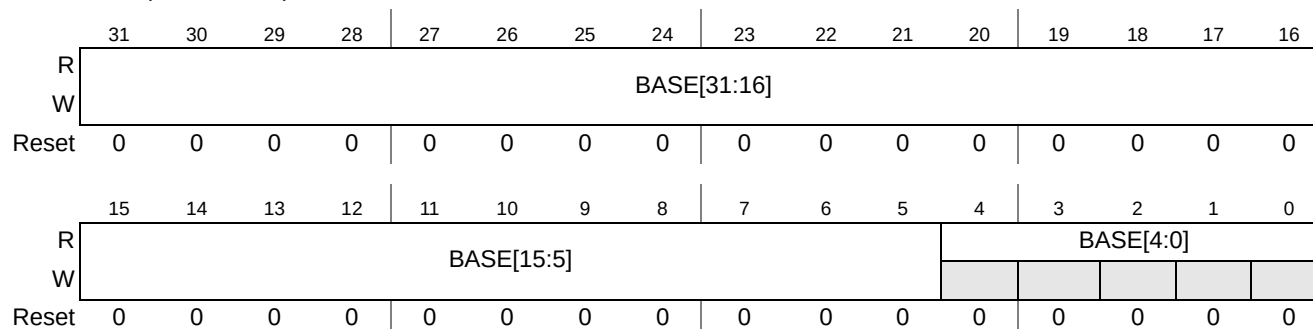
Figure 22-3. Window Destination Base Address (GXGBASE0-3)
