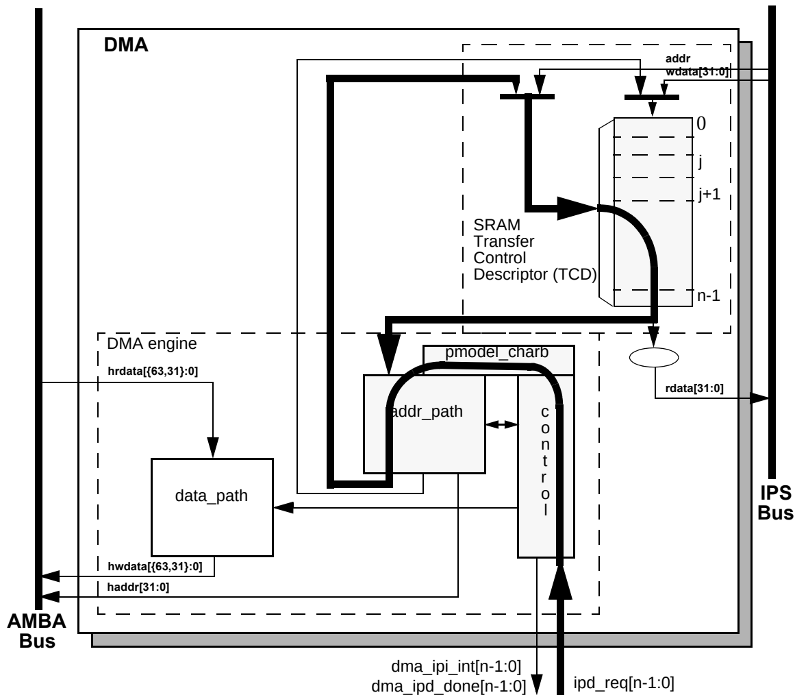
Figure 18-28. eDMA operation, part 1
