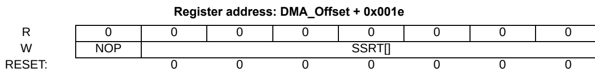
Figure 10. eDMA Set START Bit (DMASSRT) Register
