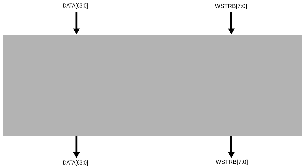
Figure 22-9. Word-wide Swap
