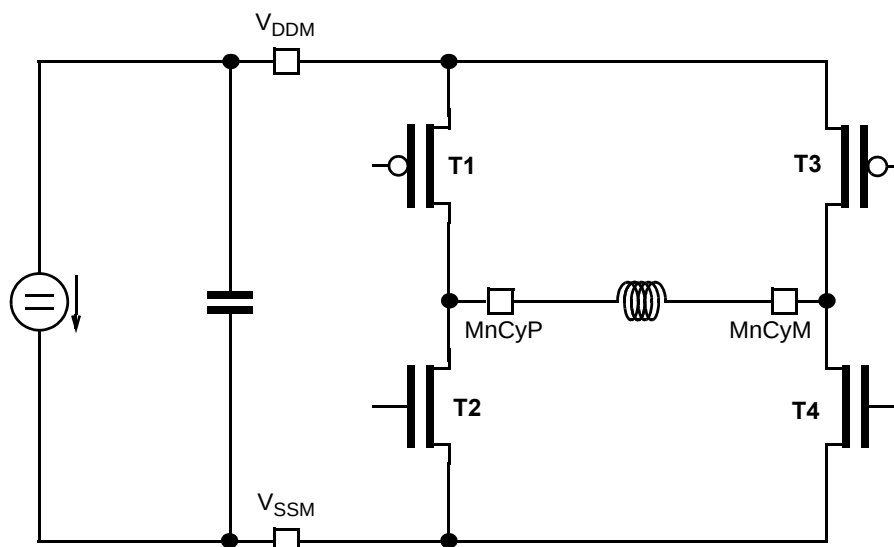
Figure 41-26. Output Transistor Assignment
