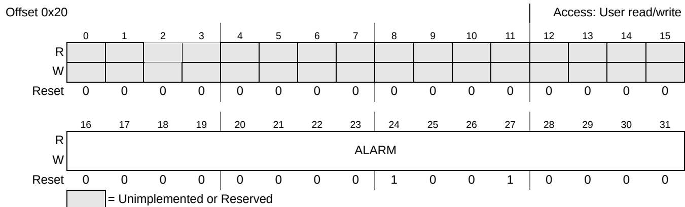
Figure 47-10. HPALRM Register
