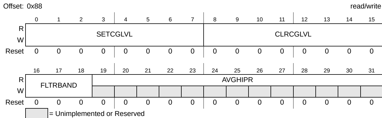
Figure 14-5. HPCFG register
