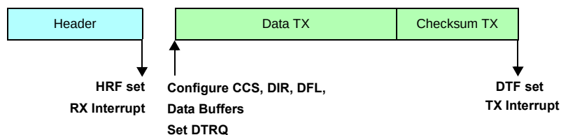
Figure 27-61. Programming consideration: slave node, transmitter, no filters
