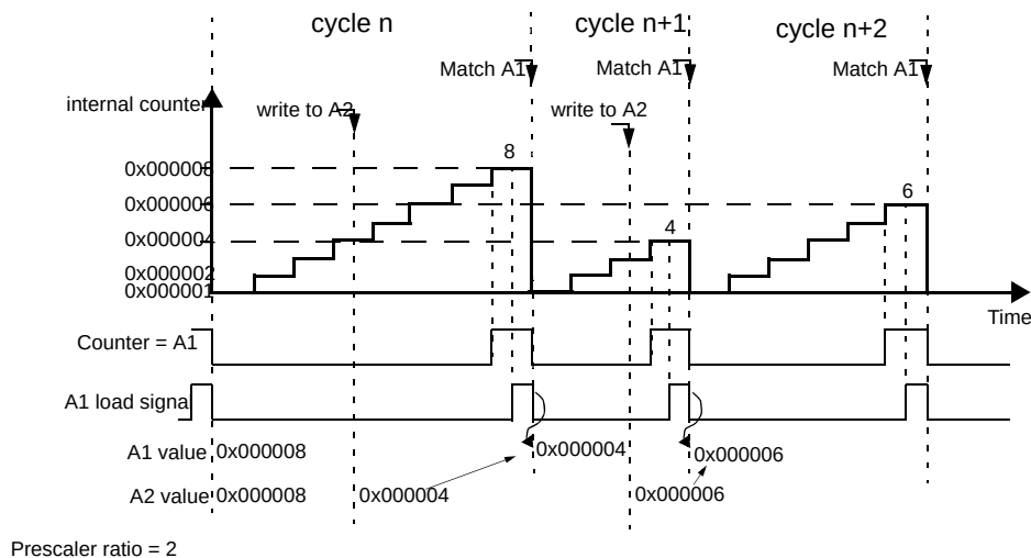
Figure 17-23. MCB Mode A1 Register Update in Up Counter Mode
