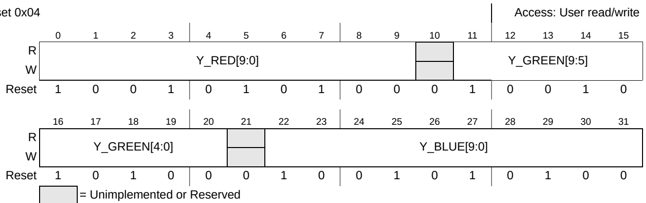
Figure 47-3. LUMA_COMP Register
