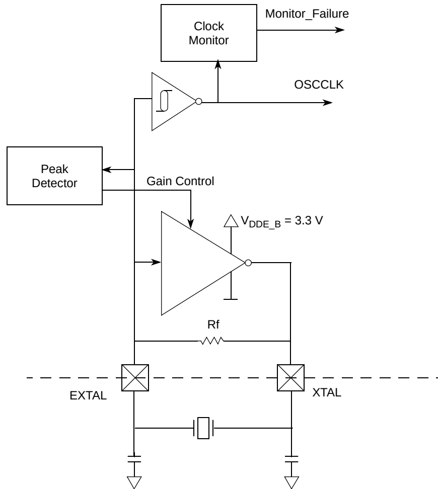
Figure 8-25. FXOSC block diagram
