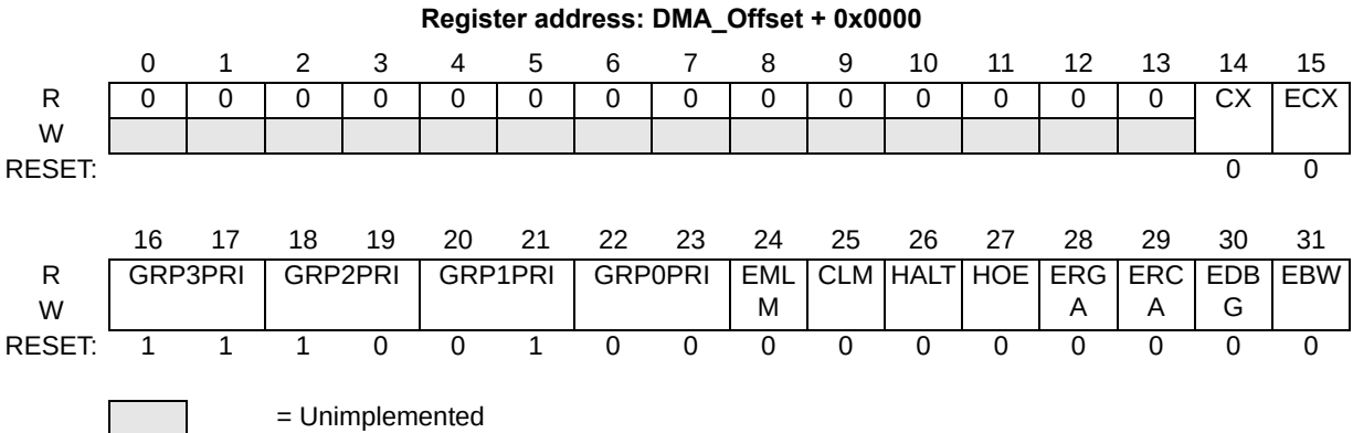
Figure 18-2. DMA Control Register (DMACR)
