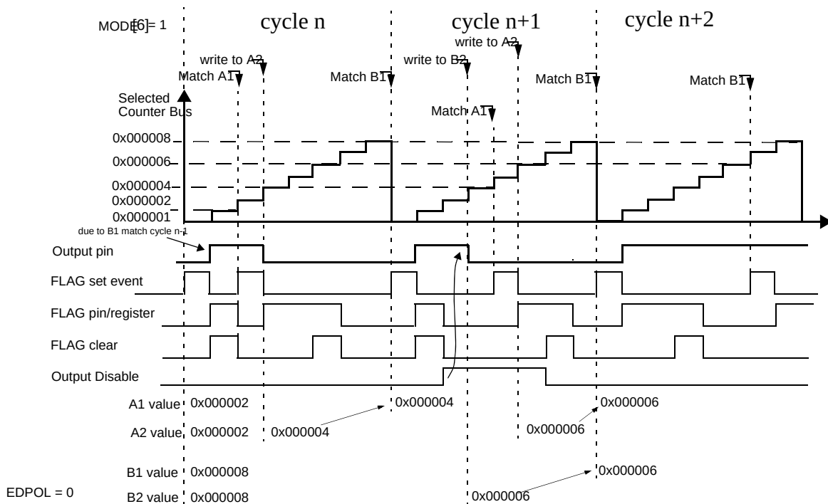
Figure 17-32. OPWMB Mode with Active Output Disable
