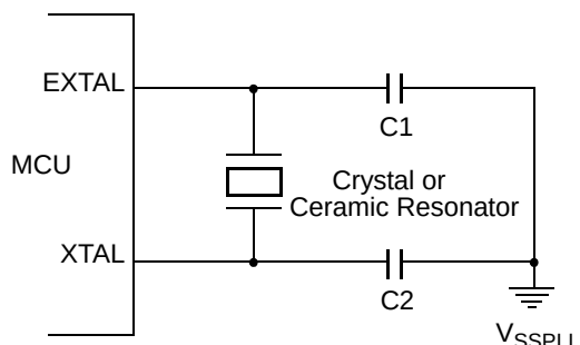
Figure 8-26. Loop controlled Pierce oscillator connections (LCP mode selected)
