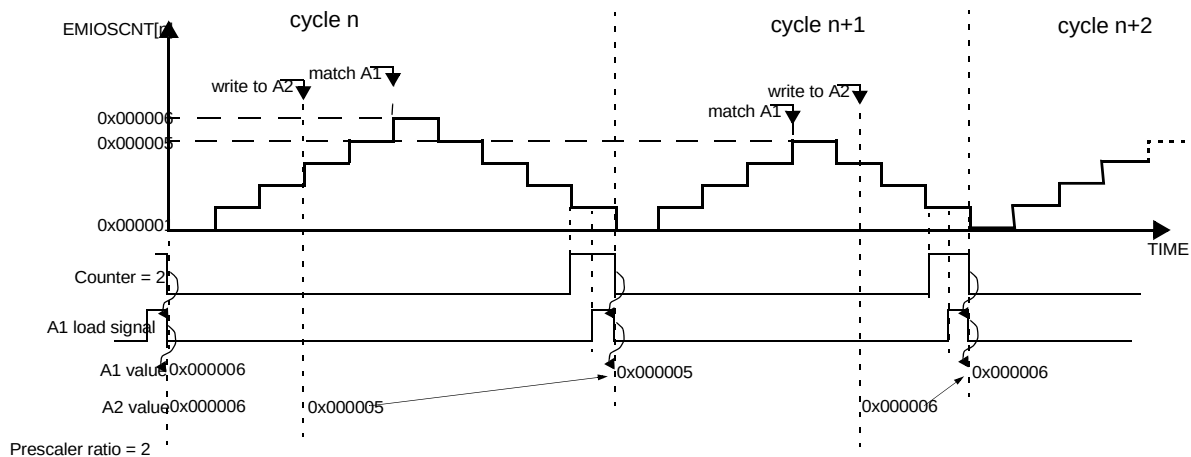
Figure 17-24. MCB Mode A1 Register Update in Up/Down Counter Mode
