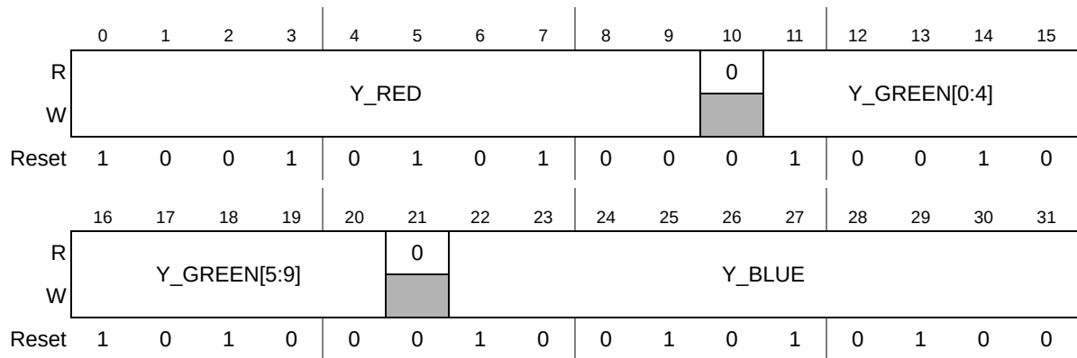
Figure 12-49. Layer LUMA Component Register (LYR_LUMA_COMPONENT)
