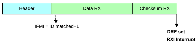
Figure 27-66. Programming consideration: slave node, at least one RX filter, BF is reset, ID matches filter
