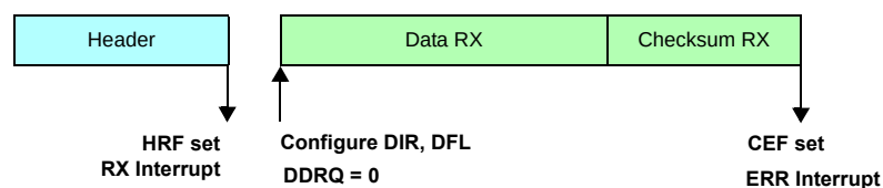
Figure 27-64. Programming consideration: slave node, receiver, no filters, checksum error
