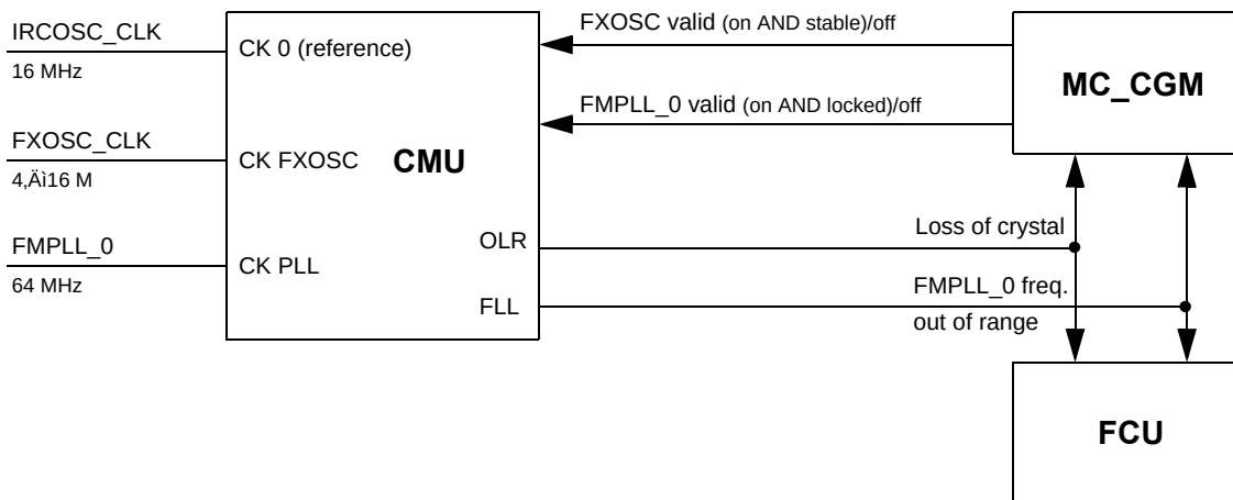
Figure 8-32. CMU component interaction
