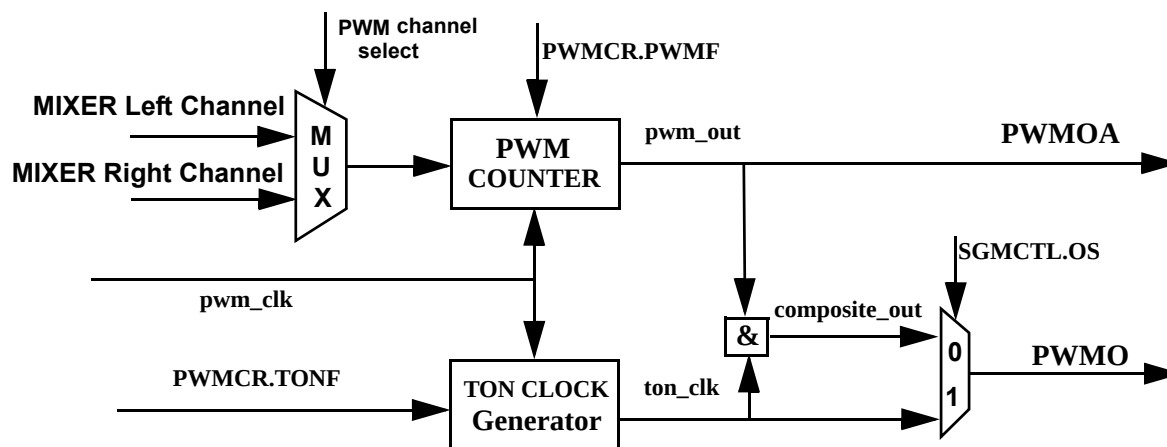
Figure 39-59. PWM Block
