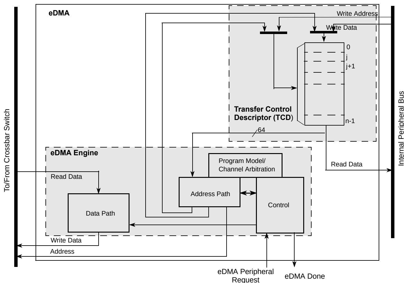
Figure 18-1. DMA block diagram
