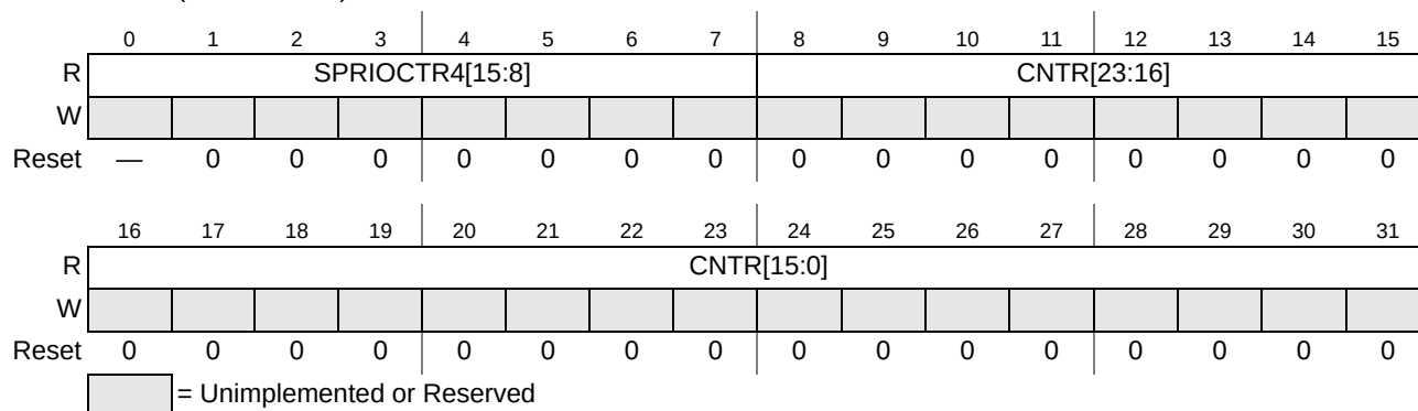
Figure 14-25. Cumulative Wait Counter 2 (CUMWCTR2)
