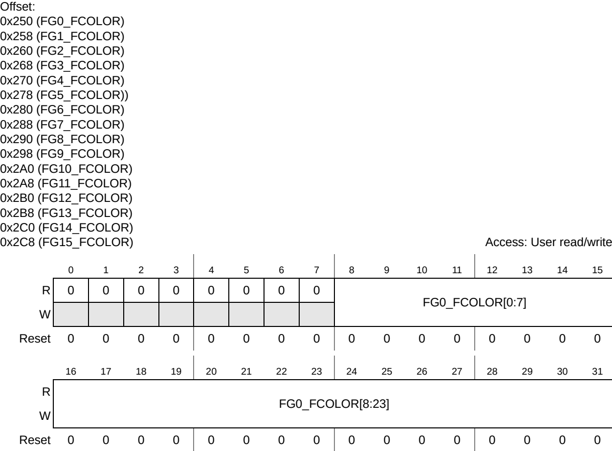
Figure 11-47. FG0_fcolor Register
