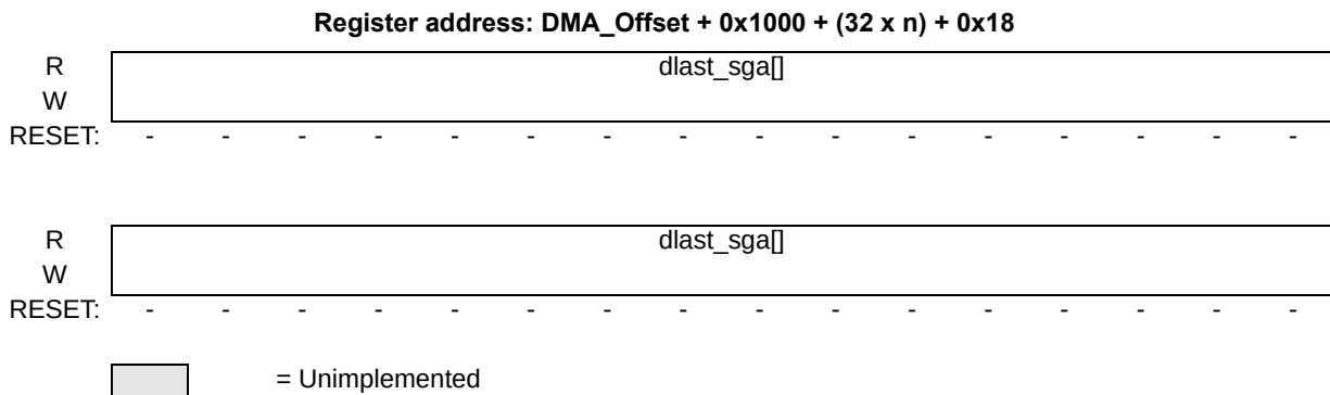
Figure 24. TCDn Word 6 (TCDn.dlast_sga) field
