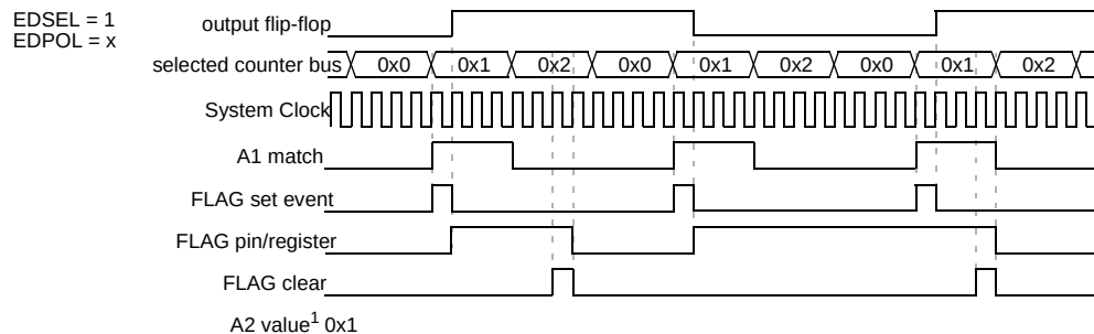
Figure 17-20. SAOC example toggling the output flip-flop
