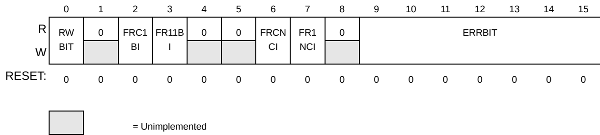
Figure 19-4. ECC Error Generation (EEGR) Register
