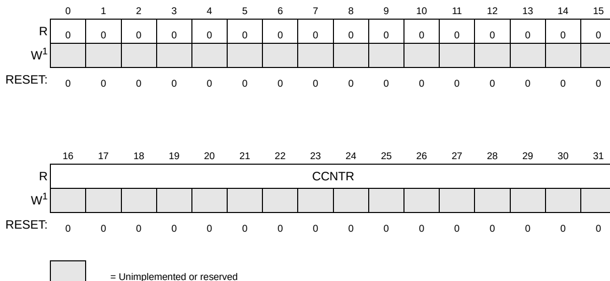
Figure 17-10. eMIO200 UC Counter Register (CCNTR[n])
