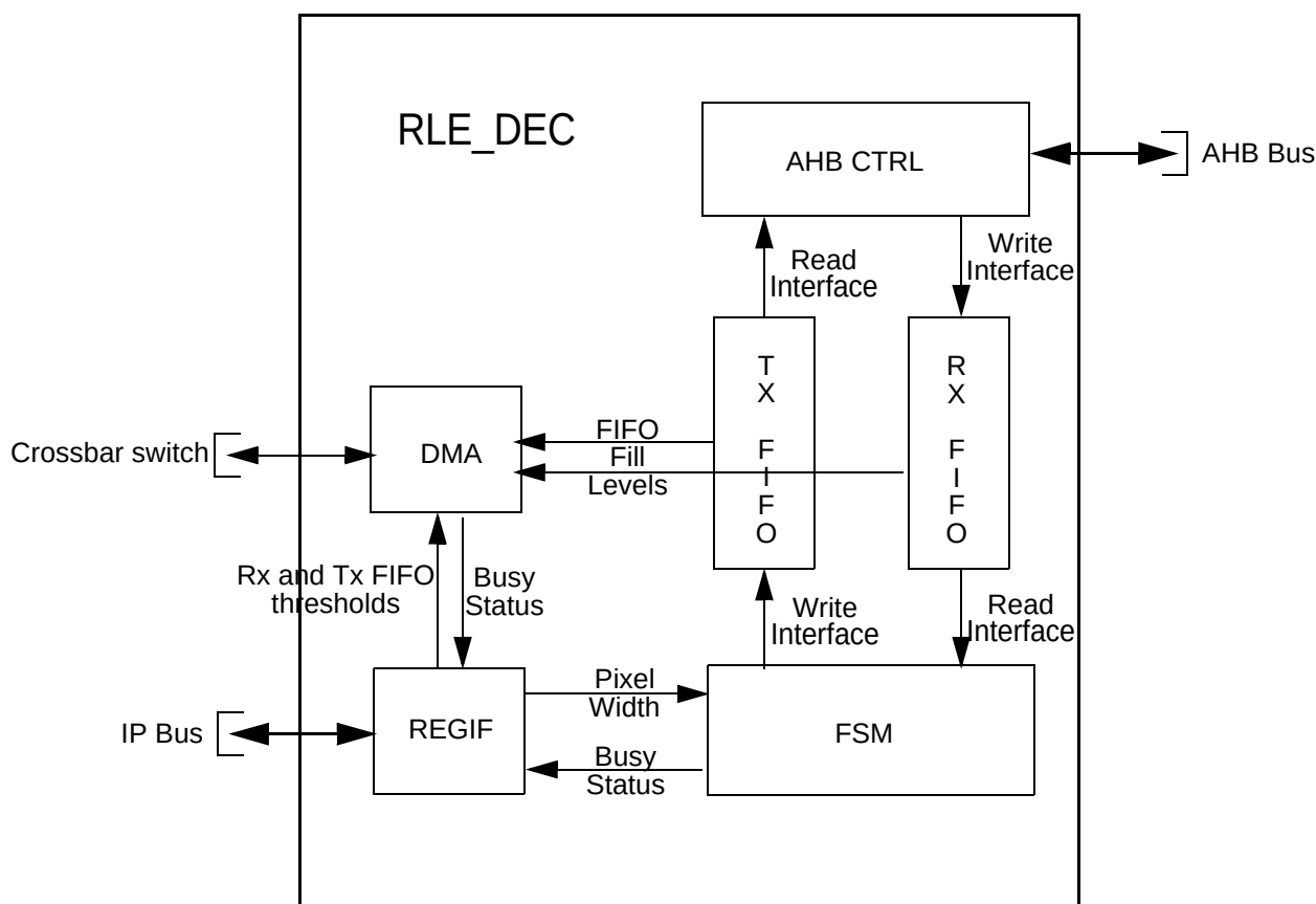
Figure 38-1. RLE_DEC block diagram
