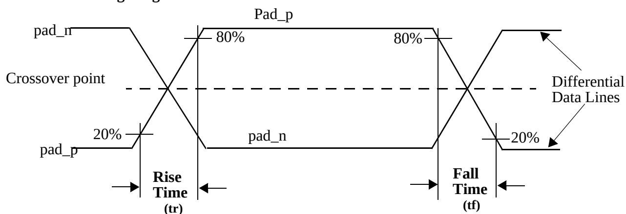
Figure 46-17. Rise/Fall Transition
