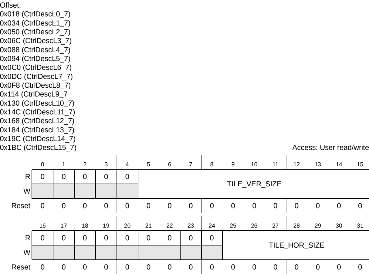
Figure 11-10. Control Descriptor L0_7 Register
