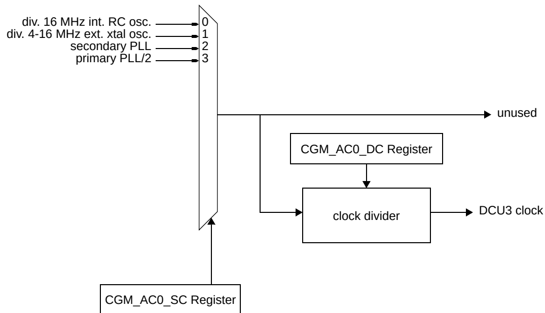
Figure 8-19. MC_CGM auxiliary clock 0 generation overview
