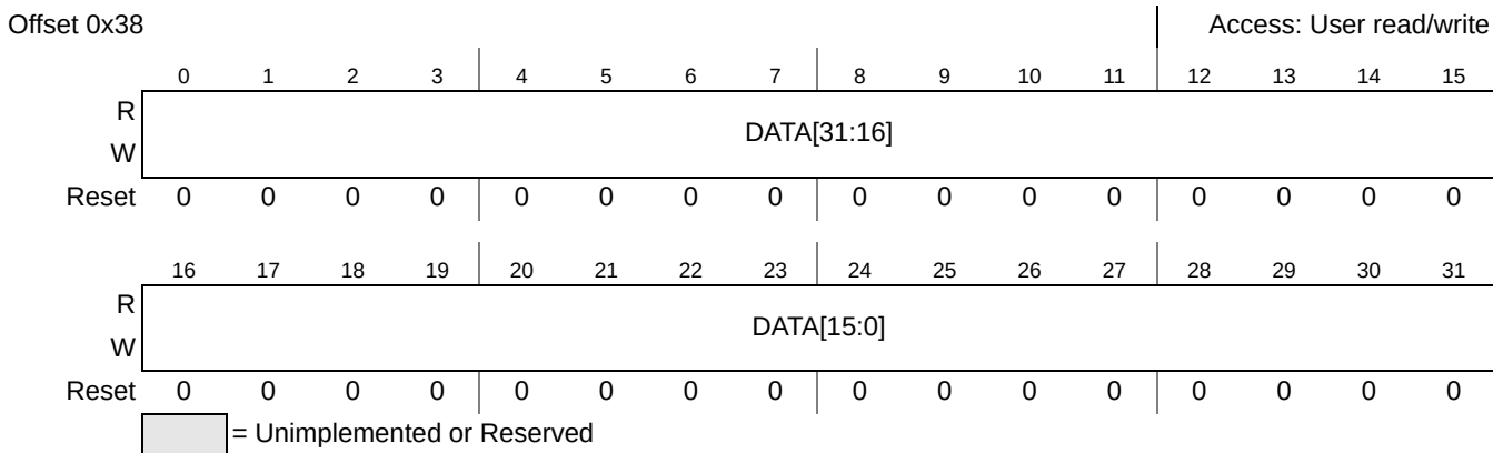
Figure 47-16. LUT_DATA Register
