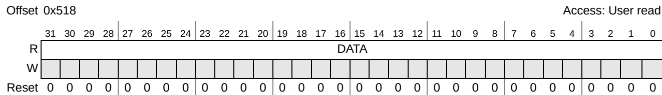
Figure 31-11. MMU Read Data (MMU_READ_DATA)
