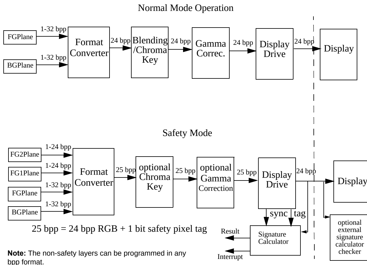
Figure 11-85. Safety Mode block diagram
