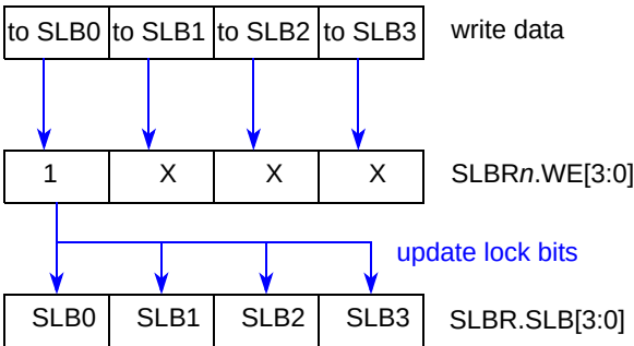
Figure 4-8. Change Lock Settings for 32-bit Protected Addresses
