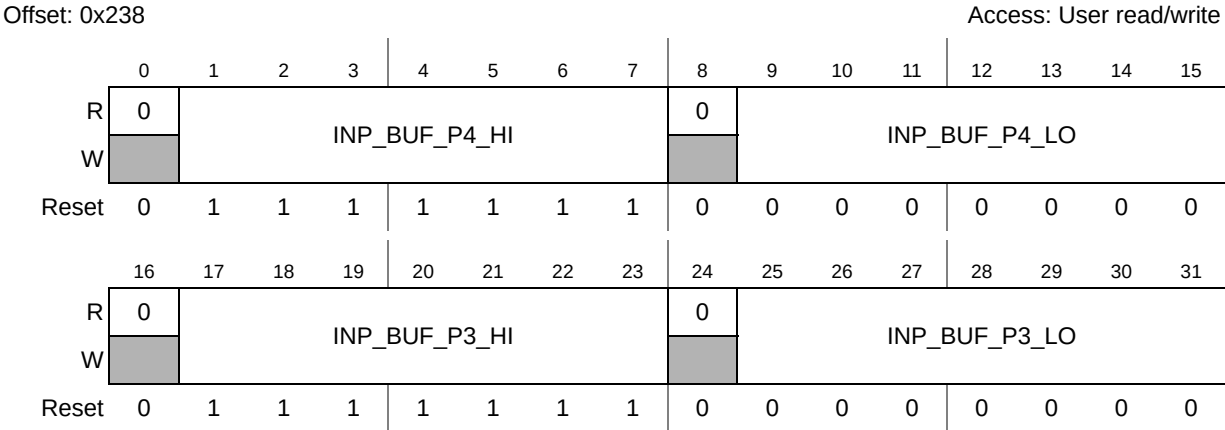
Figure 11-41. THRESHOLD_INP_BUF_2 Register
