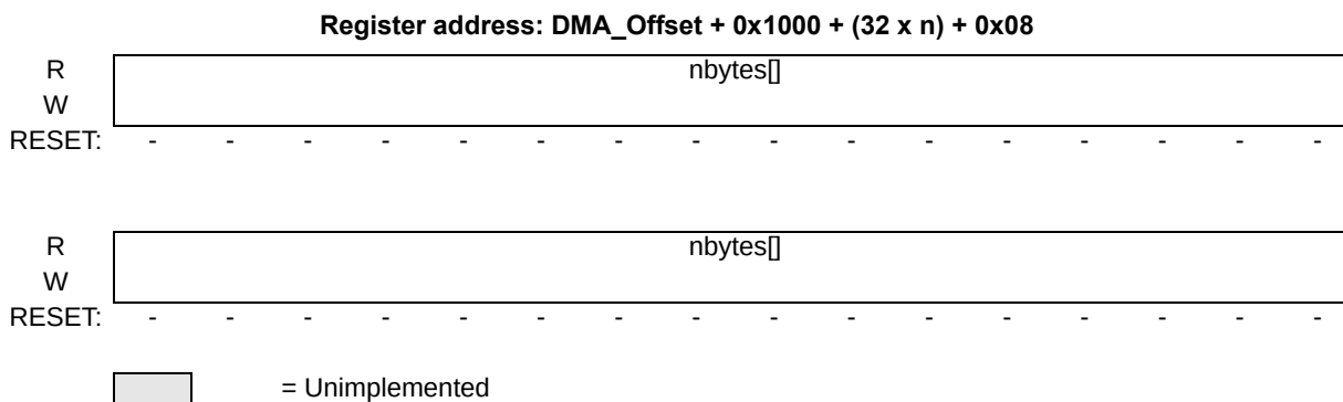
Figure 19. TCDn Word 2 (TCDn.nbytes) field
