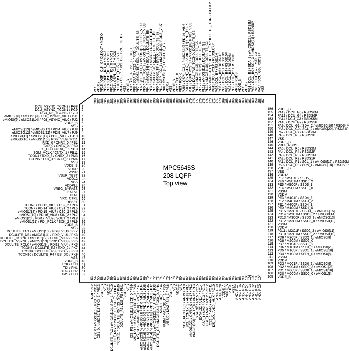
Figure 3-2. 208-pin LQFP pinout
