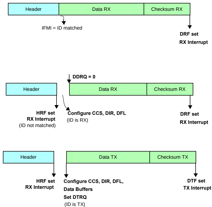
Figure 27-69. Programming consideration: slave node, RX filter, BF is set
