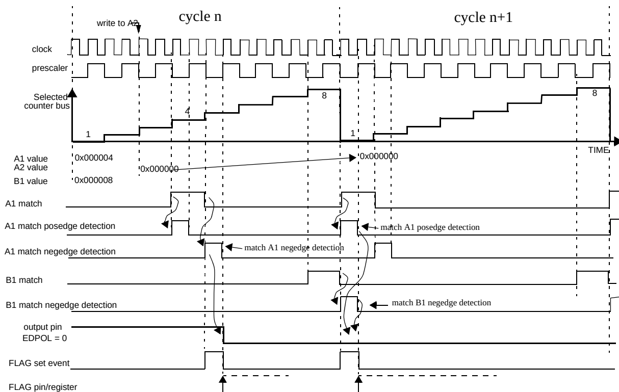
Figure 17-31. OPWMB Mode with 0% Duty Cycle
