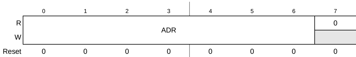
Figure 25-3. I 2 C Bus Address Register (IBAD)
