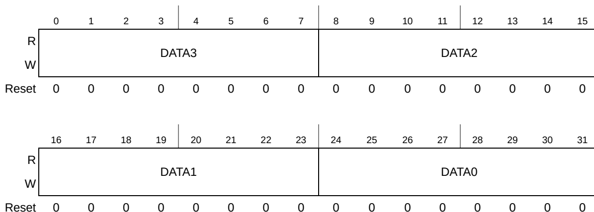
Figure 27-32. Buffer data register least significant (BDRL)
