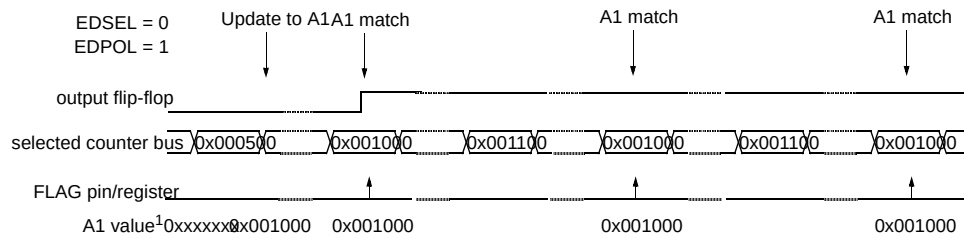
Figure 17-19. SAOC example with EDPOL value being transferred to the output flip-flop
