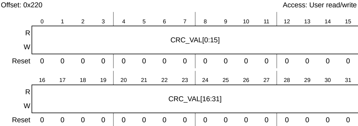
Figure 11-35. CRC_VAL Register
