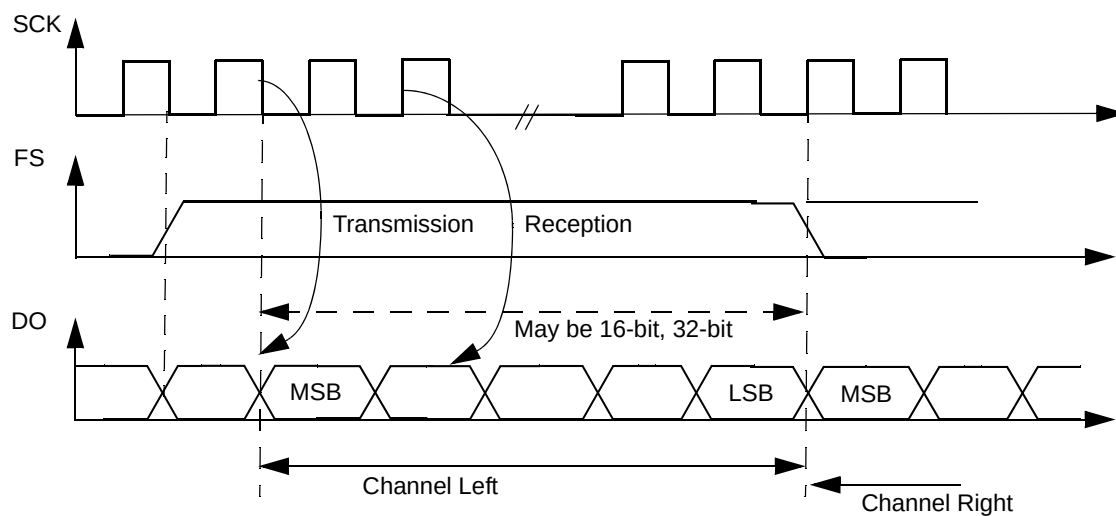
Figure 39-51. 16/32 bit
