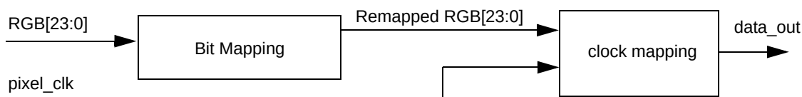
Figure 46-14. Bit mapping control
