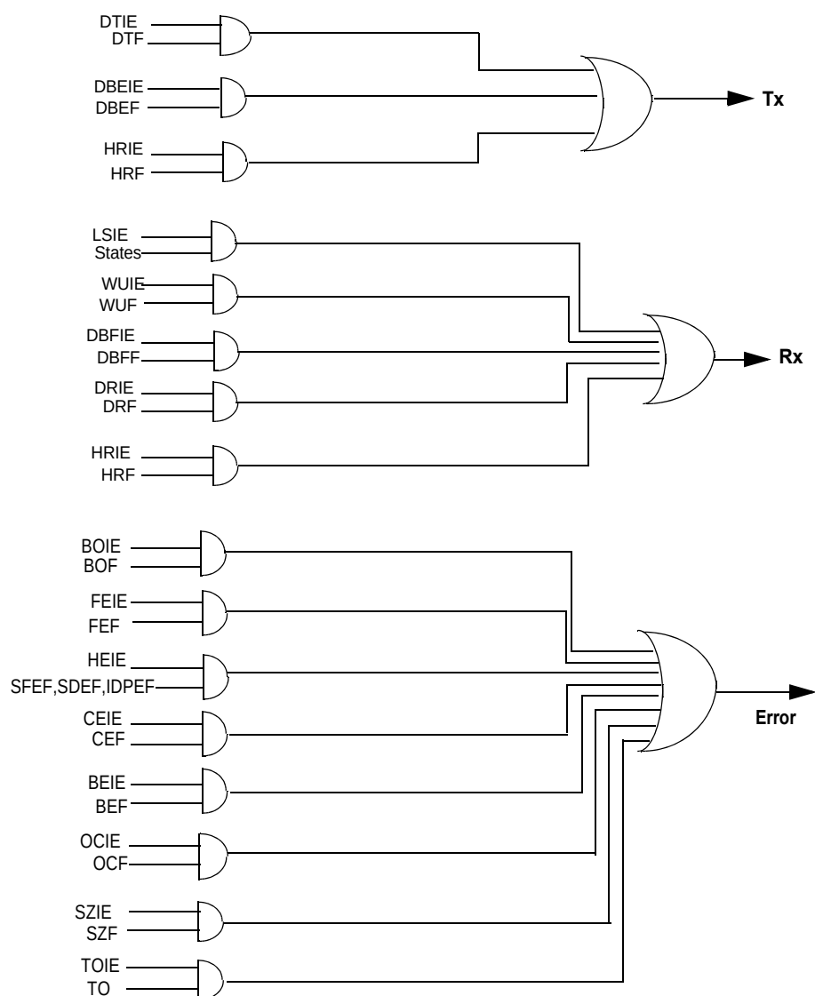
Figure 27-56. Interrupt diagram
