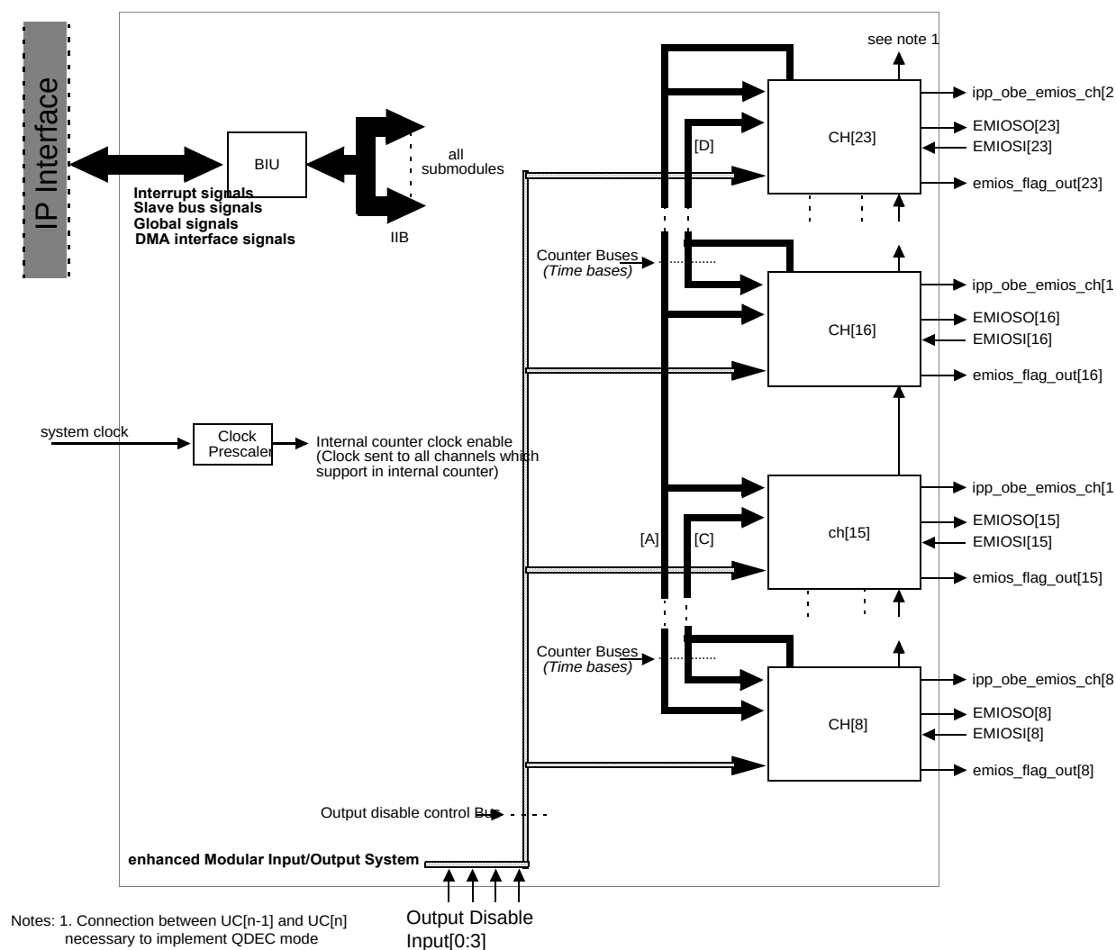
Figure 17-1. eMIOS200 block diagram
