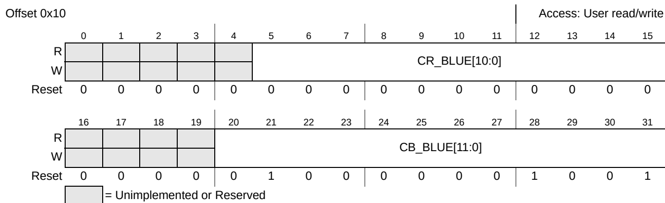
Figure 47-6. CHROMA_BLUE Register
