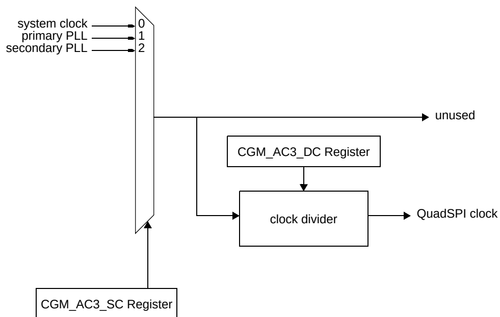
Figure 8-22. MC_CGM Auxiliary Clock 3 Generation Overview
