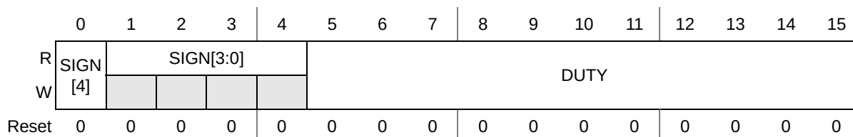
Figure 41-6. Motor Controller Duty Cycle Register (MCDC0..11)
