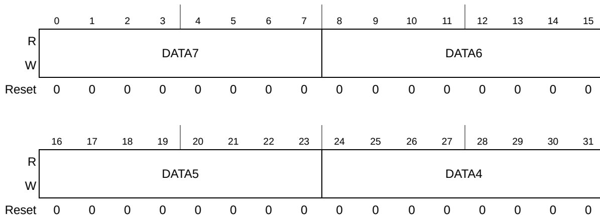
Figure 27-33. Buffer data register most significant (BDRM)
