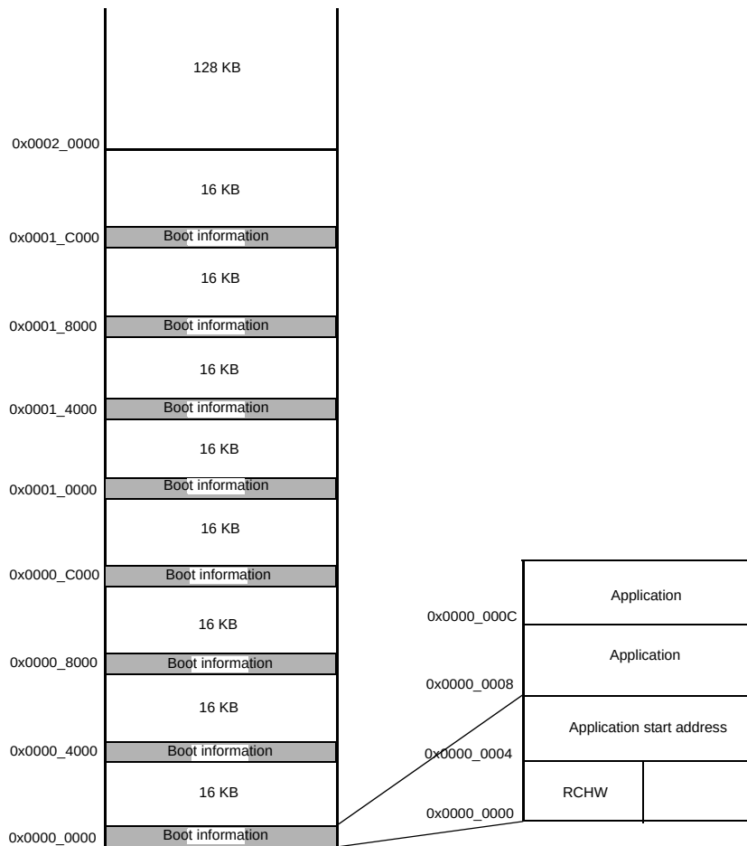
Figure 6-3. MPC5645S flash memory partitioning and RCHW search
