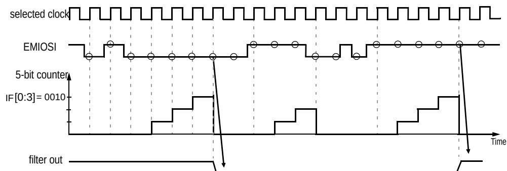
Figure 17-37. Input Programmable Filter Example
