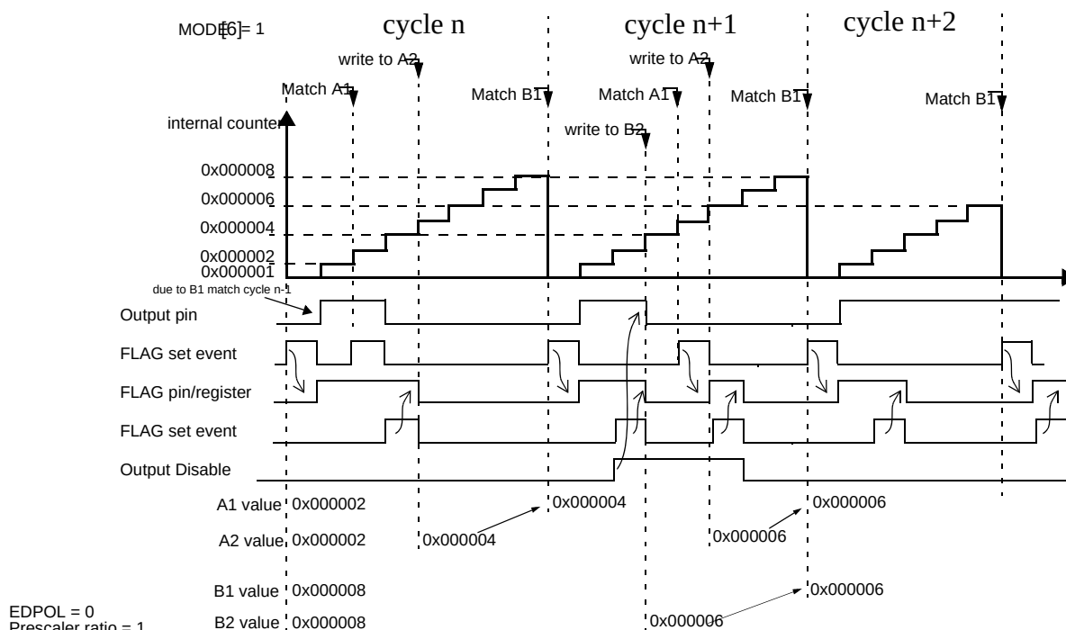
Figure 17-28. OPWFMB Mode with Active Output Disable
