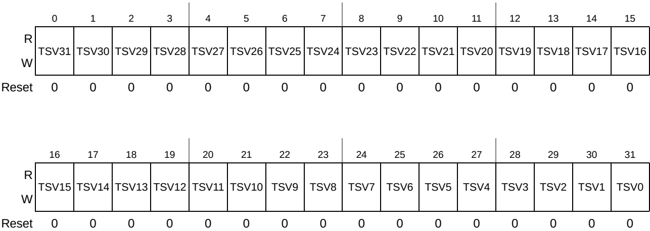
Figure 32-3. Timer Load Value Register (LDVAL)
