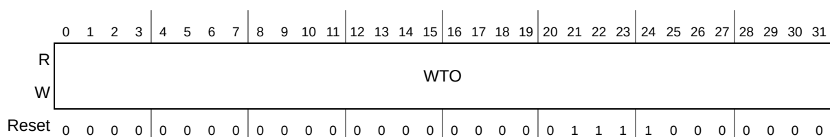
Figure 4-15. SWT Time-Out Register (SWT_TO)
