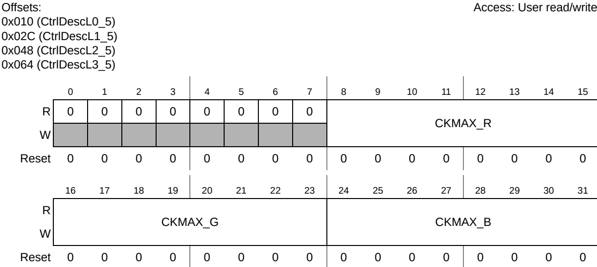
Figure 12-8. CtrlDescL0_5 Register
