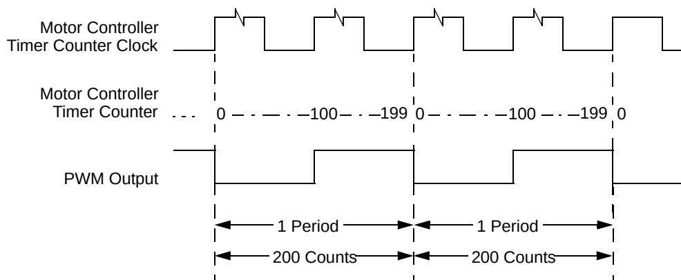
Figure 41-27. PWM Output: MCCTL0[DITH] = 0, MCCCx[MCAM] = 0x1, MCDCCx[DUTY] = 100, MCPER[PER] = 200, MCCTL1[RECIRC] = 0
