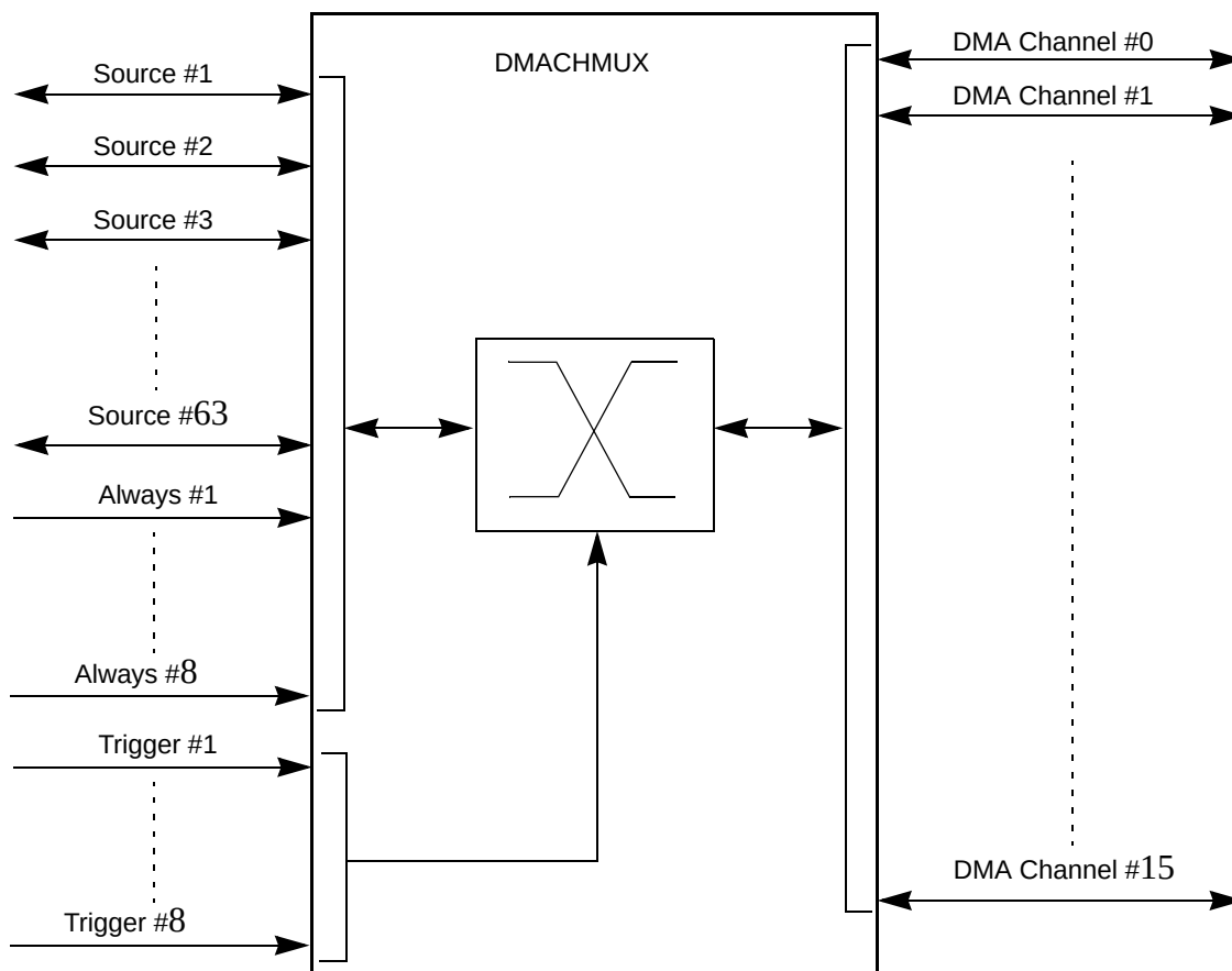
Figure 16-1. DMACHMUX block diagram
