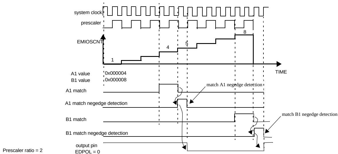
Figure 17-25. OPWFMB A1 and B1 match to Output Register Delay
