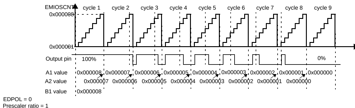
Figure 17-29. OPWFMB Mode from 100% to 0% Duty Cycle
