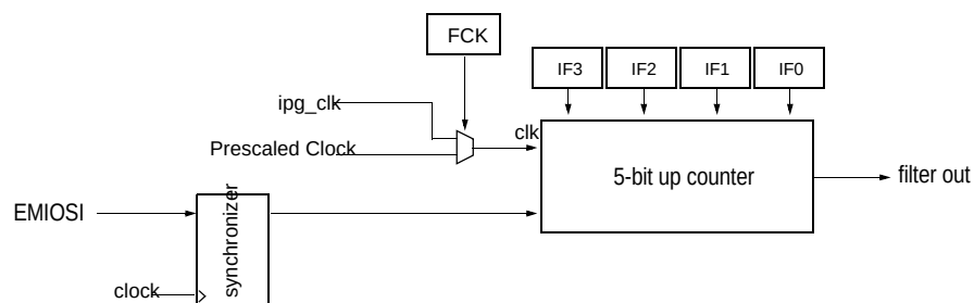
Figure 17-36. Input Programmable Filter Submodule Diagram
