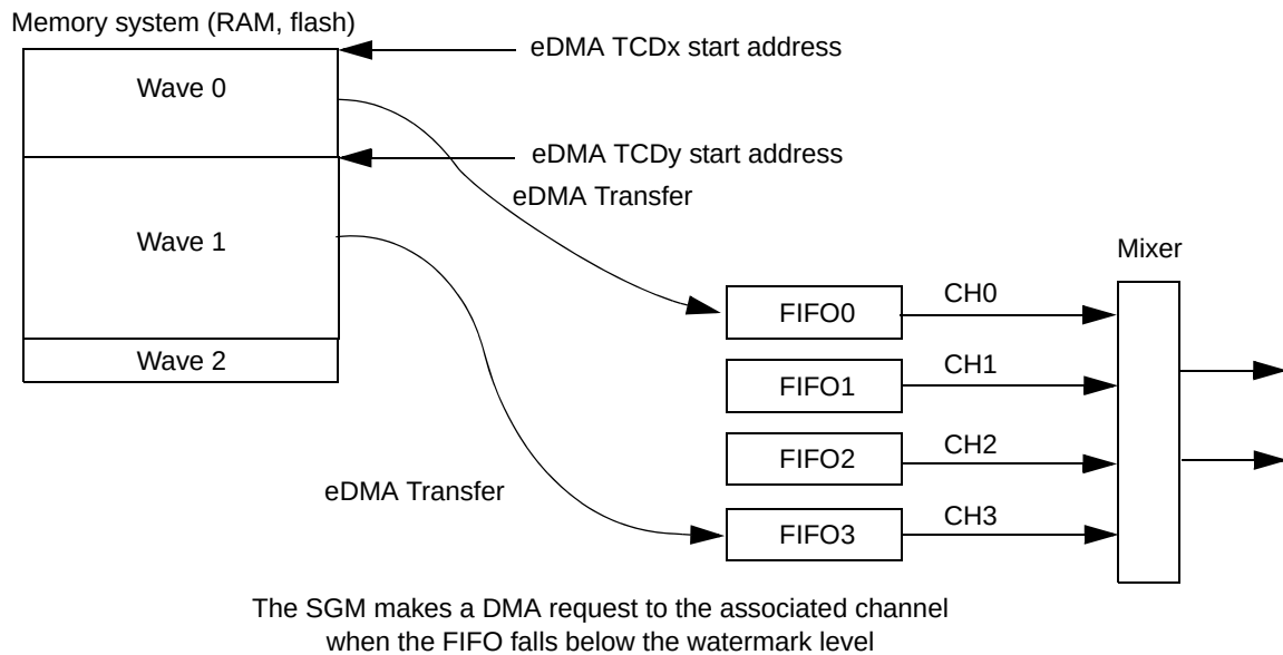
Figure 39-38. PCM Sample Flow for Wave mode
