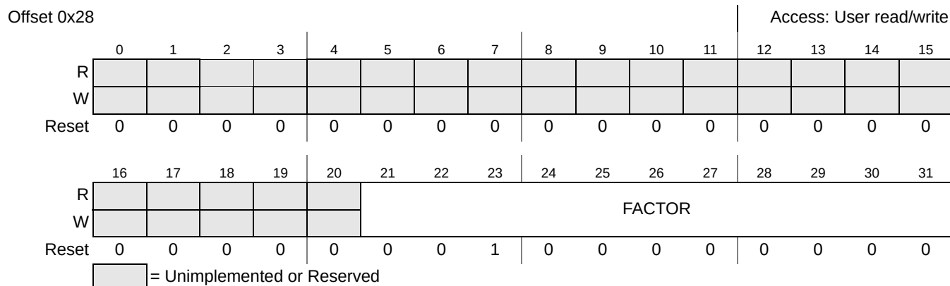
Figure 47-12. FACTOR_H Register
