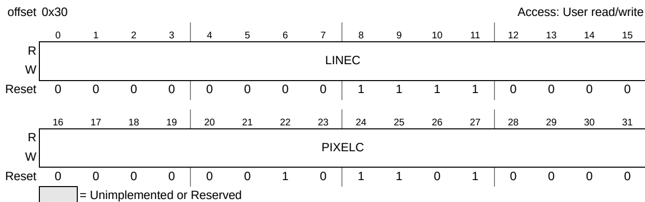
Figure 47-14. VID_SIZE Register
