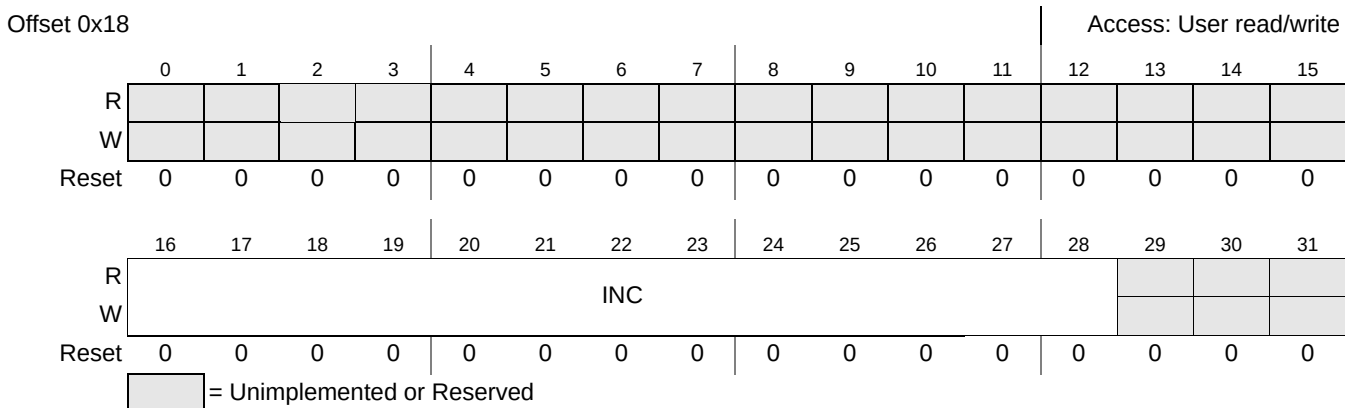
Figure 47-8. DMA_INCREMENT Register
