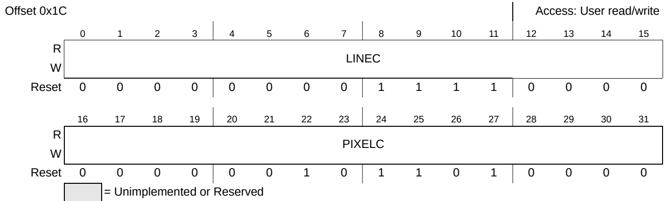
Figure 47-9. INVSZ Register
