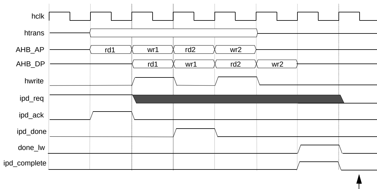
Figure 18-31. ipd_req hardware handshake
