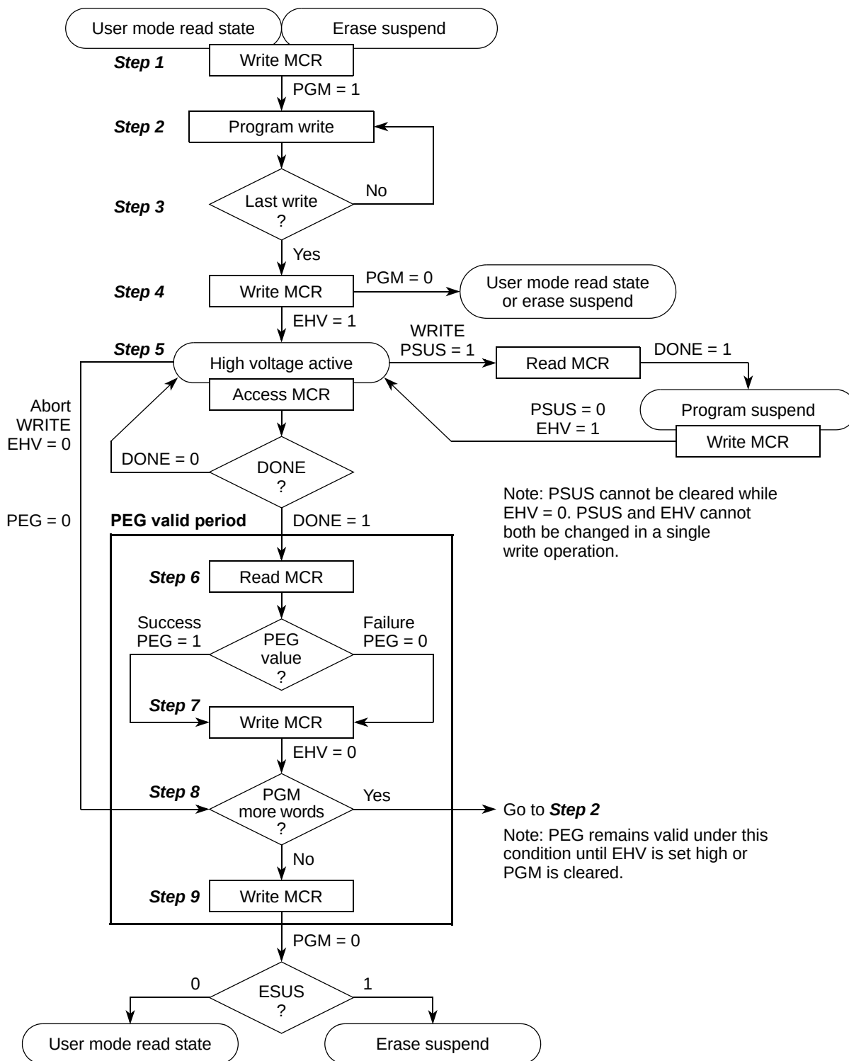
Figure 21-27. Program Sequence
