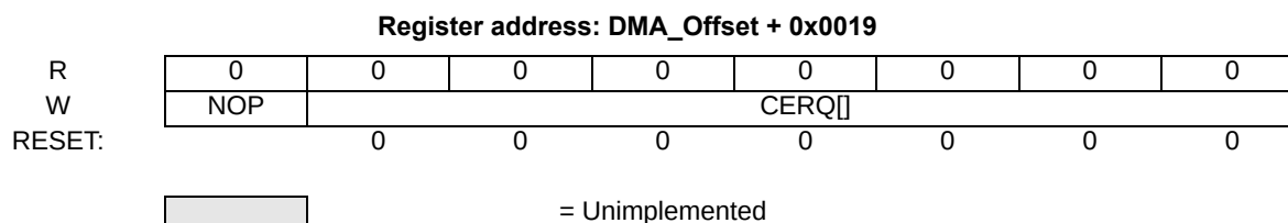
Figure 5. eDMA Clear Enable Request (DMACERQ) Register
