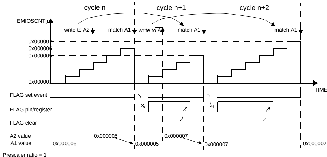
Figure 17-21. Modulus Counter Buffered (MCB) Up Count mode
