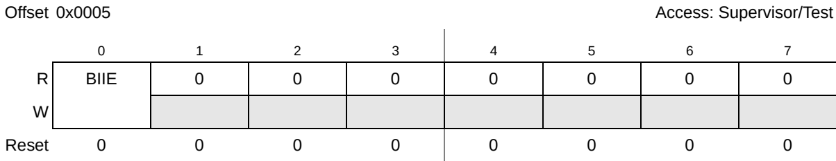
Figure 25-10. I 2 C Bus Interrupt Configuration Register (IBIC)
