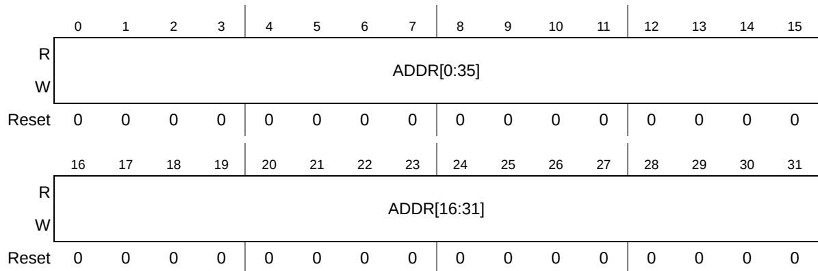
Figure 12-6. CtrlDescL0_3 Register
