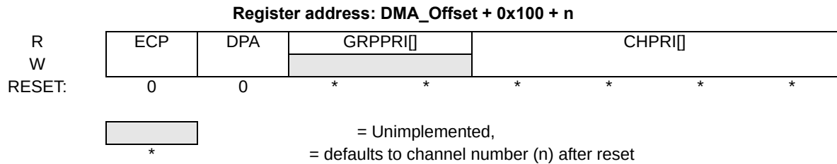
Figure 15. eDMA Channel n Priority (DCHPRIn) Register
