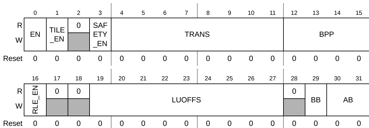
Figure 12-7. CtrlDescL0_4 Register
