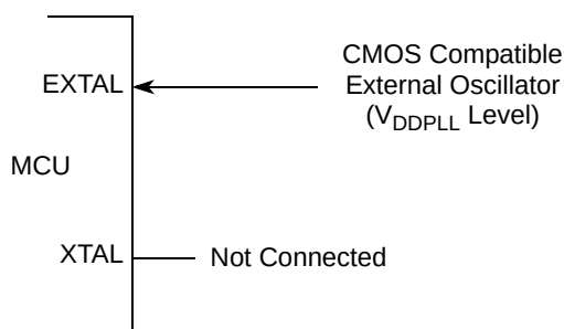
Figure 8-27. External clock connections
