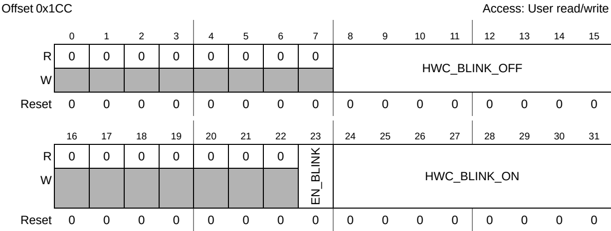
Figure 12-14. Control Descriptor Cursor_4 Register (CtrlDescCursor_4)
