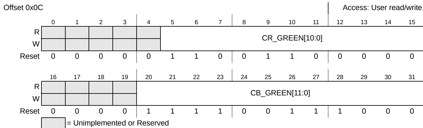
Figure 47-5. CHROMA_GREEN Register
