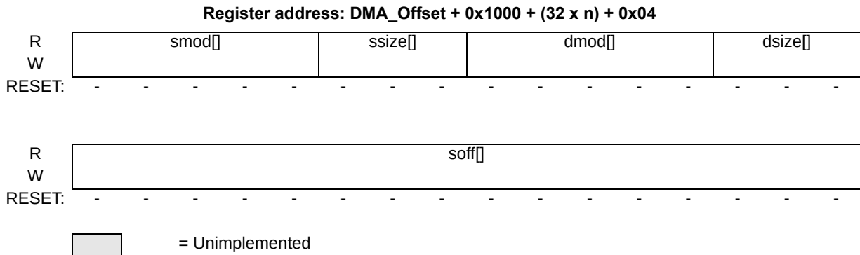
Figure 18. TCDn Word 1 (TCDn.{soff,smod,ssize,dmod,dsize}) fields
