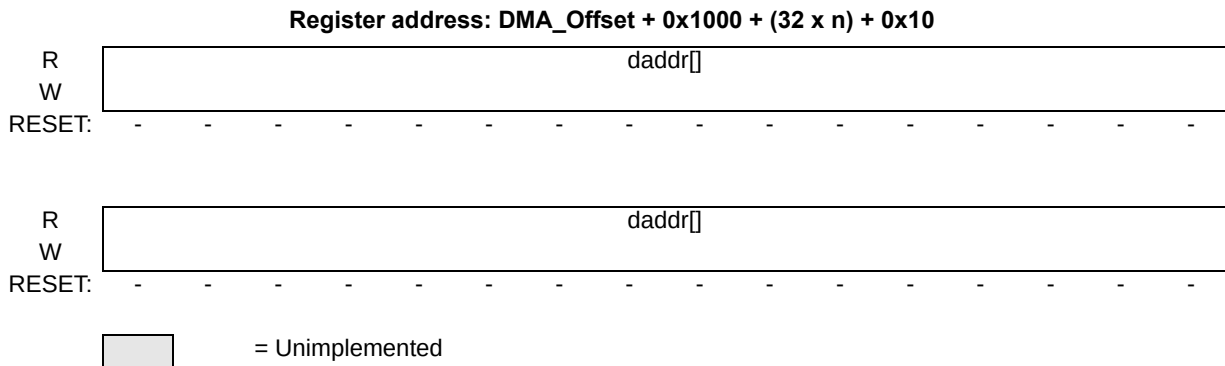
Figure 22. TCDn Word 4 (TCDn.daddr) field
