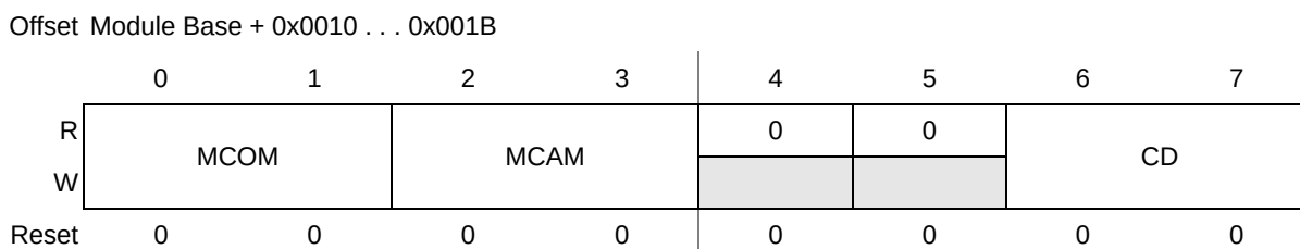
Figure 41-5. Motor Controller Channel Control Register (MCCC0..11)
