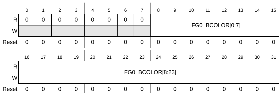
Figure 11-48. FG0_bcolor Register
