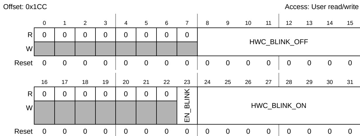
Figure 11-14. Control Descriptor Cursor 4 Register (CtrlDescCursor_4)
