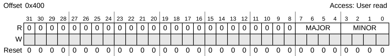
Figure 31-4. Revision (G12_REVISION)
