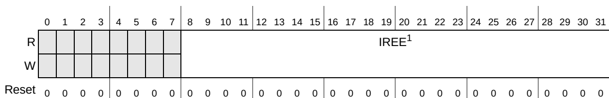
Figure 43-7. Interrupt Rising-Edge Event Enable Register (IREER)
