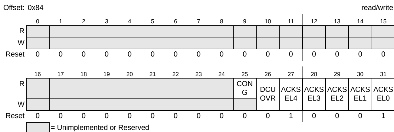
Figure 14-4. prioman_config2 register (CFG2)
