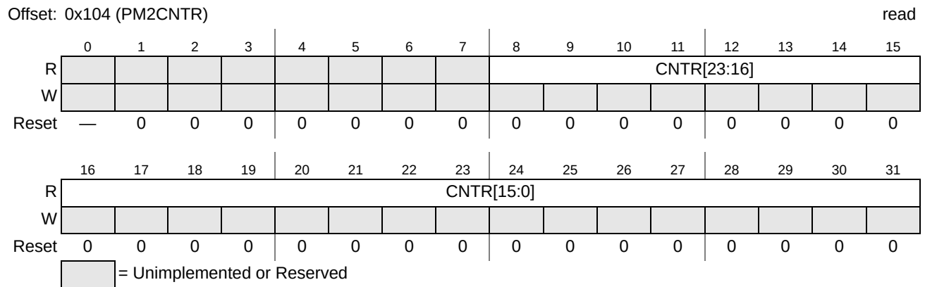
Figure 14-15. Performance Monitor 2 Read Counter (PM2CNTR)
