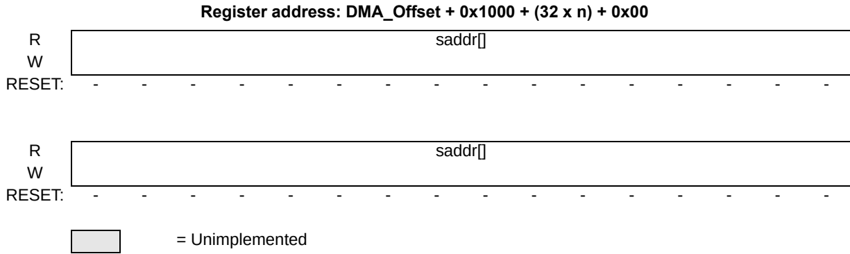
Figure 17. TCDn Word 0 (TCDn.saddr) field
