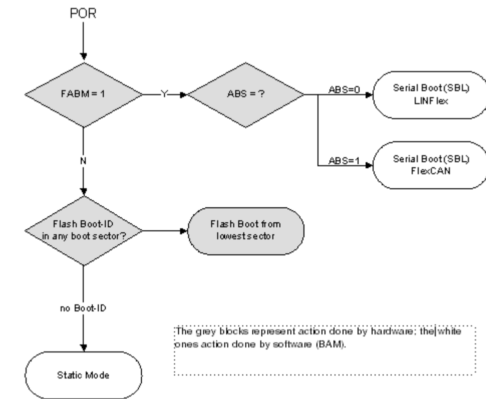
Figure 6-1. Boot mode selection
