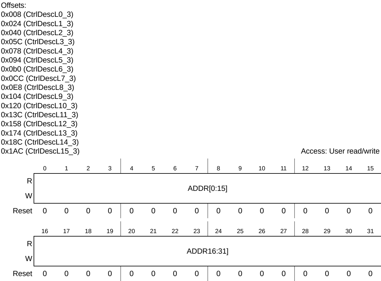
Figure 11-6. CtrlDescL0_3 Register
