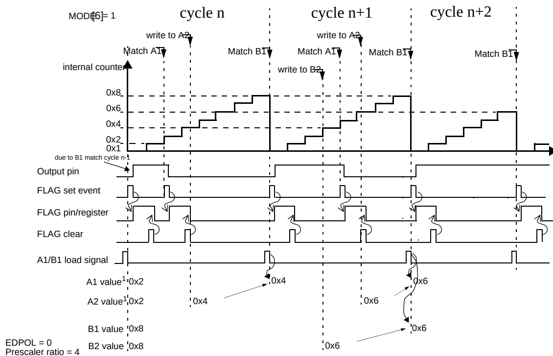
Figure 17-27. OPWFMB A1 and B1 Registers Update and Flags
