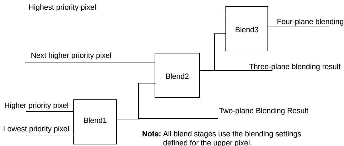
Figure 11-64. Pixel blending stack
