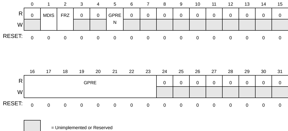
Figure 17-4. eMIOS200 Module Configuration Register (MCR)
