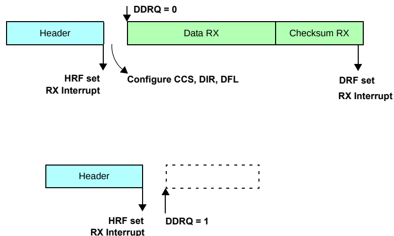
Figure 27-62. Programming consideration: slave node, receiver, no filters
