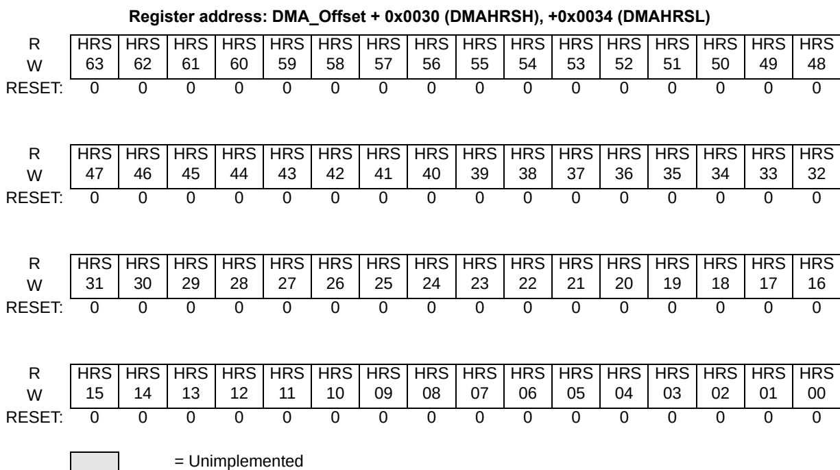
Figure 14. eDMA Hardware Request Status (DMAHRSH, DMAHRS�) Registers
