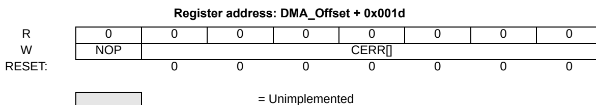
Figure 9. eDMA Clear Error (DMACERR) Register
