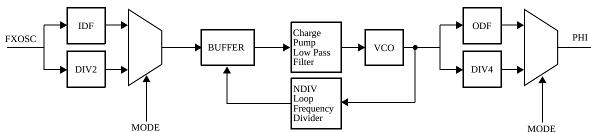
Figure 8-29. FMPLL block diagram
