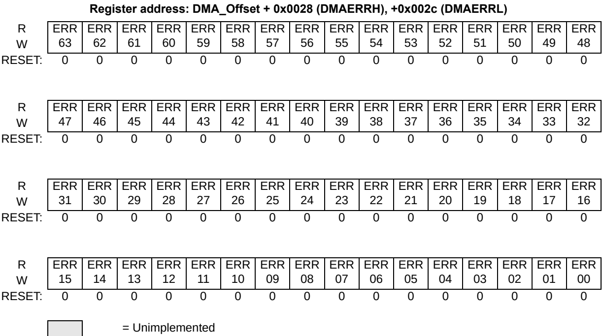
Figure 13. eDMA Error (DMAERRH, DMAERRL) Registers
