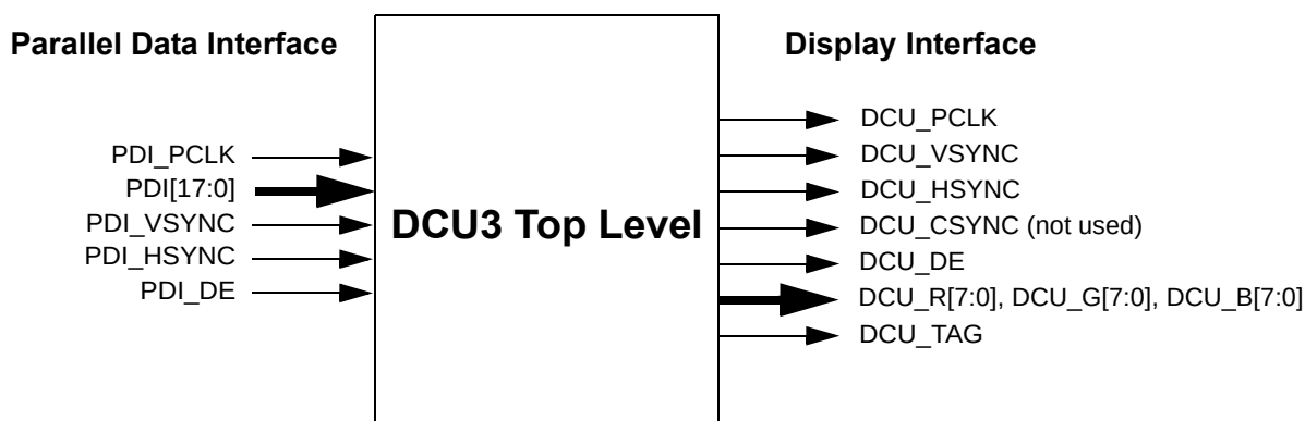
Figure 11-2. External signals
