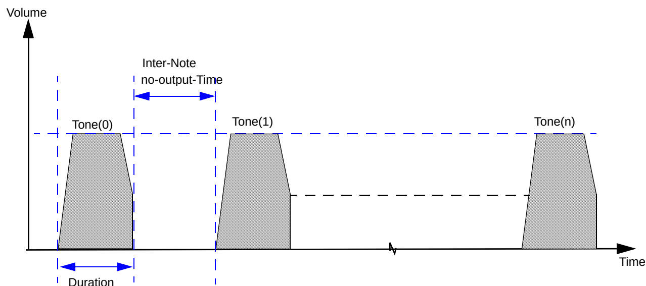
Figure 39-42. DDS Mode for one Channel
