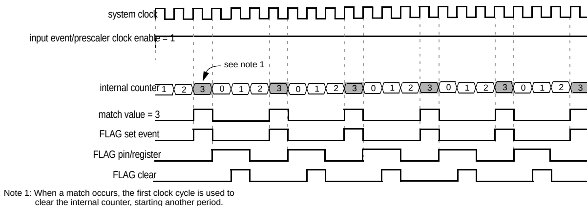
Figure 17-38. Time base period when running in the fastest prescaler ratio
