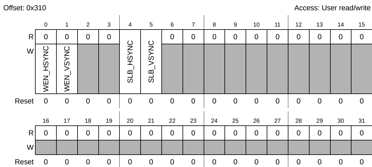
Figure 11-59. Soft Lock HSYNC/VSYNC PARA Register
