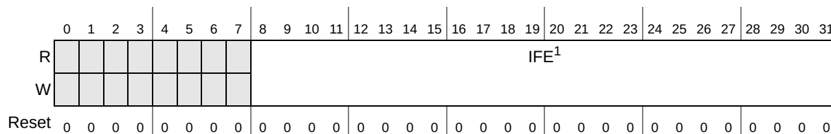
Figure 43-9. Interrupt Filter Enable Register (IFER)
