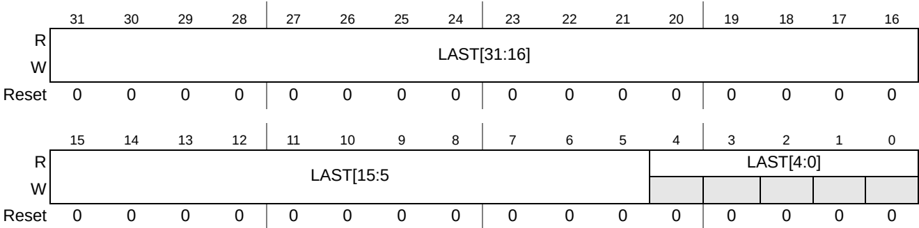
Figure 22-5. Window Last Address (GXGLAST0-3)
