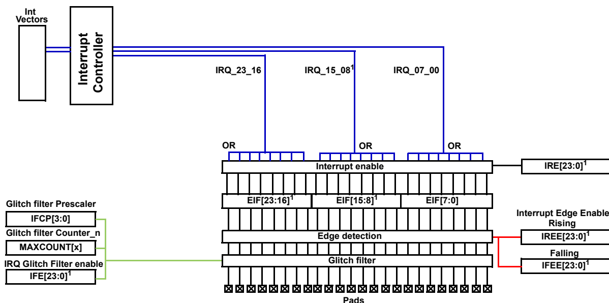
Figure 43-22. External interrupt pad diagram
