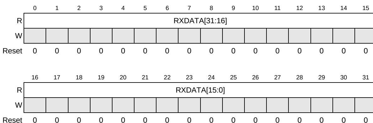
Figure 35-16. RX Buffer Data Registers 0–31 (QSPI_RBDR0–QSPI_RBDR31)
