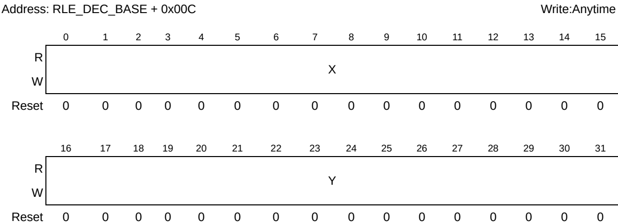
Figure 38-5. Decompressed Image Coordinates Register (RLE_DEC_DICR)
