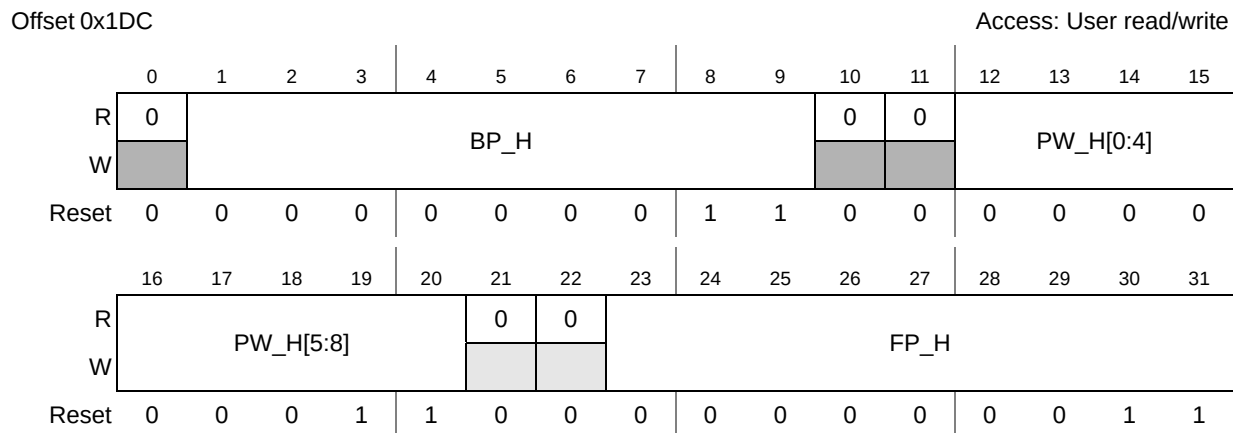
Figure 12-18. HSYN_PARA Register
