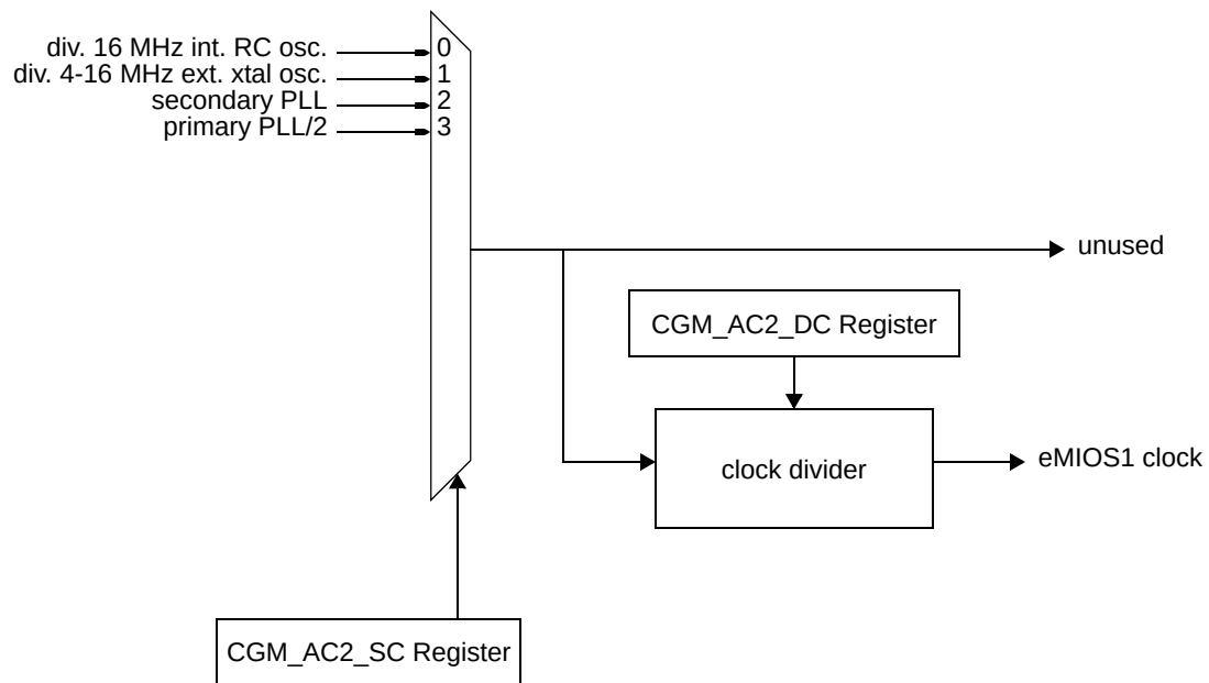
Figure 8-21. MC_CGM Auxiliary Clock 2 Generation Overview
