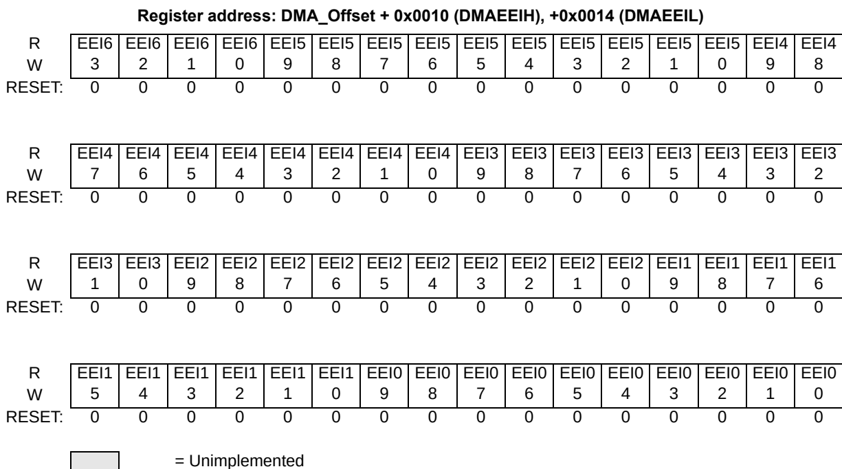
Figure 3. eDMA Enable Error Interrupt (DMAEEIH, DMAEEIL) Registers
