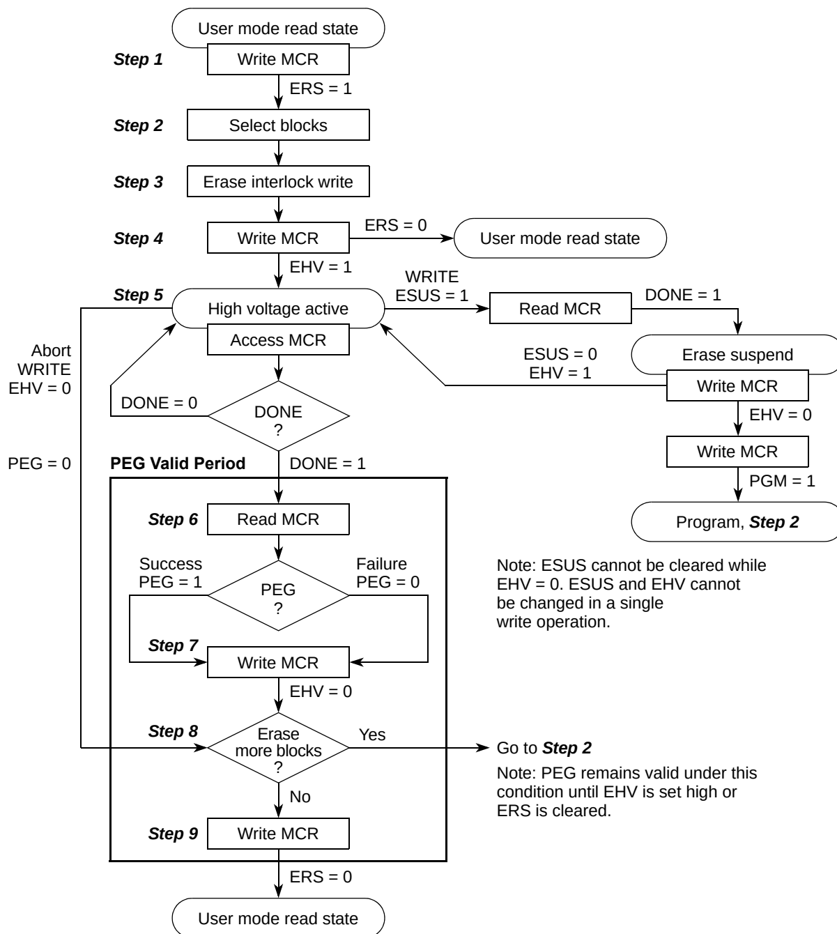
Figure 21-28. Erase Sequence
