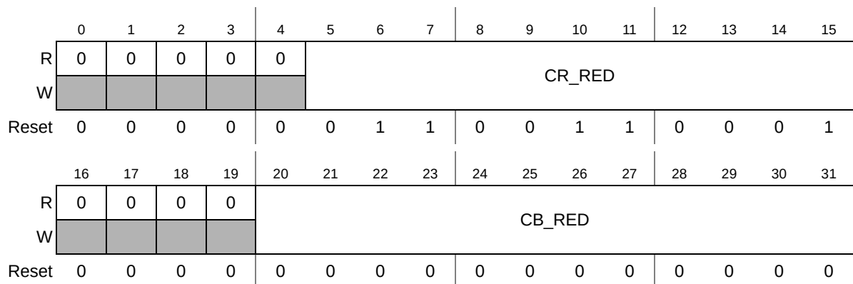
Figure 12-50. Layer RED Chroma Component Register (LYR_CHROMA_RED)
