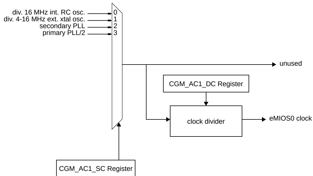
Figure 8-20. MC_CGM Auxiliary Clock 1 Generation Overview
