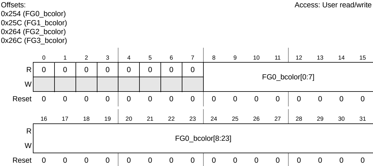
Figure 12-47. FG0_bcolor Register
