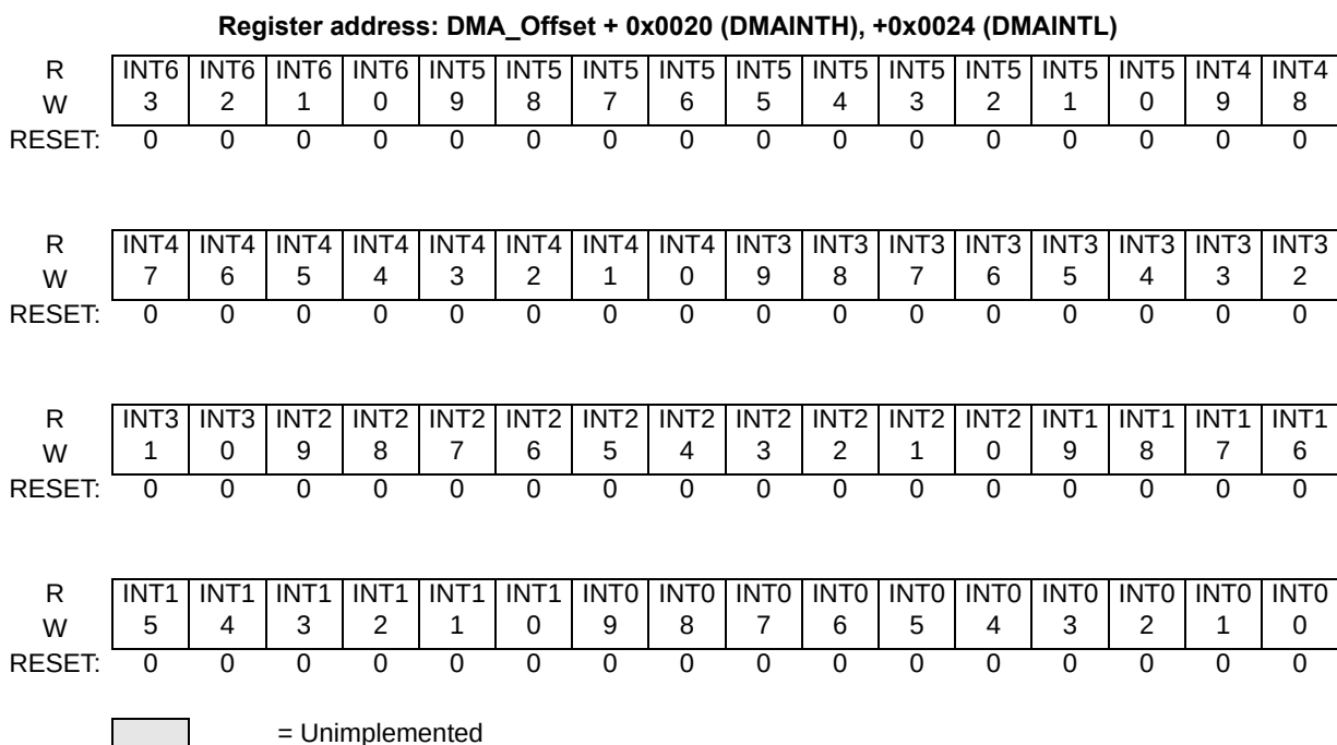
Figure 12. eDMA Interrupt Request (DMAINTH, DMAINTL) Registers
