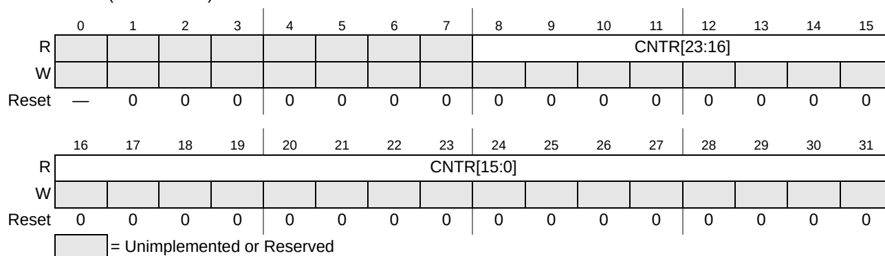
Figure 14-32. Summed Priority Counter 4 (SPRIOCTR4)
