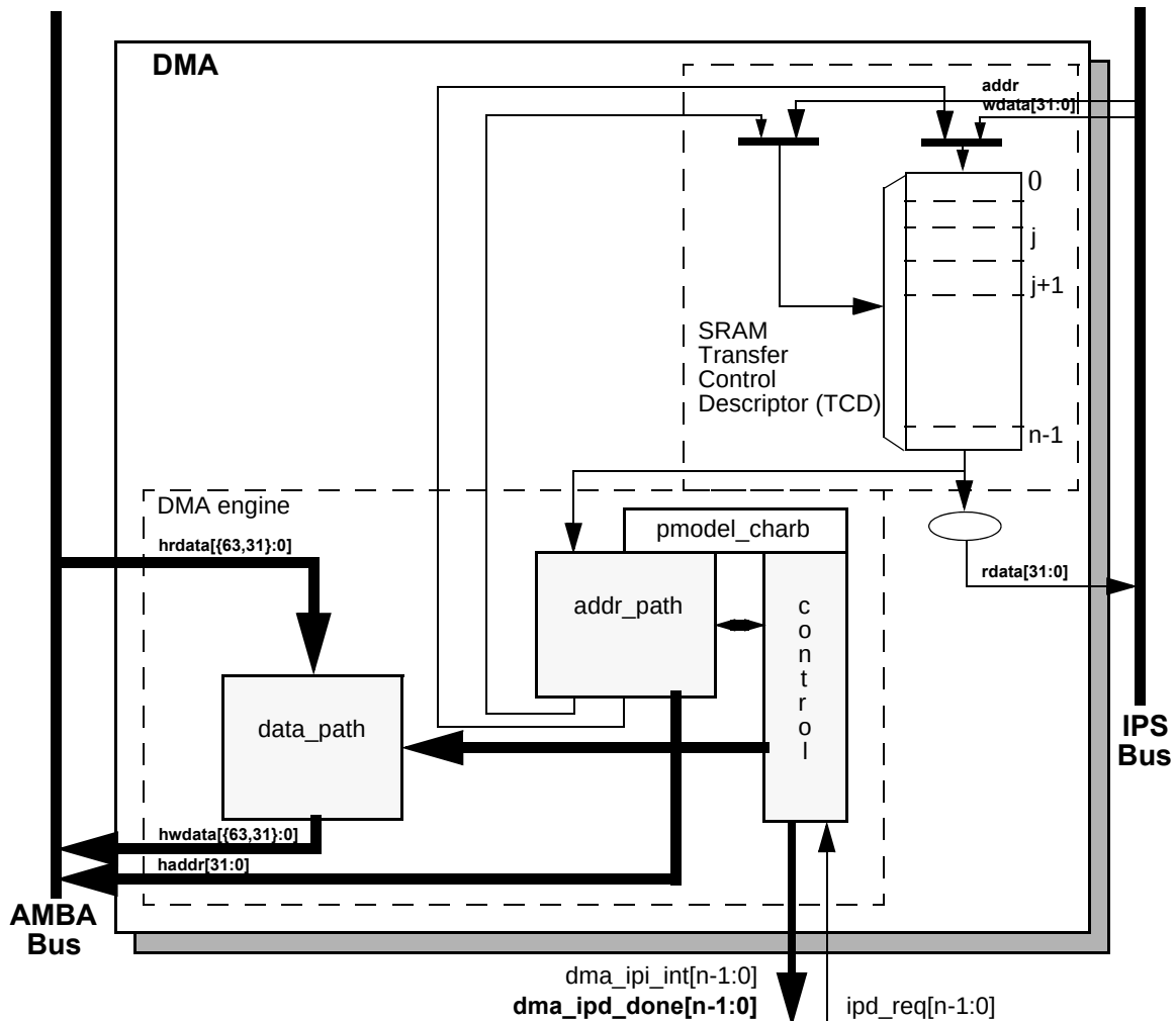
Figure 18-29. eDMA operation, part 2
