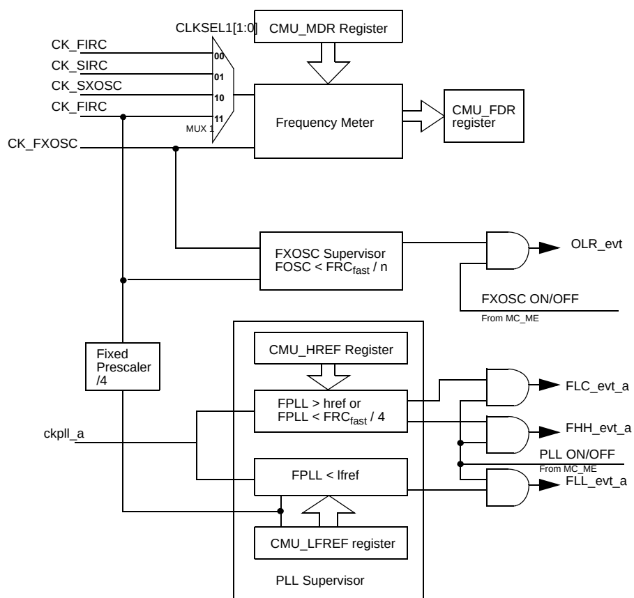
Figure 8-33. Clock Monitor Unit diagram
