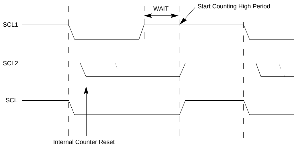
Figure 25-13. I²C Bus Clock Synchronization
