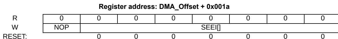
Figure 6. eDMA Set Enable Error Interrupt (DMASEEI) Register
