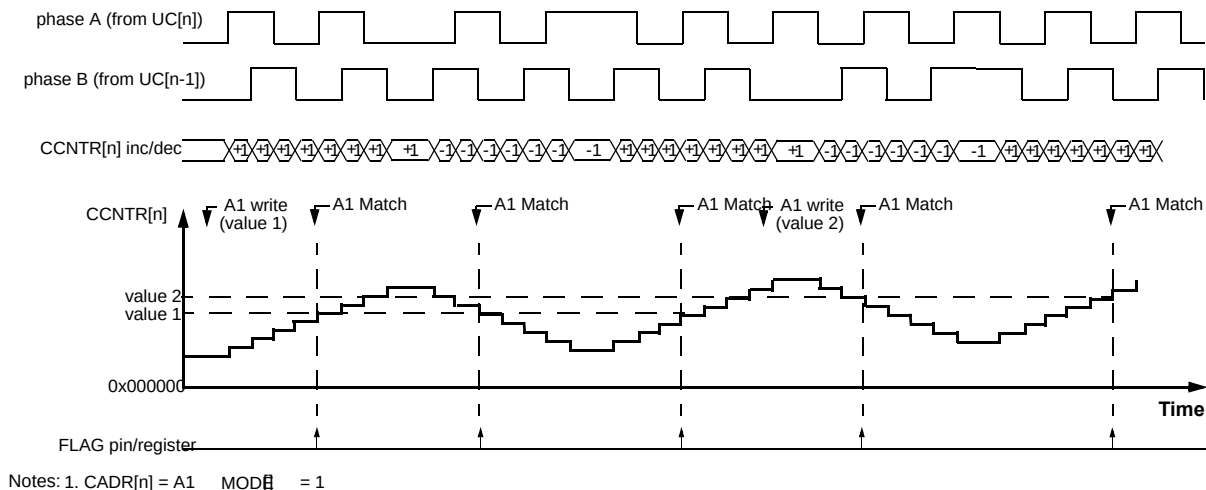
Figure 17-35. Quadrature Decode mode example with phase_a & phase_B encoder
