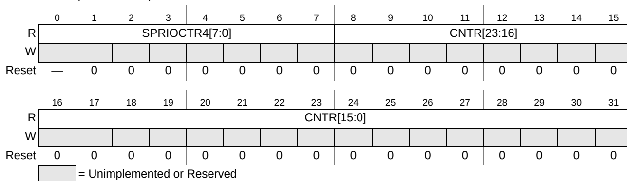
Figure 14-24. Cumulative Wait Counter 1 (CUMWCTR1)
