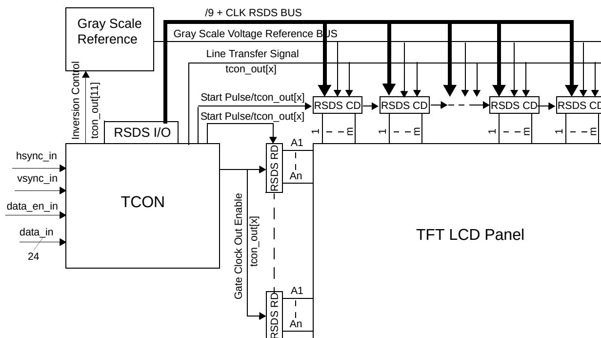
Figure 46-1. Application diagram of the TCON
