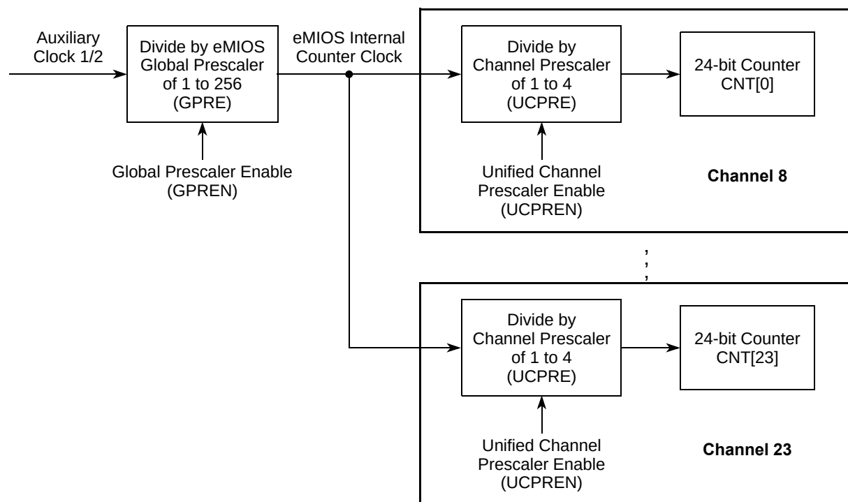
Figure 17-14. eMIOS prescalers
