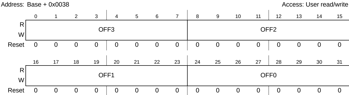
Figure 13-13. DQS Config Offset Count Register (DRAMC_DQS_OC)
