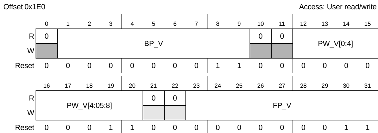
Figure 12-19. VSYN_PARA Register
