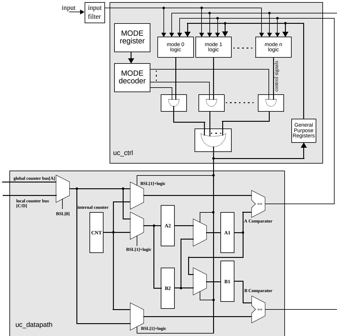
Figure 17-16. Unified Channel Control and Datapath Block Diagrams
