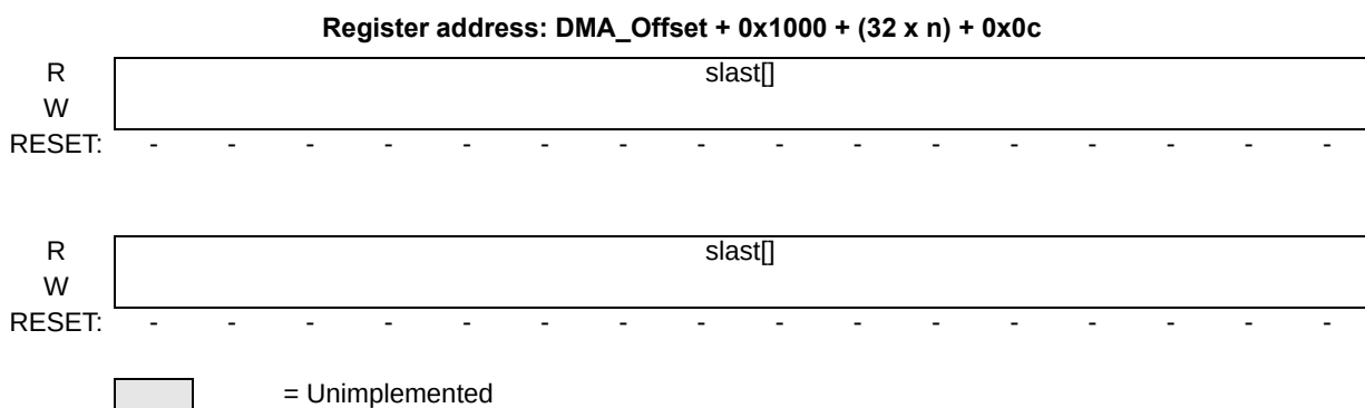
Figure 21. TCDn Word 3 (TCDn.slast) field
