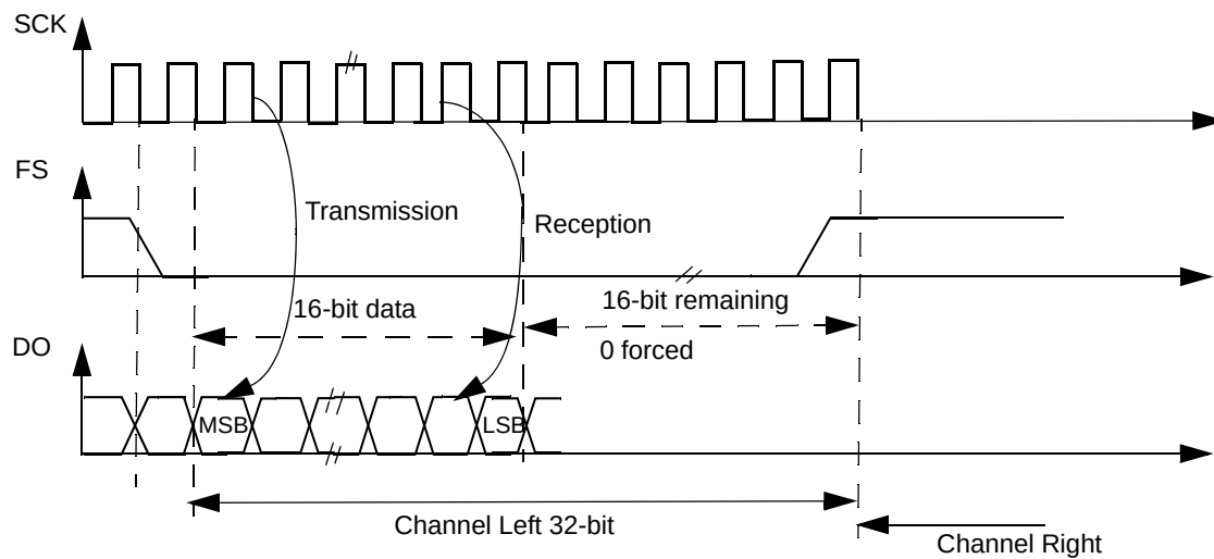
Figure 39-50. Philips Mode 16-bit extended to 32-bit
