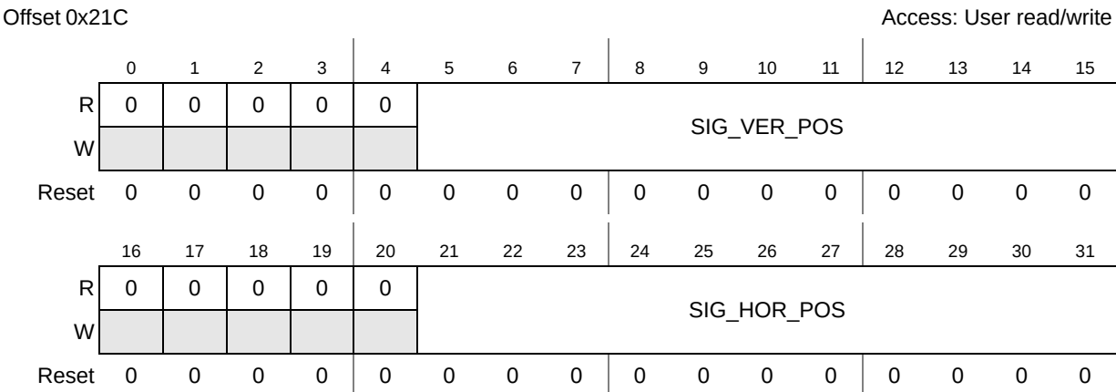
Figure 12-34. SIGN_CALC_2 register
