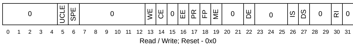
Figure 50-5. Machine State Register (MSR)
