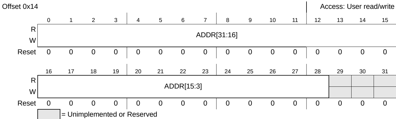
Figure 47-7. DMA_ADDR Register
