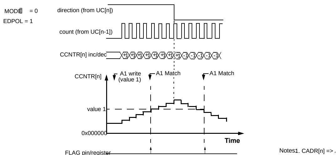
Figure 17-34. Quadrature Decode mode example with count & direction encoder
