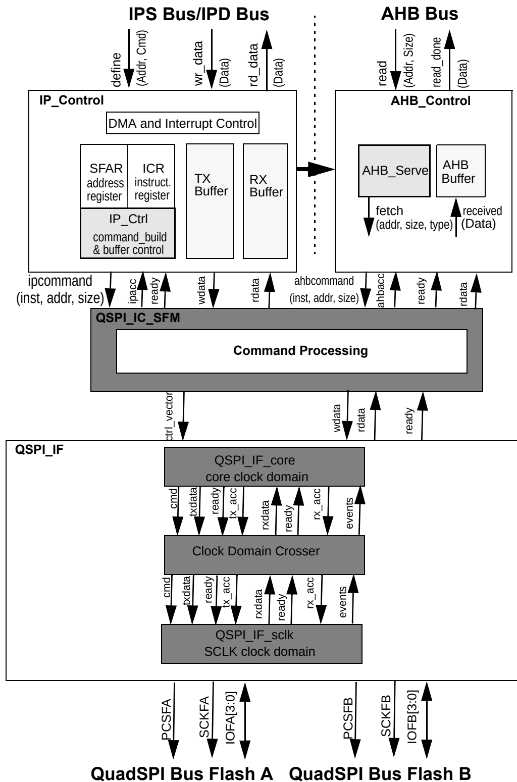
Figure 35-1. QuadSPI block diagram
