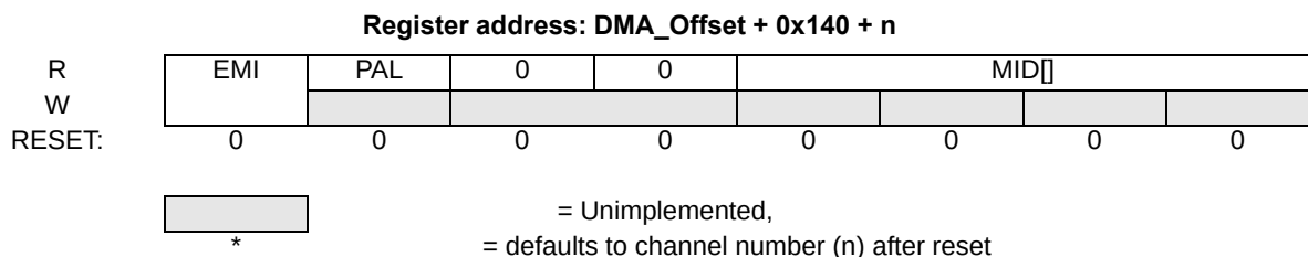
Figure 16. eDMA Channel n Master ID (DCHMIDn) Register
