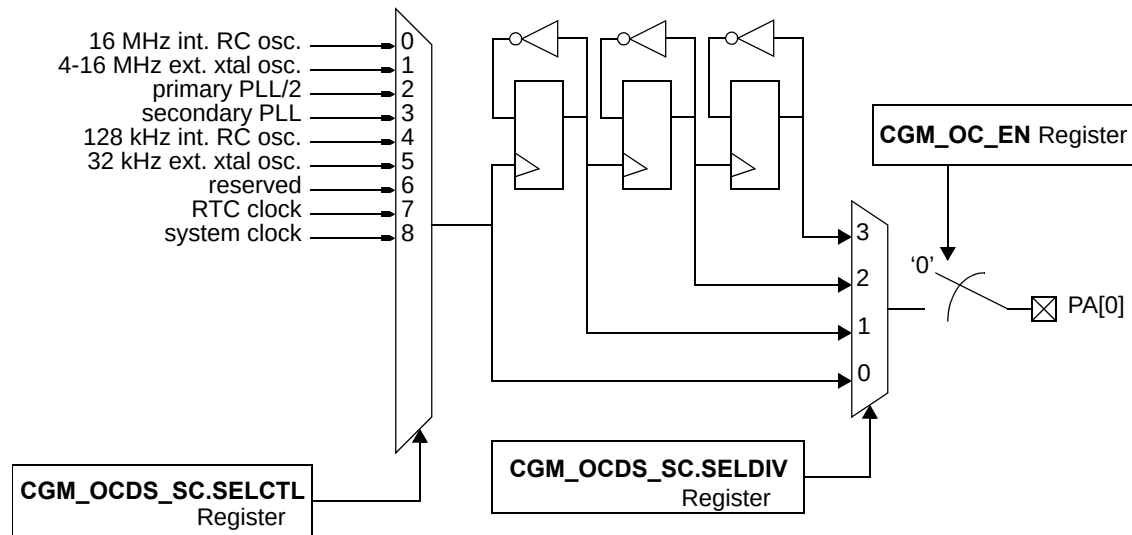
Figure 8-24. MC_CGM Output Clock Multiplexer and PA[0] Generation
