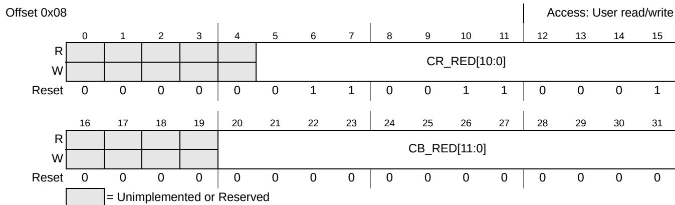
Figure 47-4. CHROMA_RED Register
