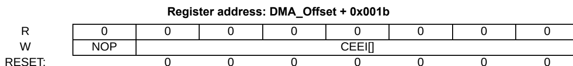
Figure 7. eDMA Clear Enable Error Interrupt (DMACEEI) Register
