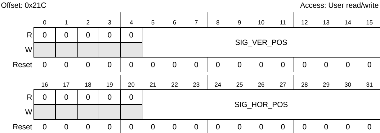
Figure 11-34. SIGN_CALC_2 Register
