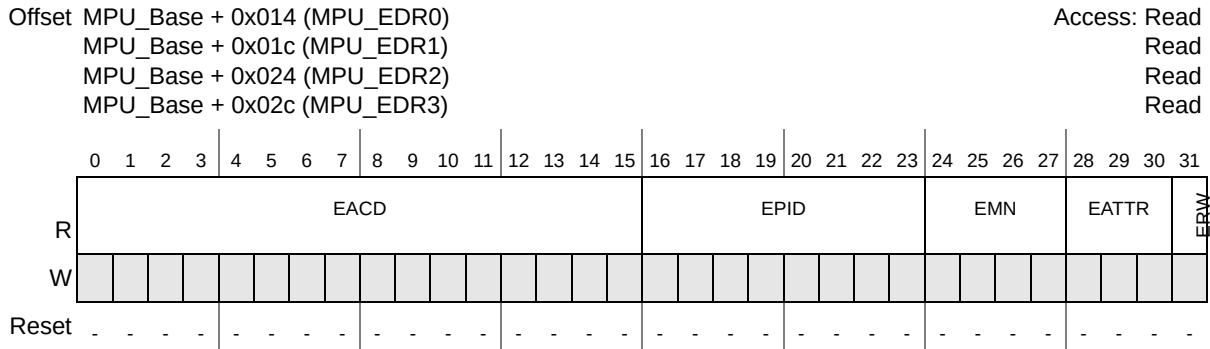
Figure 28-4. MPU Error Detail Register, Slave Port n (MPU_EDRn)
