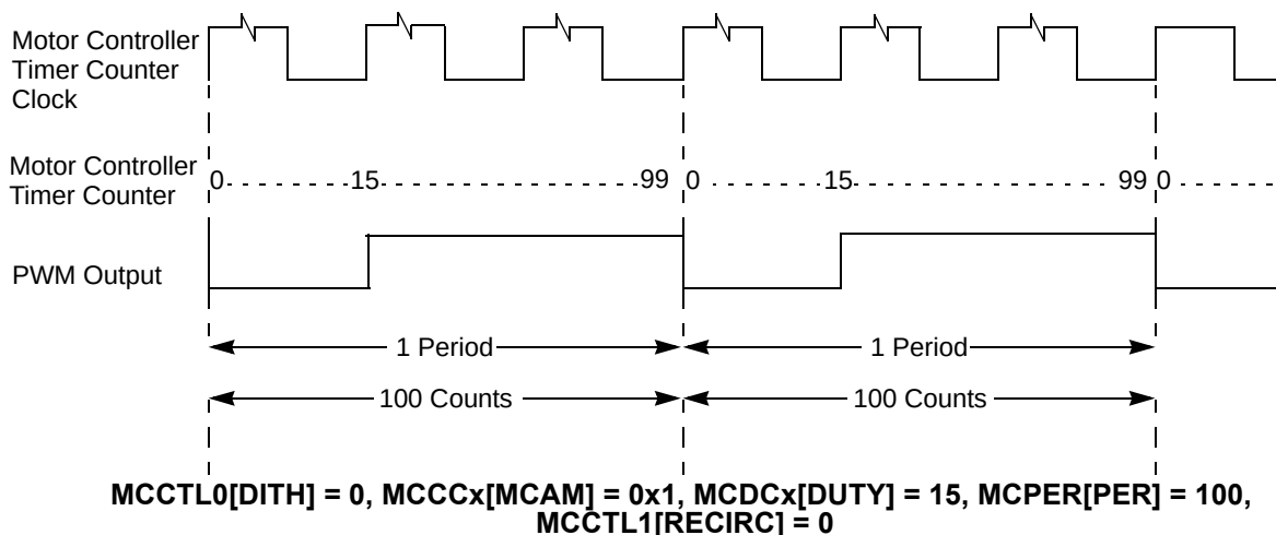
Figure 41-19. Left Aligned
