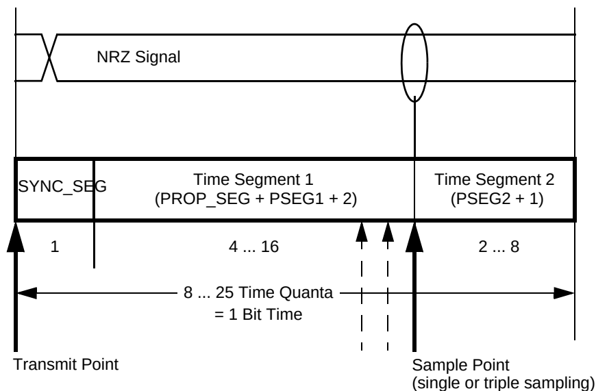
Figure 20-17. Segments within the Bit Time
