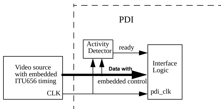
Figure 12-91. PDI Input data mode
