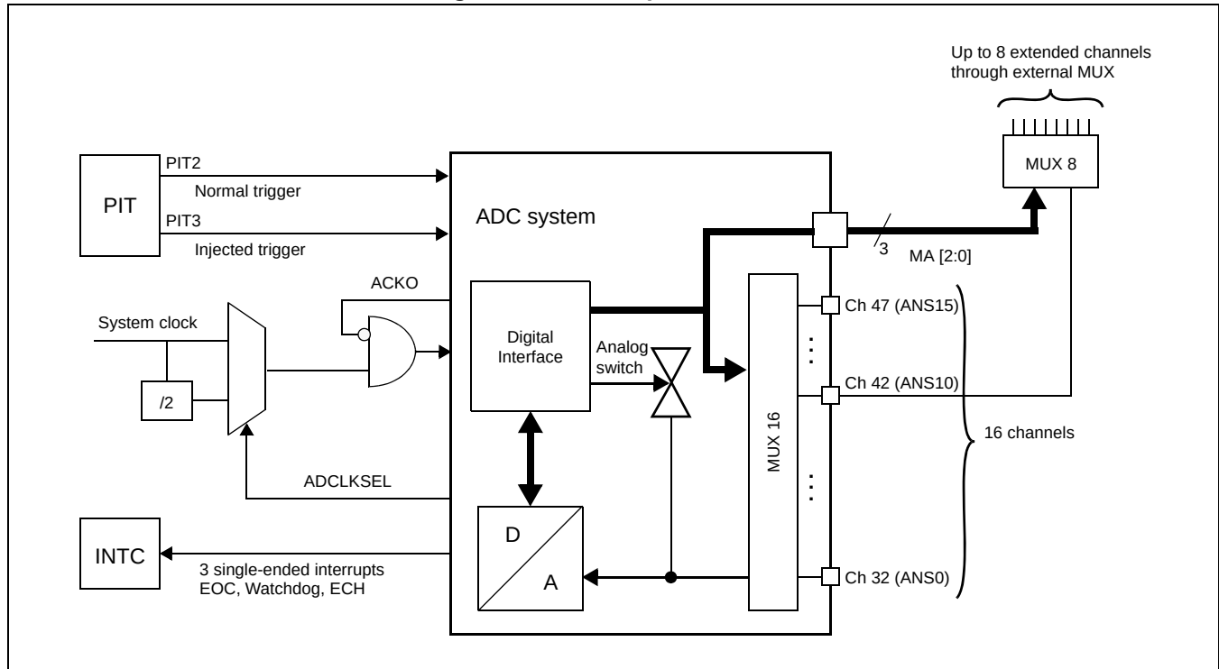
Figure 5-1. ADC implementation
