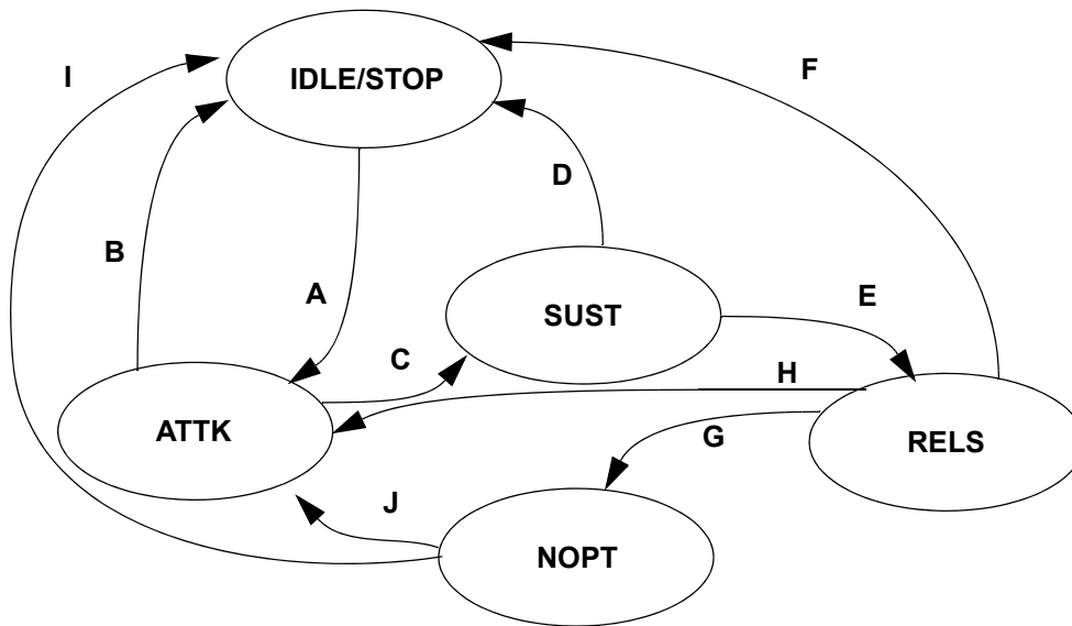
Figure 39-44. DDS-Mode State Machine - by Function
