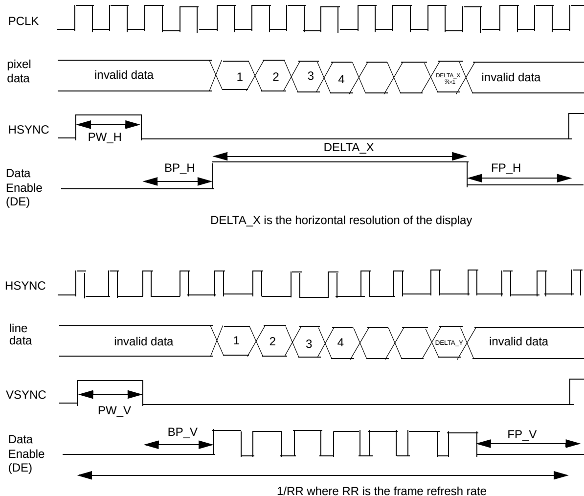
Figure 11-63. HSYNC and VSYNC timing diagram
