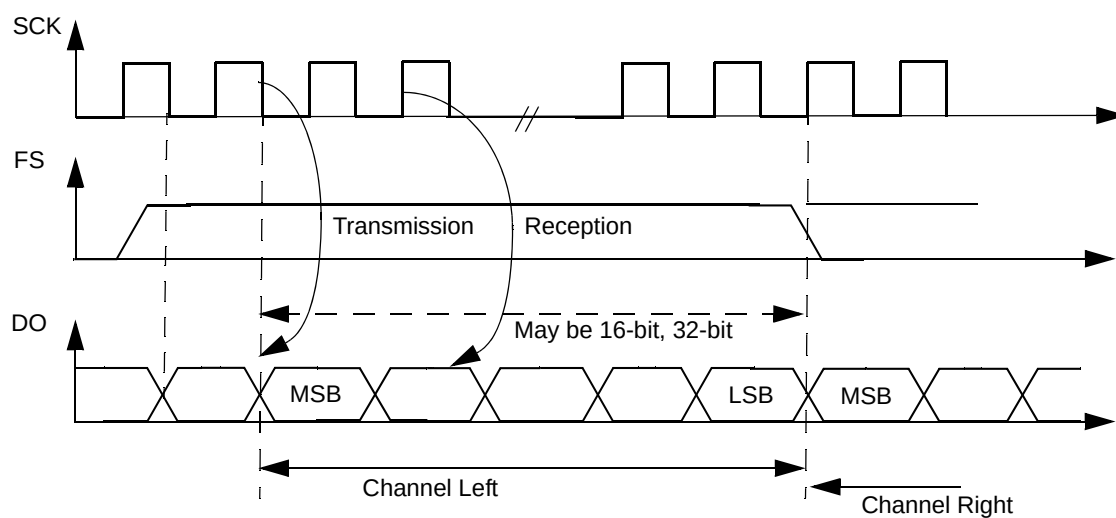
Figure 39-54. 16/32bit
