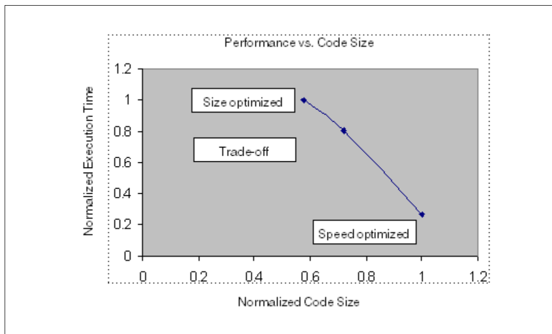
Figure 50-4. Influence of compiler settings on application performance and code size
