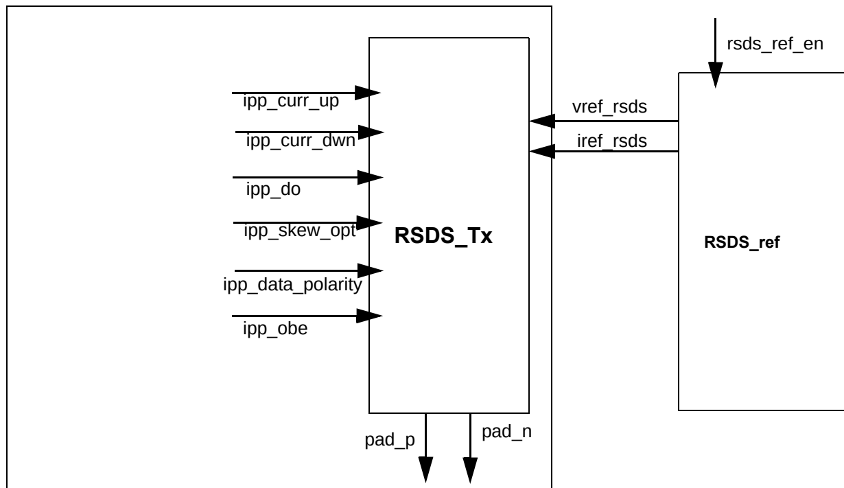
Figure 46-15. RSDS interface
