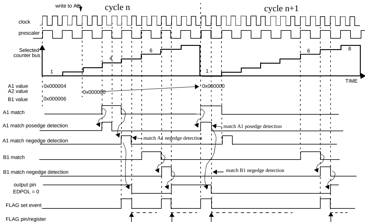
Figure 17-30. OPWMB Mode Matches and Flags
