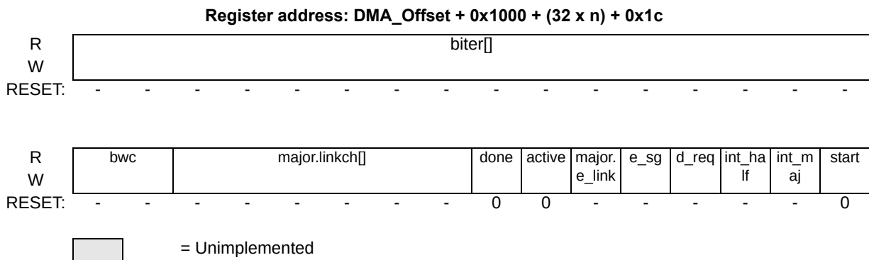
Figure 25. TCDn Word 7 (TCDn.{biter,control/status}) fields
