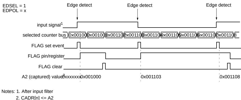
Figure 17-18. Single Action Input Capture with both edges triggering example
