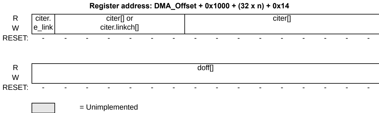
Figure 23. TCDn Word 5 (TCDn.{citer,doff}) fields
