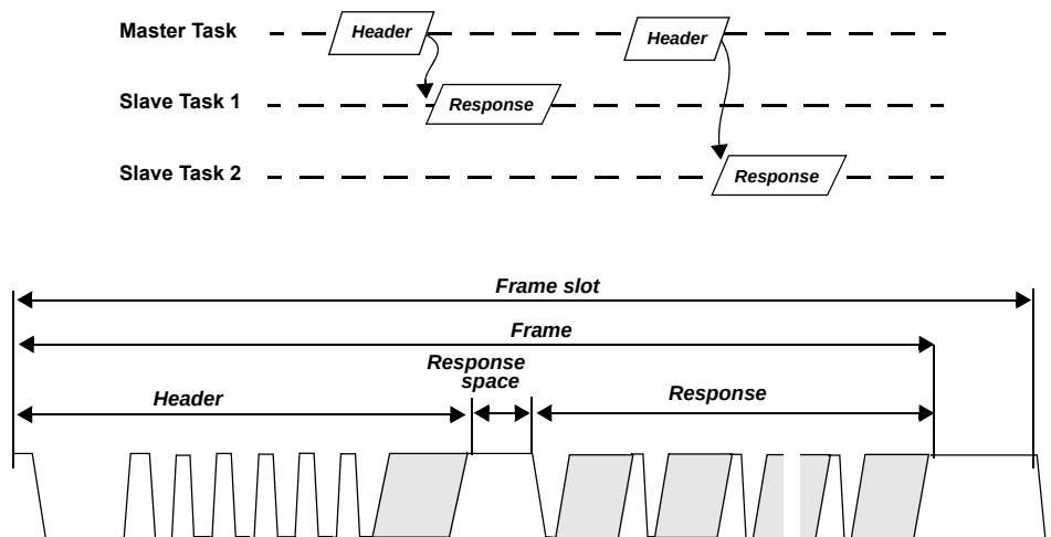
Figure 27-3. LIN frame structure
