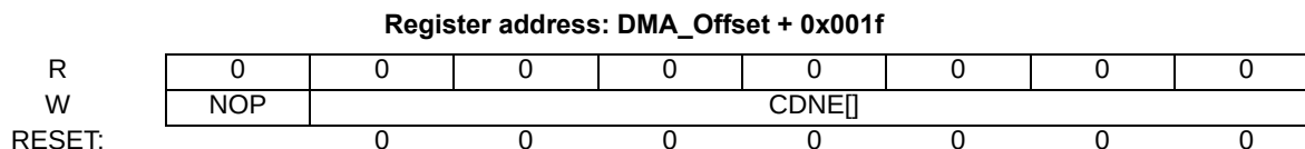
Figure 11. eDMA Clear DONE Status (DMACDNE) Register
