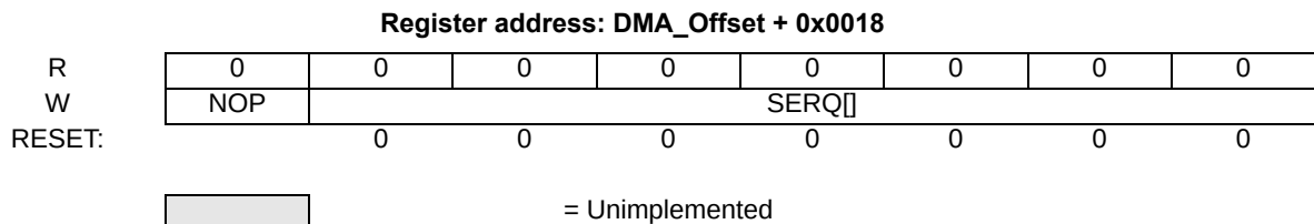
Figure 4. eDMA Set Enable Request (DMASERQ) Register
