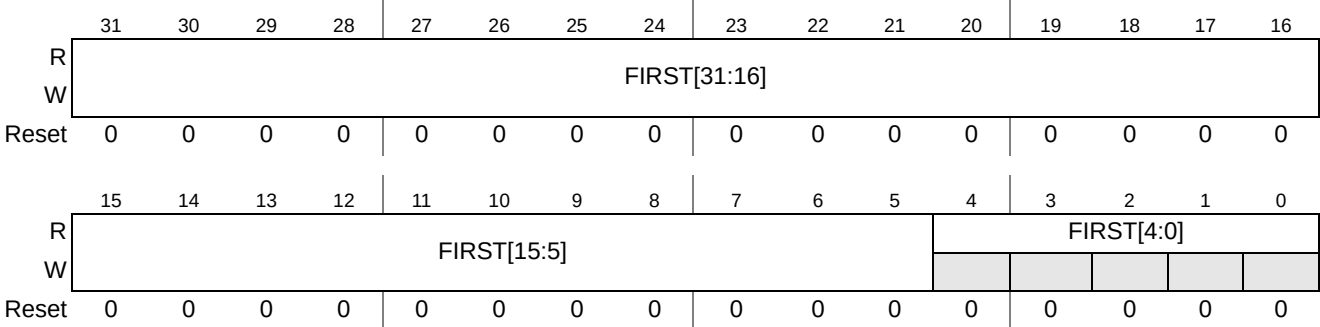
Figure 22-4. Window First Address (GXGFRST0-3)
