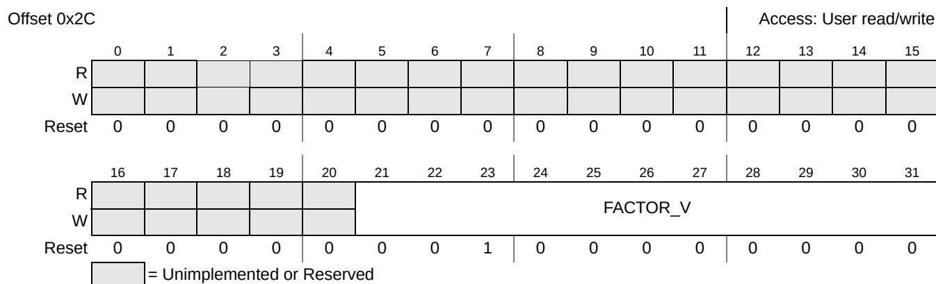
Figure 47-13. VFACTOR Register
