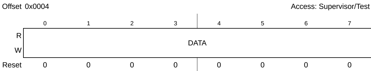
Figure 25-9. I 2 C Bus Data I/O Register (IBDR)
