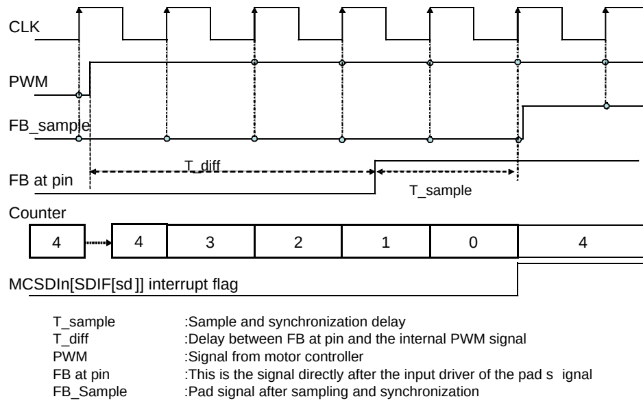
Figure 41-34. Example for \text{MCSDTO}[\text{TOUT}] = 4
