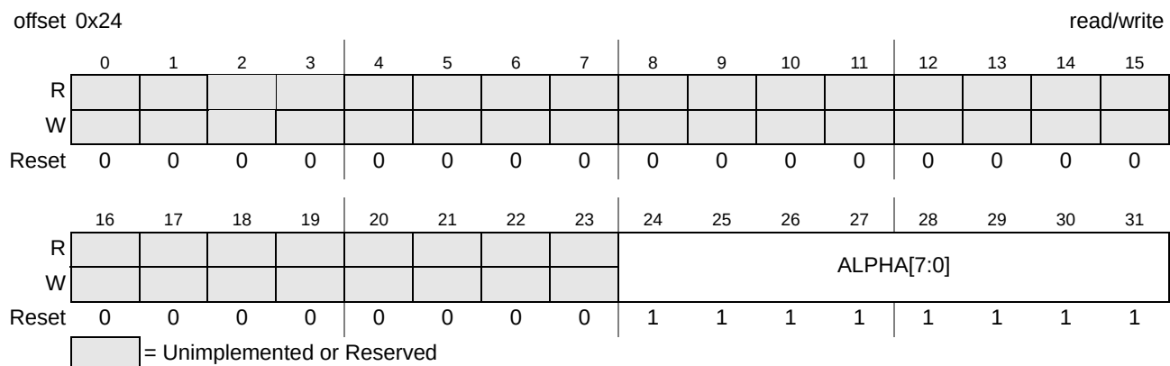
Figure 47-11. ALPHA Register
