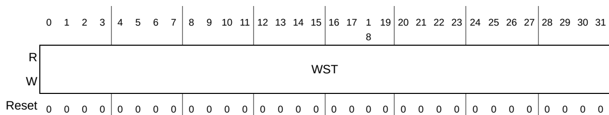
Figure 4-16. SWT Window Register (SWT_WN)
