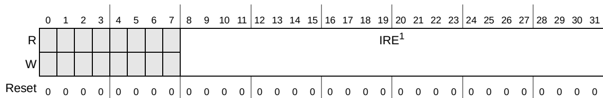
Figure 43-6. Interrupt Request Enable Register (IRER)
