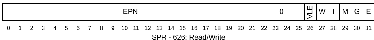
Figure 50-3. MMU Assist Register 2 (MAS2)
