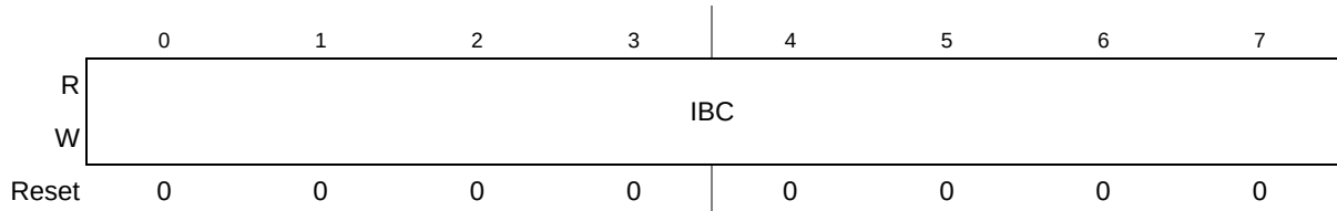
Figure 25-4. I 2 C Bus Frequency Divider Register (IBFD)
