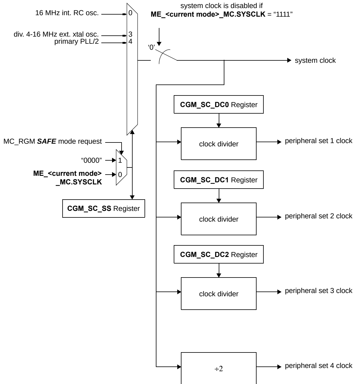
Figure 8-18. MC_CGM system clock generation overview
