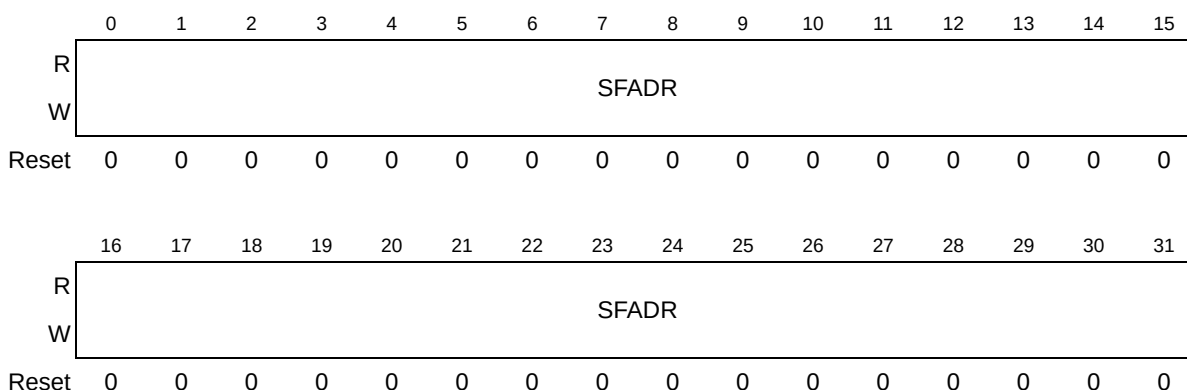
Figure 35-5. Serial Flash Address Register (QSPI_SFAR)
