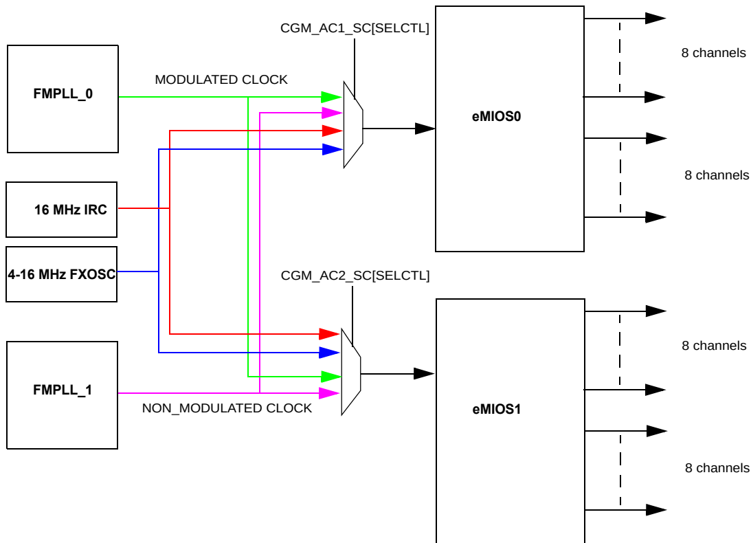
Figure 17-2. eMIOS clocking configuration
