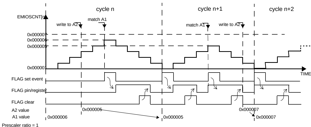
Figure 17-22. Modulus Counter Buffered (MCB) Up/Down Mode
