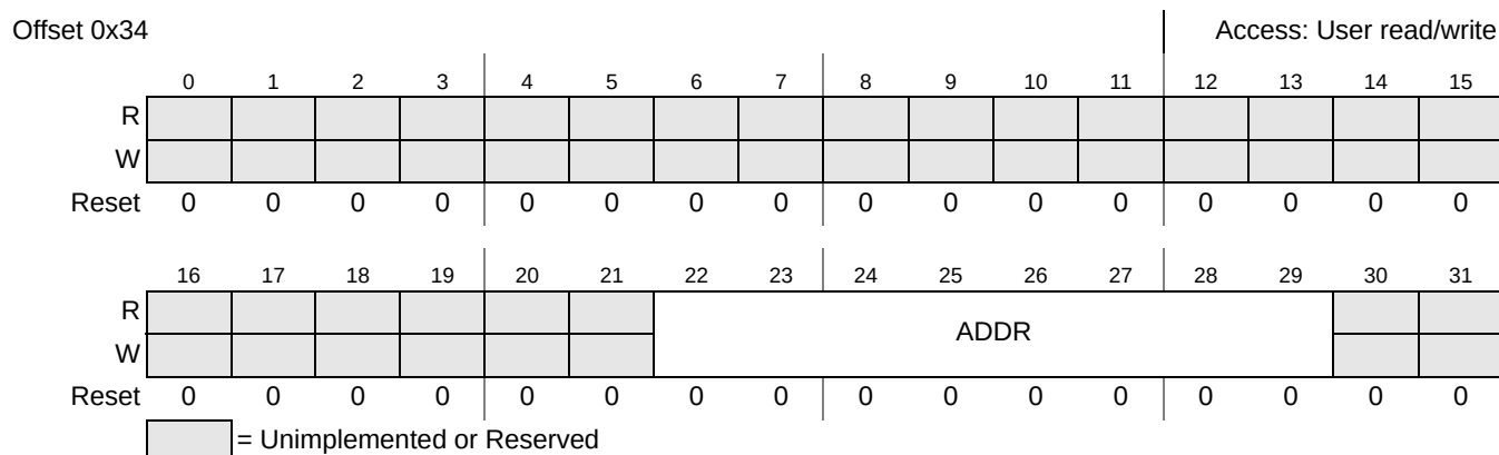
Figure 47-15. LUT_ADDR Register
