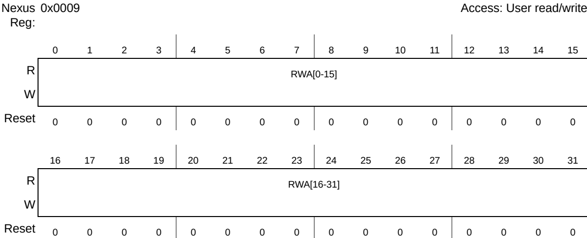
Figure 30-9. Read/Write Access Address Register (RWA)
