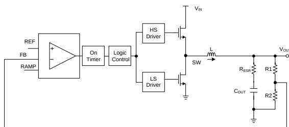
Figure 3: Simplified Compensation Block
