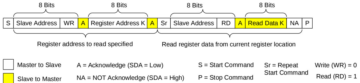
Figure 12: I²C Read Example (Read Register)
