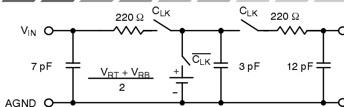
Figure 2. Input Equivalent Circuit
