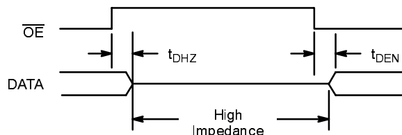
Figure 4. Output Enable/Disable Timing Diagram
