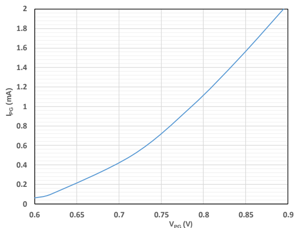
Figure 8: PGGOOD Clamped Voltage vs. Pull-Up Current
