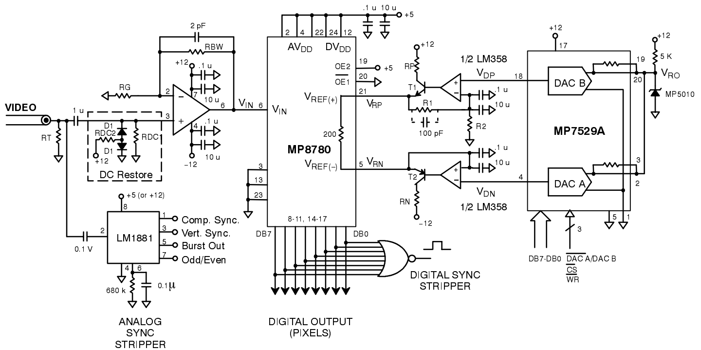
Figure 21. Video Digitizer
