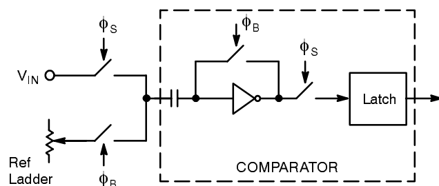
Figure 6. MP8780 Comparator
