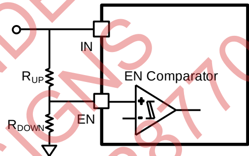
Figure 9: Adjustable UVLO
