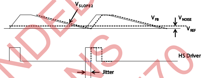
Figure 5: Skip-Mode Jitter
