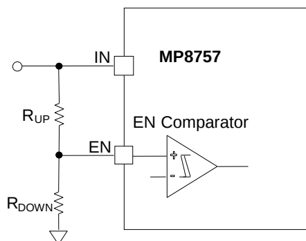
Figure 9—Adjustable UVLO
