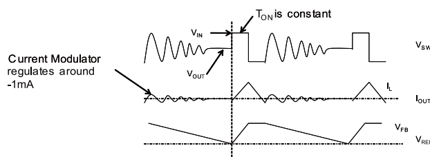
Figure 3: DCM Operation
