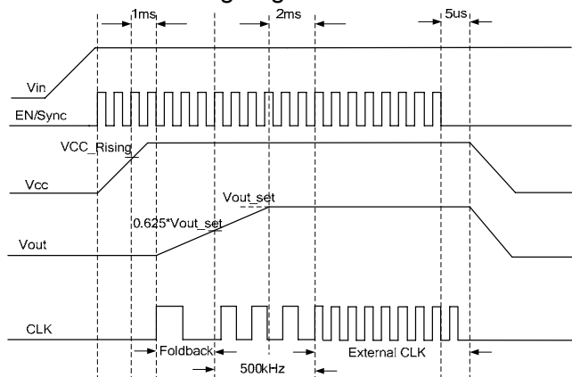
Figure 4—Startup Sequence Using External Sync Clock Signal
