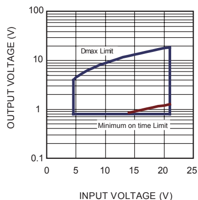
Operating Range
