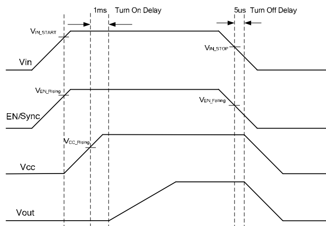
Figure 3—Startup Sequence Using EN Divider
