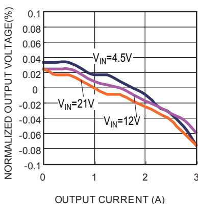
Load Regulation
