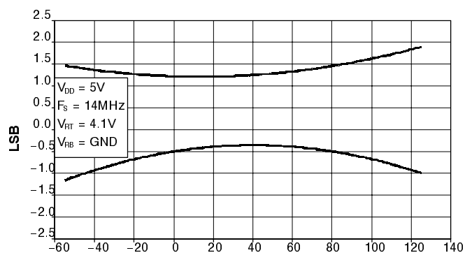
Figure 9. INL vs TEMPERATURE
