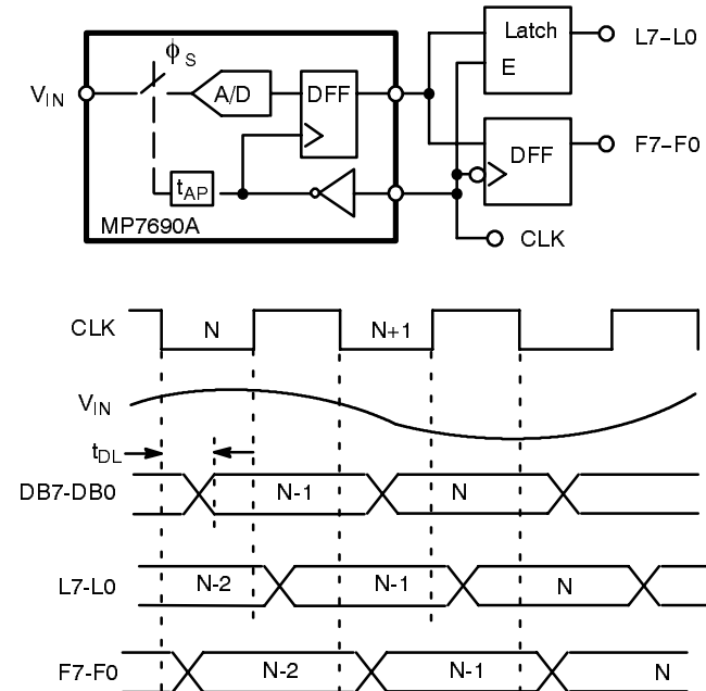
Figure 14. MP7690A Functional Equivalent Circuit and Interface Timing
