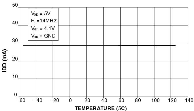
Figure 7. I_{DD} vs TEMPERATURE
