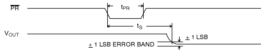
Figure 4. PRESET Timing
