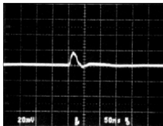
Graph 22. Digital Feedthrough
