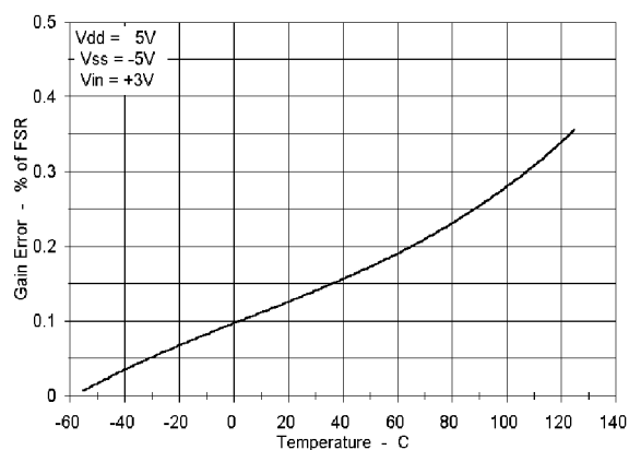
Graph 10. Gain Error vs. Temperature
