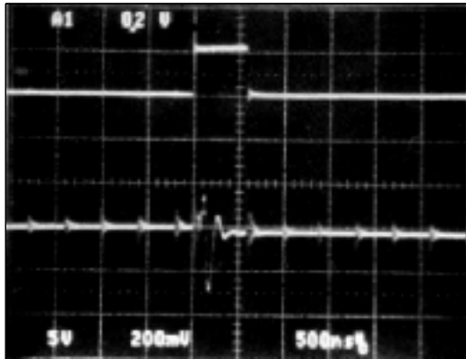
Graph 15. 1 LSB Digital Step Change
