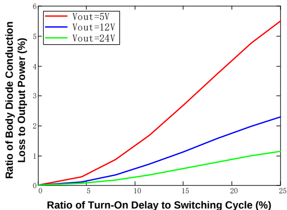
Figure 12: Turn-On Delay vs. Power Loss
