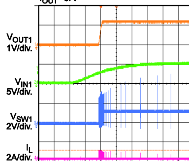
VIN Power Up without
