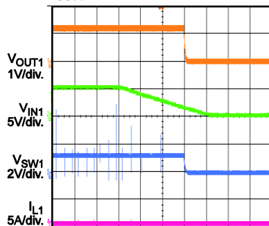
VIN Power Down without
