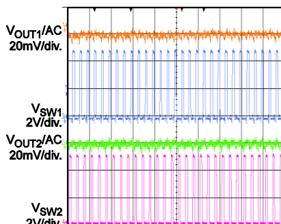
Output Ripple
