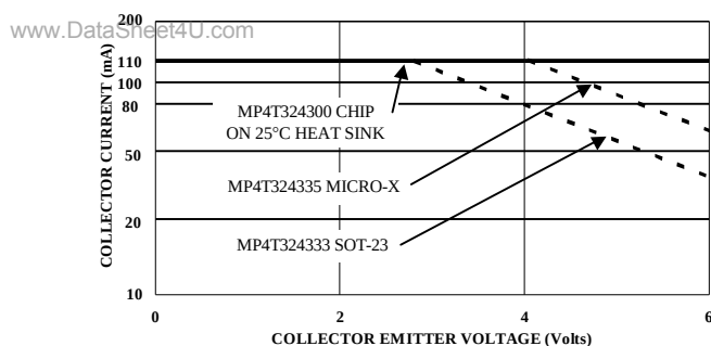
DC SAFE OPERATING RANGE at 25 °C
