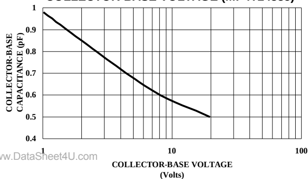
NOMINAL COLLECTOR-BASE CAPACITANCE vs COLLECTOR-BASE VOLTAGE (MP4T24335)
