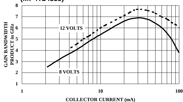
NOMINAL GAIN BANDWIDTH PRODUCT ( f_T ) vs COLLECTOR CURRENT at V_{CE} = 8 and 12 VOLTS (MP4T24335)
