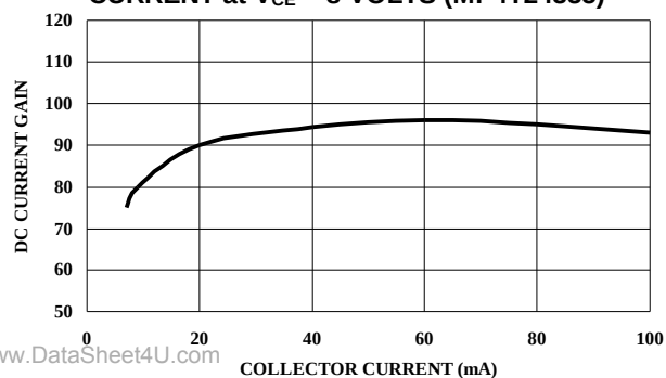
NOMINAL DC CURRENT GAIN ( h_{FE} ) vs COLLECTOR CURRENT at V_{CE} = 8 VOLTS (MP4T24335)
