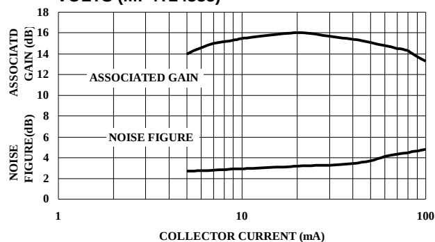
NOMINAL NOISE FIGURE and ASSOCIATED GAIN vs COLLECTOR CURRENT at 1 GHz and V_{CE} = 12 VOLTS (MP4T24335)
