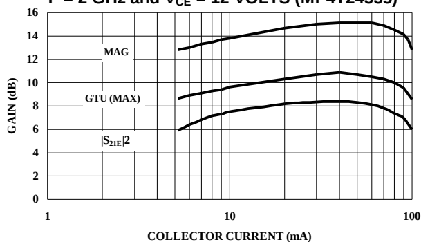
NOMINAL GAIN vs COLLECTOR CURRENT at F = 2 GHz and V_{CE} = 12 VOLTS (MP4T24335)
