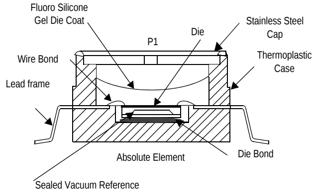
Figure 2. Cross Sectional Diagram SSOP (not to scale)
