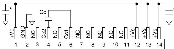
COMPONENT SIDE VIEW
