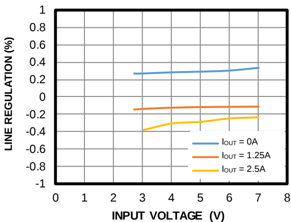
Line Regulation
