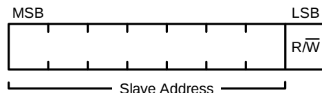
Figure 8: 7-Bit Addressing
