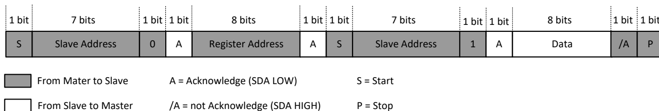
Figure 17: I²C Single Read
