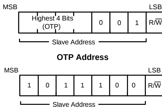
Figure 14: 7-Bit Address
