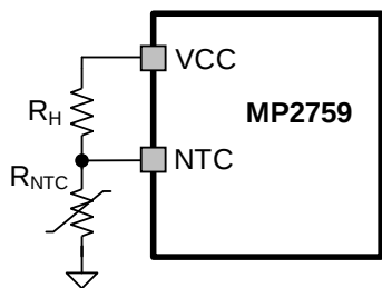
Figure 6: Thermistor Connection
