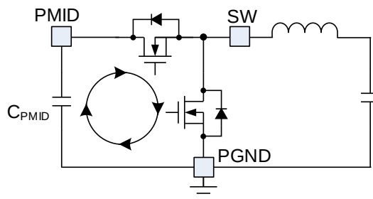
Figure 7: High-Frequency Current Path
